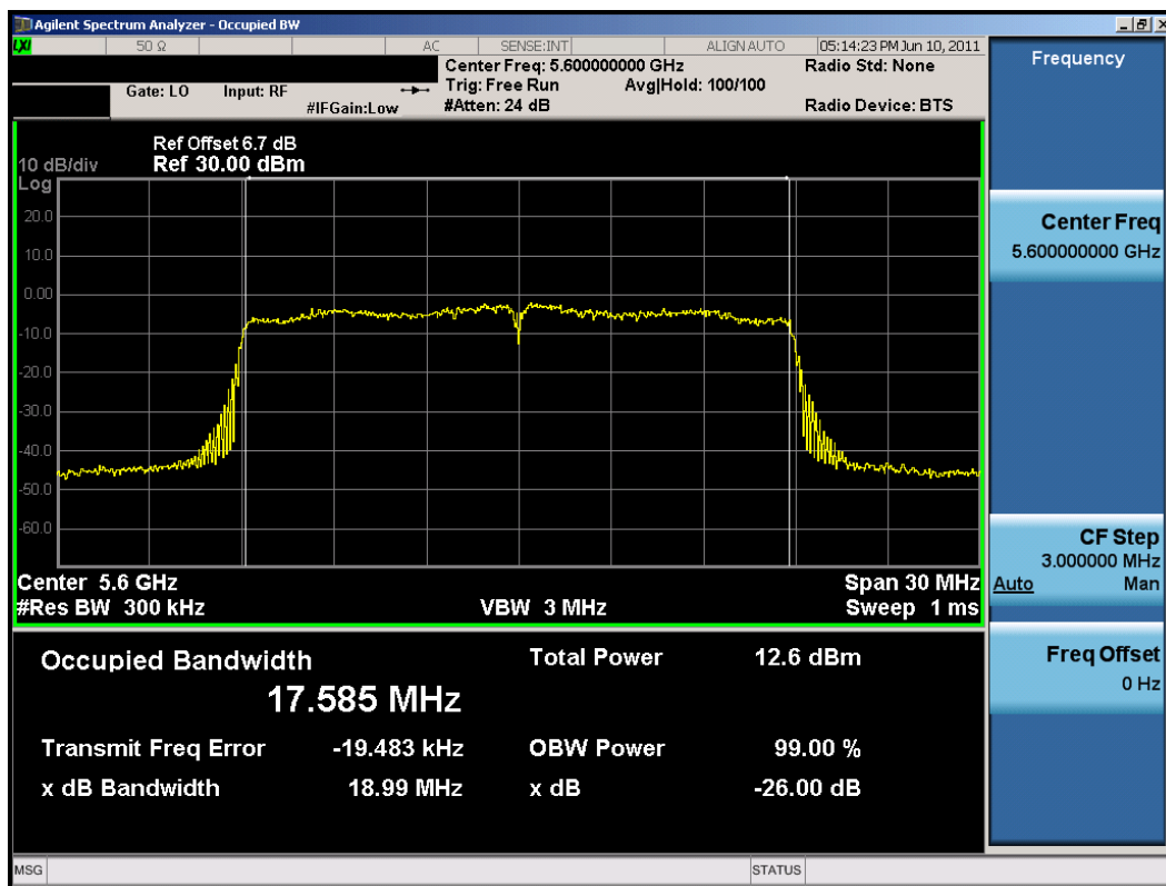
Plot 6-17. 26dB Bandwidth Plot (802.11n (UNII Band 3) – Ch. 120)
