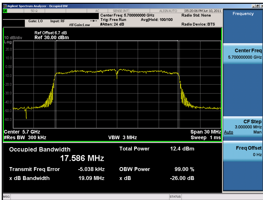
Plot 6-18. 26dB Bandwidth Plot (802.11n (UNII Band 3) – Ch. 140)
