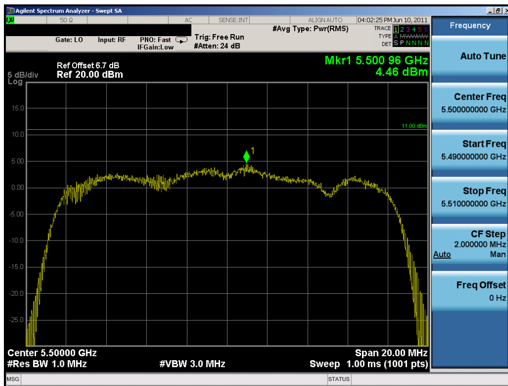
Plot 6-31. Peak Power Spectral Density Plot (802.11a (UNII Band 3) – Ch. 100)
