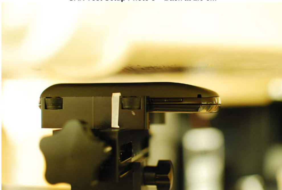
SAR Test Setup Photo 6 – Back at 1.0 cm (Extended Battery)
