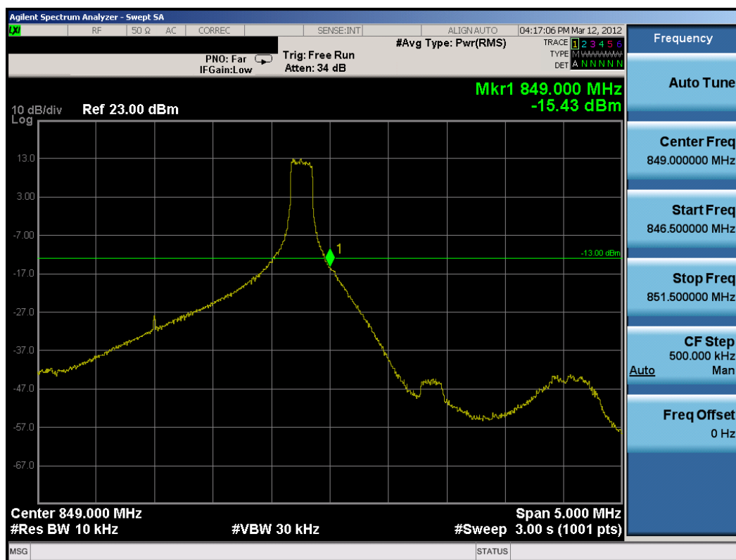
Plot 8-39. Upper Band Edge Plot (3MHz QPSK – RB Size 1, Offset 14)
