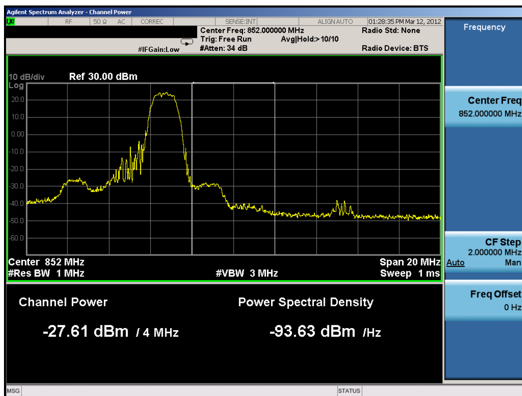
Plot 8-47. Upper Extended Band Edge Plot (5MHz QPSK – RB Size 1, Offset 24)
