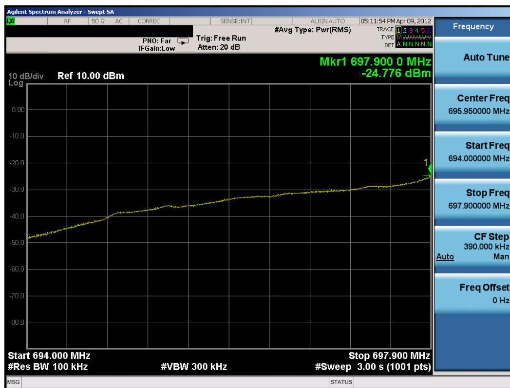
Plot 7-25. Lower Extended Band Edge Plot (5MHz QPSK – RB Size 25)
