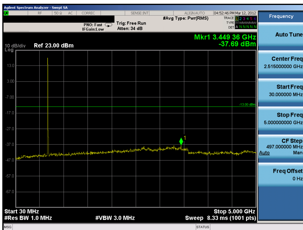
Plot 7-15. Conducted Spurious Plot (10MHz QPSK – RB Size 1, RB Offset 0 – Low Channel)
