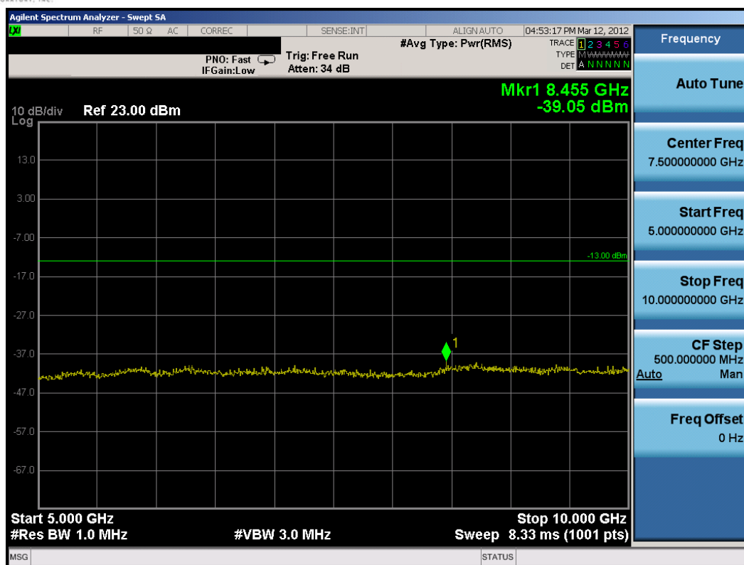
Plot 7-16. Conducted Spurious Plot (10MHz QPSK – RB Size 1, RB Offset 0 – Low Channel)
