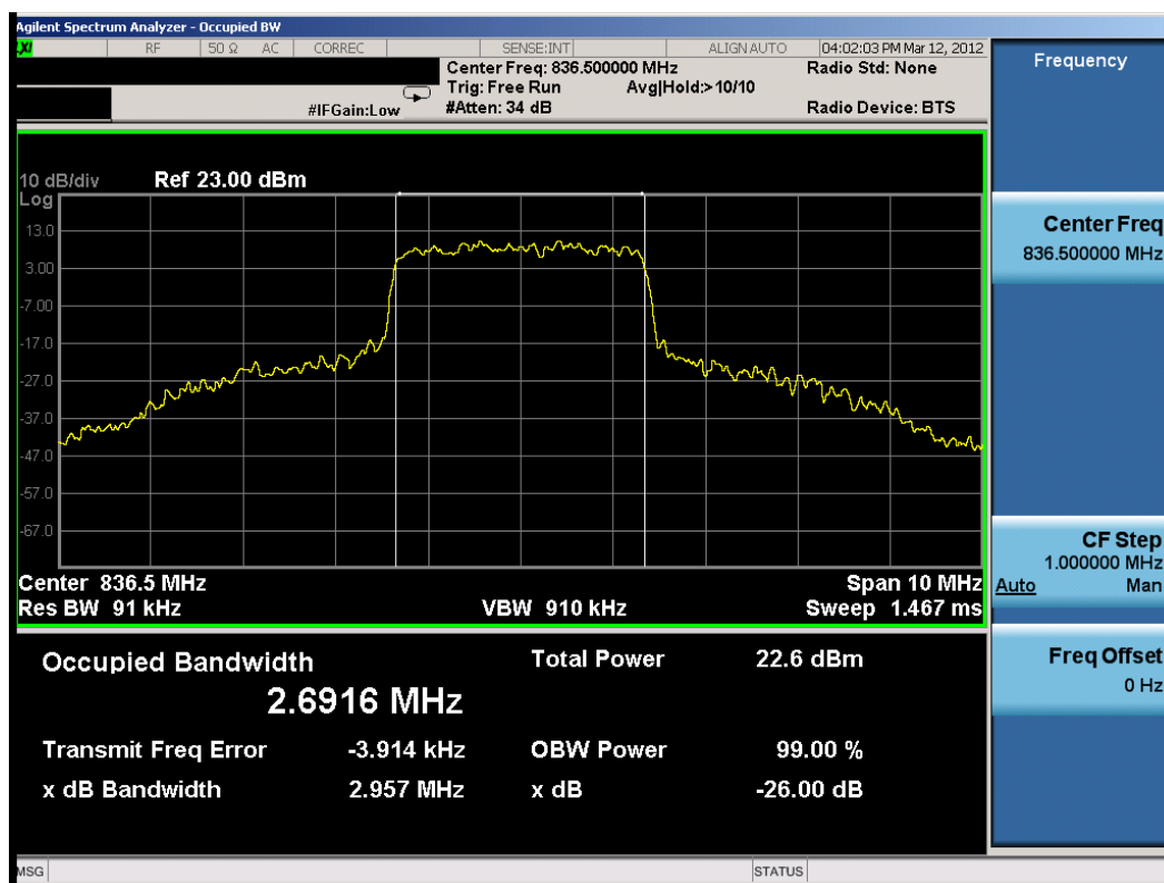
Plot 8-15. Occupied Bandwidth Plot (3MHz QPSK – RB Size 15)
