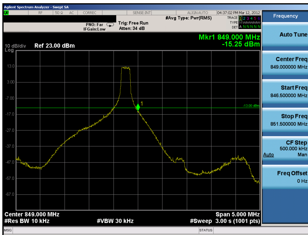
Plot 8-37. Upper Band Edge Plot (1.4MHz QPSK – RB Size 1, Offset 5)
