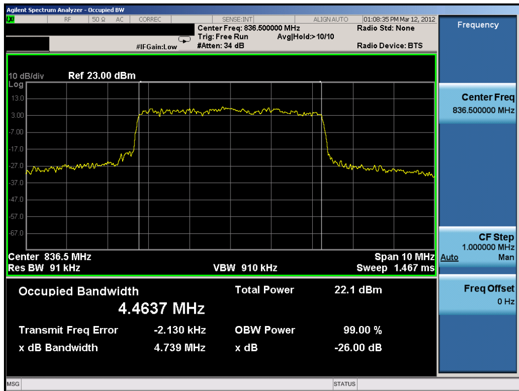
Plot 8-17. Occupied Bandwidth Plot (5MHz QPSK – RB Size 25)
