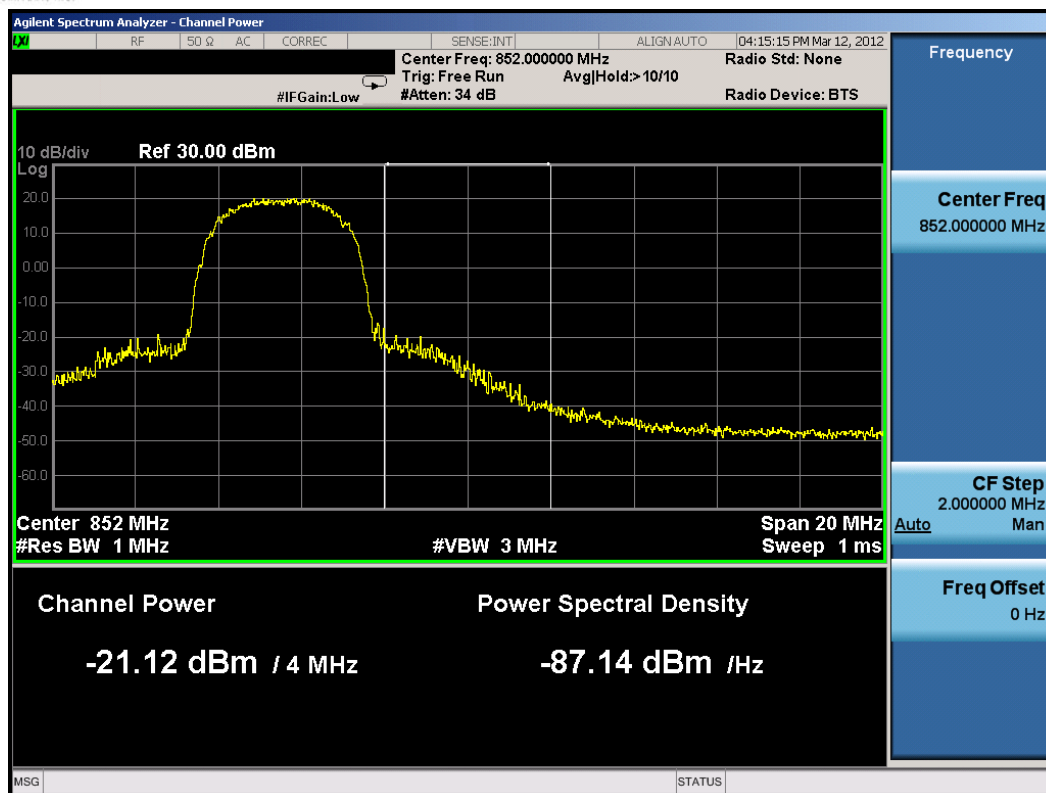
Plot 8-46. Upper Extended Band Edge Plot (3MHz QPSK – RB Size 15, Offset 0)
