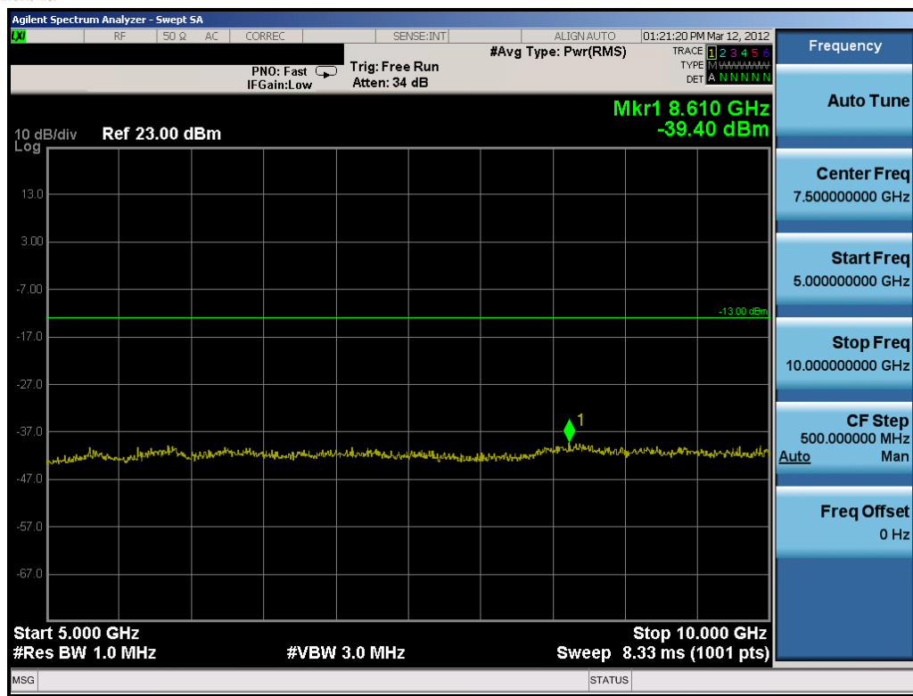
Plot 8-36. Conducted Spurious Plot (5MHz QPSK – RB Size 1, RB Offset 0 – High Channel)
