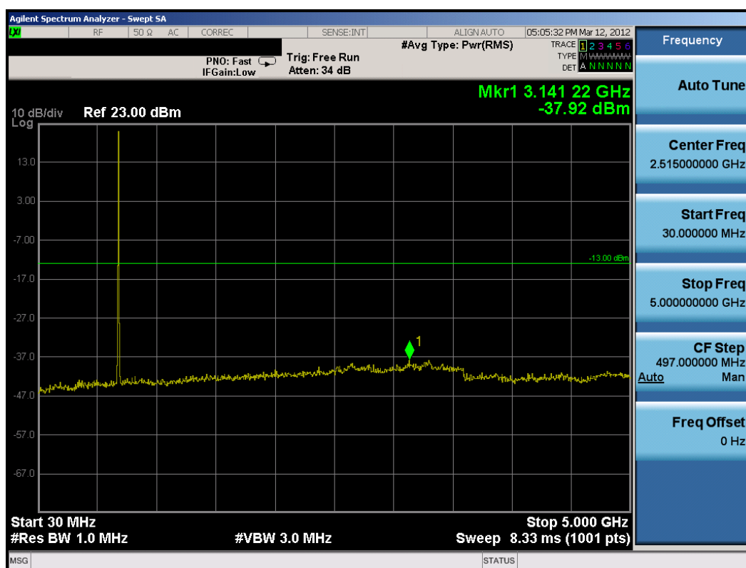
Plot 7-11. Conducted Spurious Plot (5MHz QPSK – RB Size 1, RB Offset 0 – Mid Channel)
