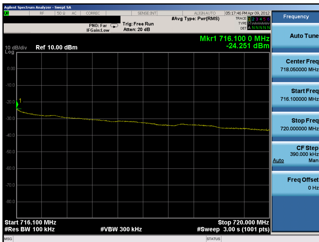
Plot 7-29. Upper Extended Band Edge Plot (5MHz QPSK – RB Size 25)
