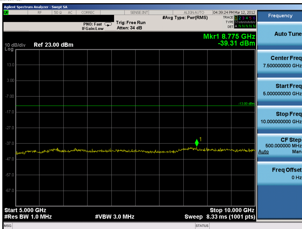
Plot 8-24. Conducted Spurious Plot (1.4MHz QPSK – RB Size 1, RB Offset 0 – High Channel)
