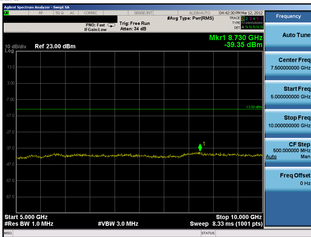
Plot 7-18. Conducted Spurious Plot (10MHz QPSK – RB Size 1, RB Offset 0 – Mid Channel)
