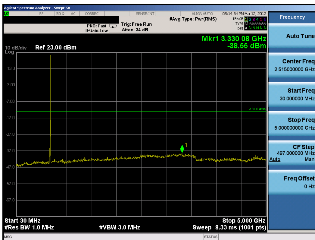
Plot 7-13. Conducted Spurious Plot (5MHz QPSK – RB Size 1, RB Offset 0 – High Channel)
