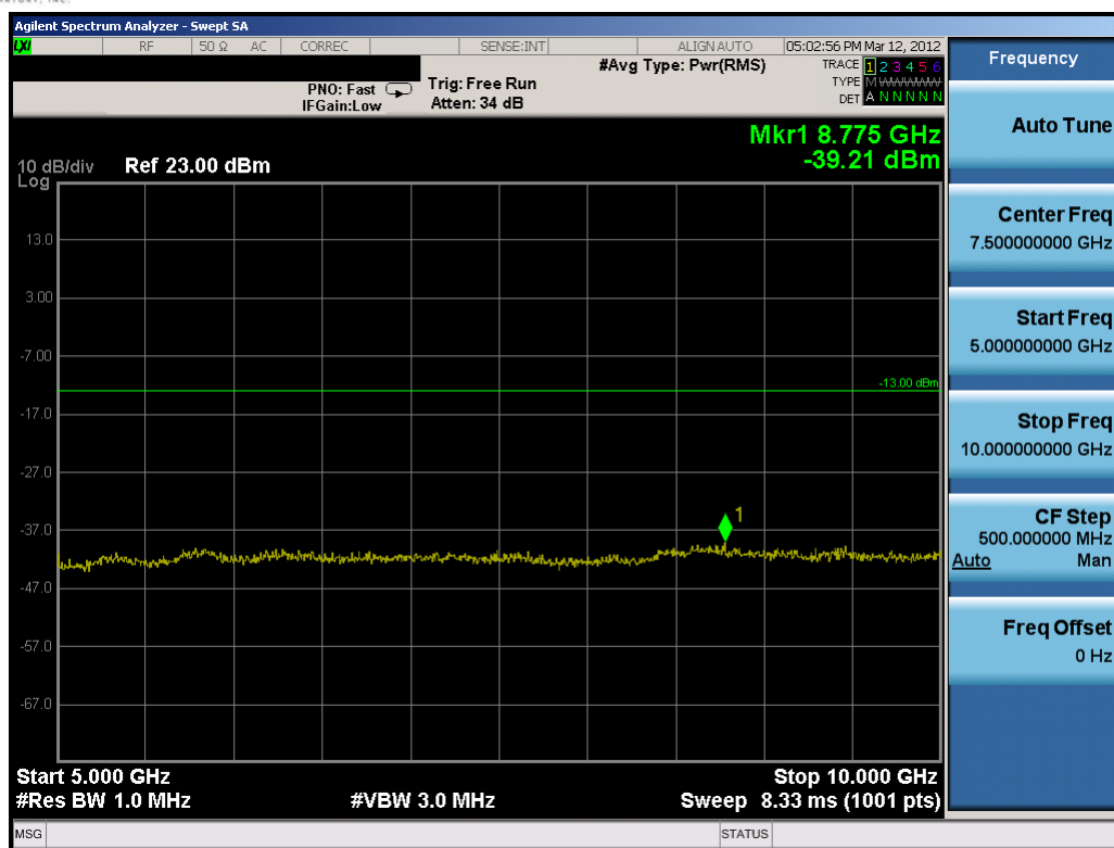
Plot 7-20. Conducted Spurious Plot (10MHz QPSK – RB Size 1, RB Offset 0 – High Channel)
