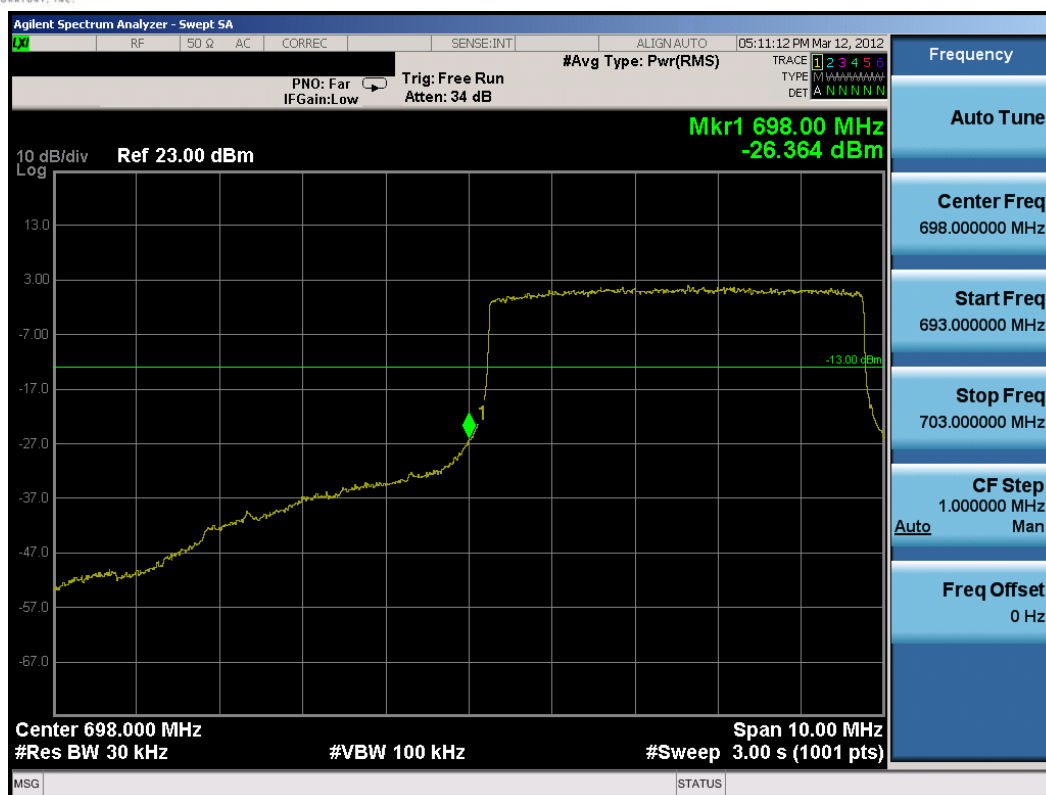
Plot 7-2. Lower Band Edge Plot (5MHz QPSK – RB Size 25, Offset 0)
