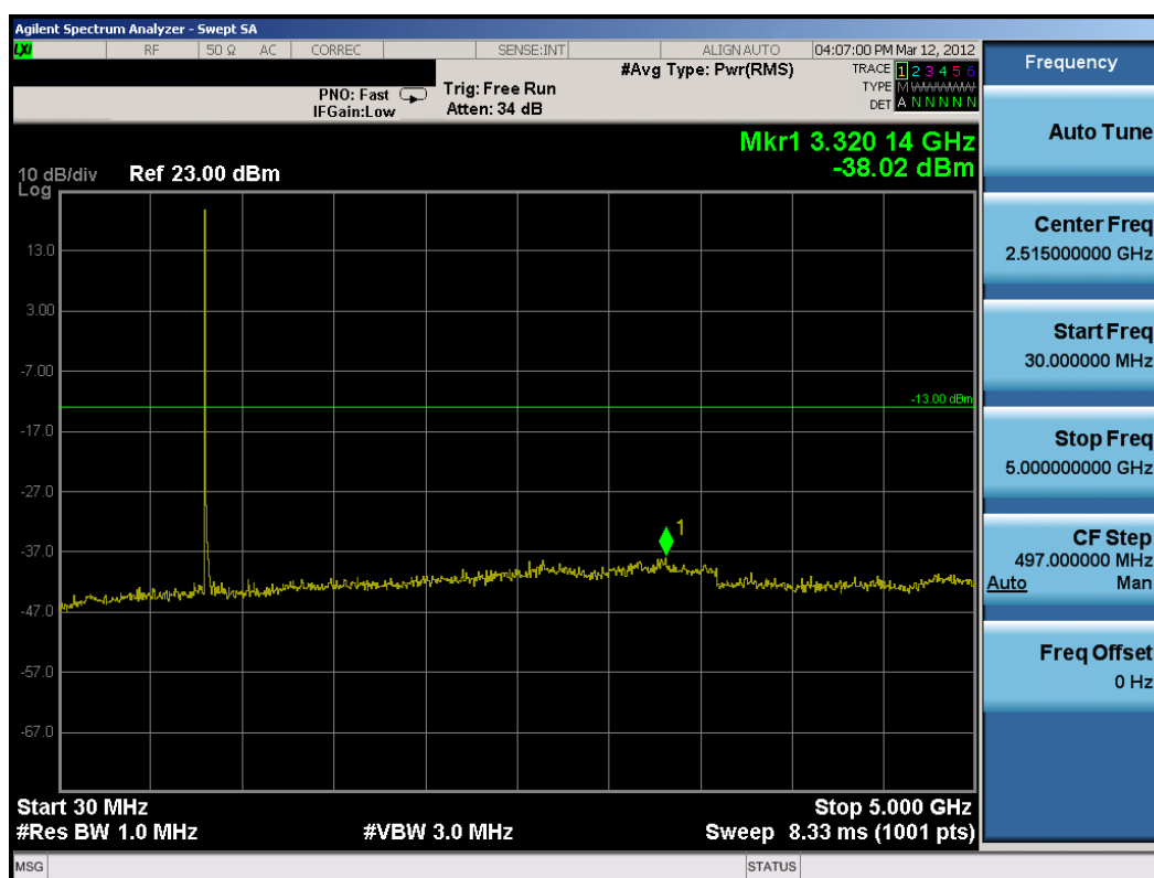
Plot 8-25. Conducted Spurious Plot (3MHz QPSK – RB Size 1, RB Offset 0 – Low Channel)
