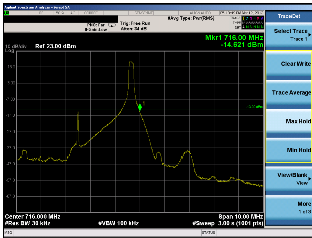
Plot 7-21. Upper Band Edge Plot (5MHz QPSK – RB Size 1, Offset 24)
