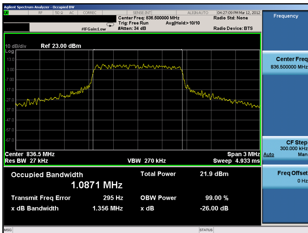
Plot 8-13. Occupied Bandwidth Plot (1.4MHz QPSK – RB Size 6)
