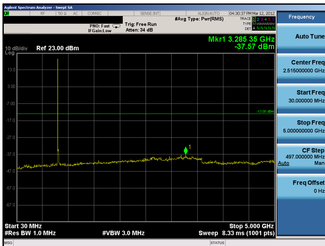
Plot 8-19. Conducted Spurious Plot (1.4MHz QPSK – RB Size 1, RB Offset 0 – Low Channel)
