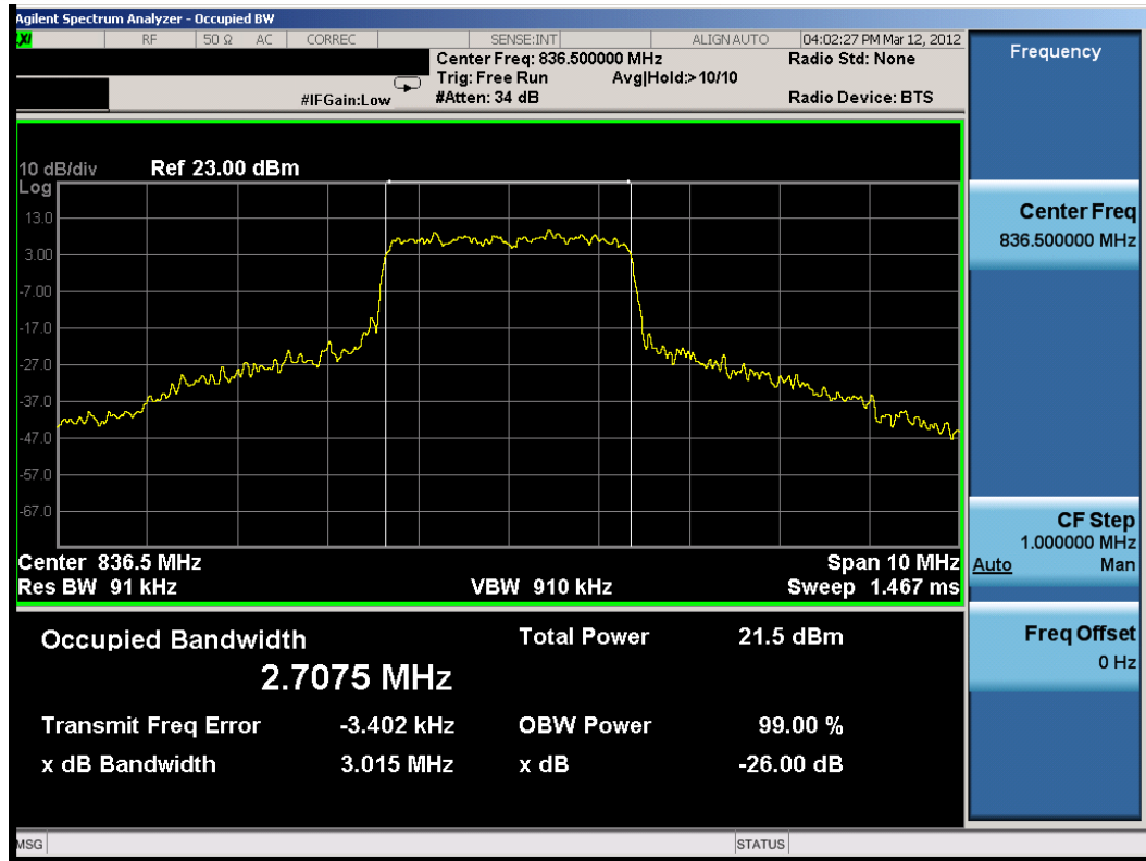
Plot 8-16. Occupied Bandwidth Plot (3MHz 16-QAM – RB Size 15)
