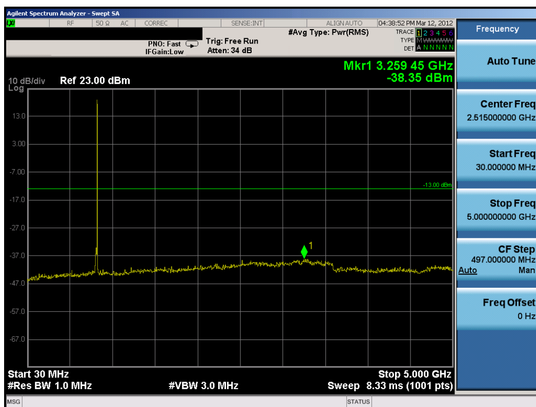
Plot 8-23. Conducted Spurious Plot (1.4MHz QPSK – RB Size 1, RB Offset 0 – High Channel)
