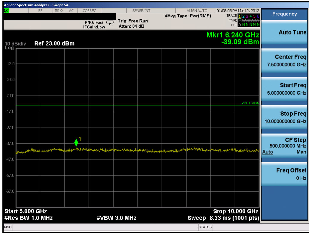
Plot 8-34. Conducted Spurious Plot (5MHz QPSK – RB Size 1, RB Offset 0 – Mid Channel)
