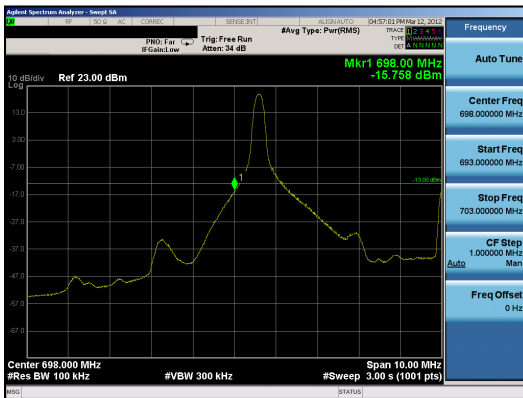
Plot 7-3. Lower Band Edge Plot (10MHz QPSK – RB Size 1, Offset 0)
