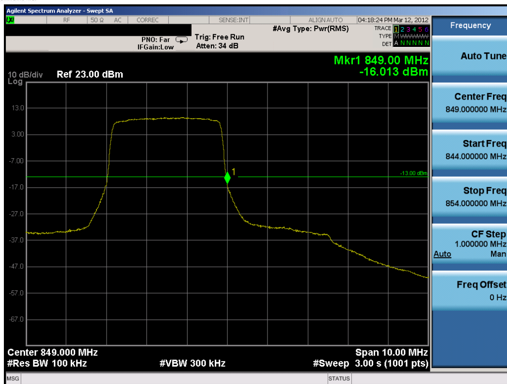
Plot 8-40. Upper Band Edge Plot (3MHz QPSK – RB Size 15, Offset 0)
