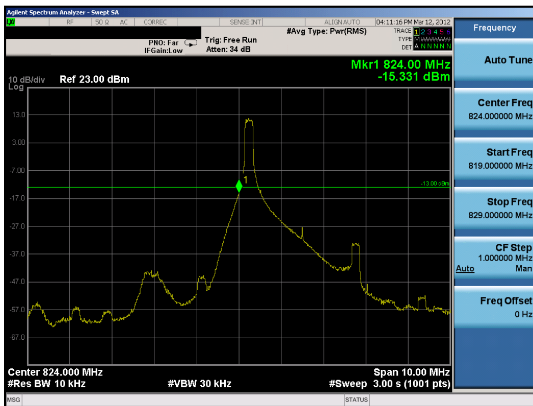
Plot 8-3. Lower Band Edge Plot (3MHz QPSK – RB Size 1, Offset 0)
