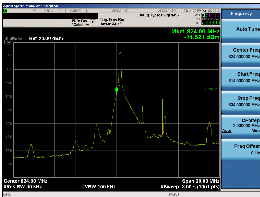
Plot 8-5. Lower Band Edge Plot (5MHz QPSK – RB Size 1, Offset 0)
