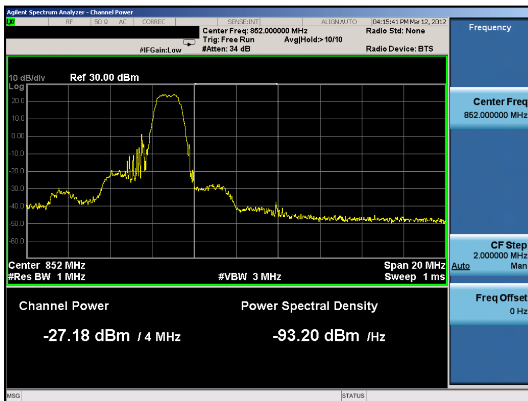
Plot 8-45. Upper Extended Band Edge Plot (3MHz QPSK – RB Size 1, Offset 14)
