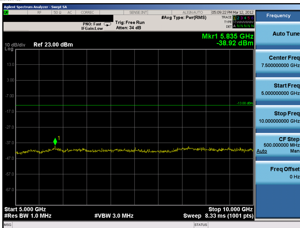
Plot 7-10. Conducted Spurious Plot (5MHz QPSK – RB Size 1, RB Offset 0 – Low Channel)
