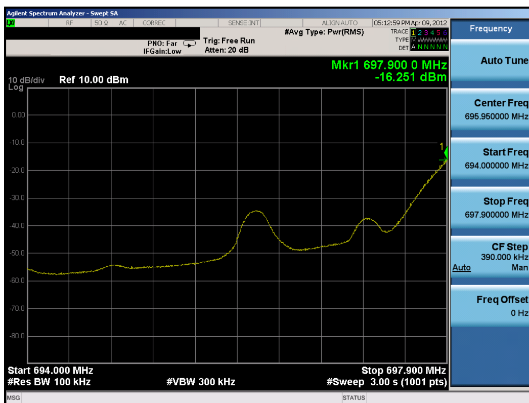
Plot 7-27. Lower Extended Band Edge Plot (5MHz QPSK – RB Size 1)
