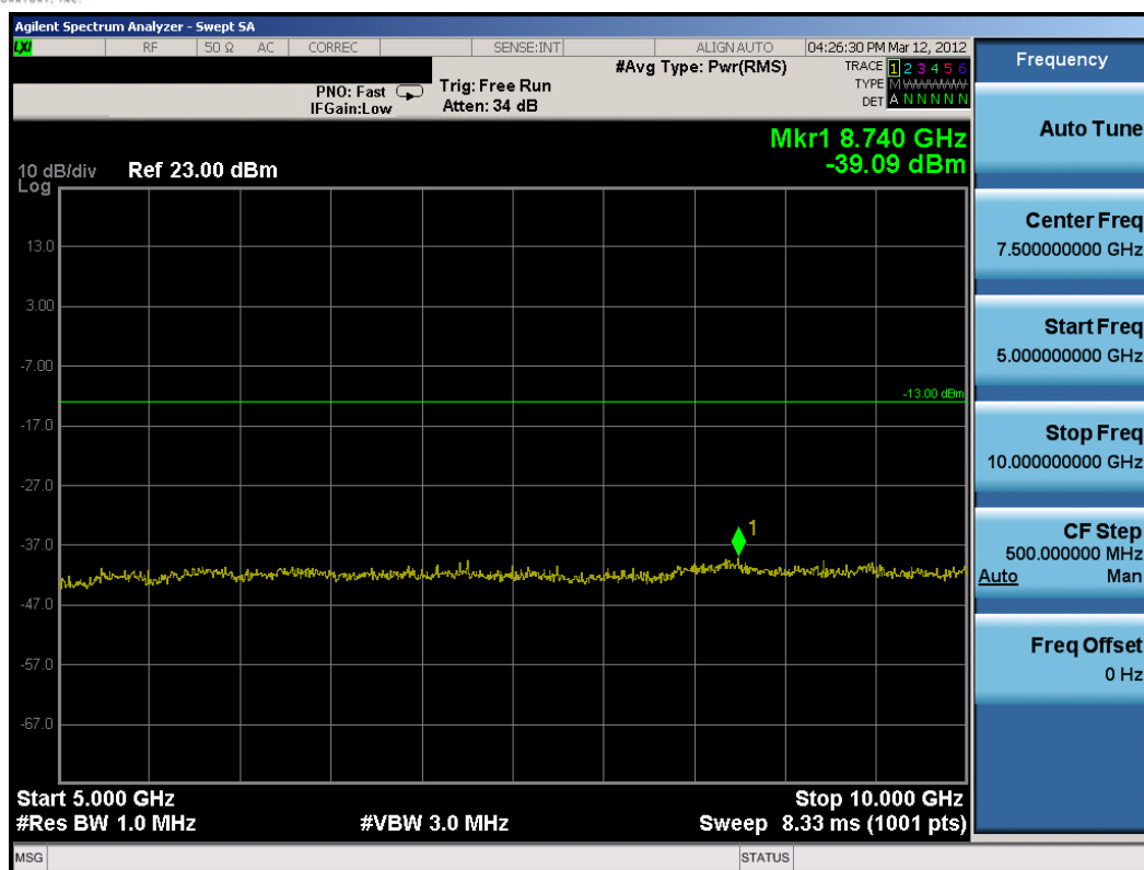
Plot 8-22. Conducted Spurious Plot (1.4MHz QPSK – RB Size 1, RB Offset 0 – Mid Channel)
