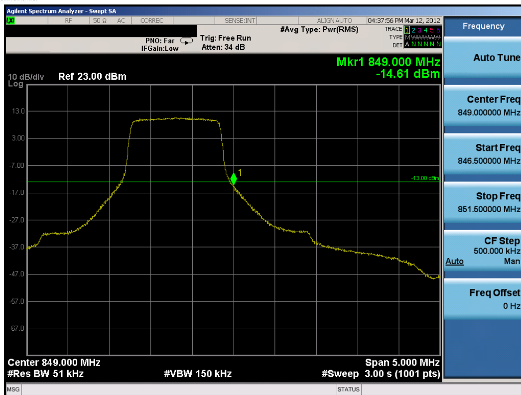
Plot 8-38. Upper Band Edge Plot (1.4MHz QPSK – RB Size 6, Offset 0)
