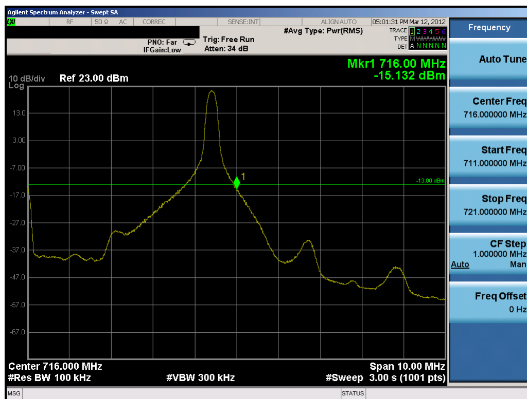
Plot 7-23. Upper Band Edge Plot (10MHz QPSK – RB Size 1, Offset 49)
