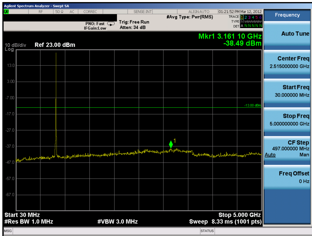
Plot 8-35. Conducted Spurious Plot (5MHz QPSK – RB Size 1, RB Offset 0 – High Channel)
