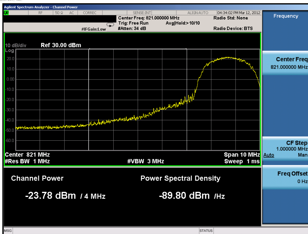
Plot 8-8. Lower Extended Band Edge Plot (1.4MHz QPSK – RB Size 6, Offset 0)
