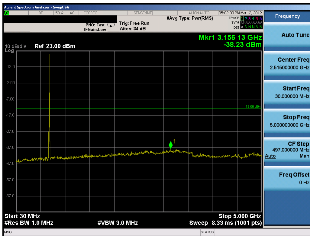
Plot 7-19. Conducted Spurious Plot (10MHz QPSK – RB Size 1, RB Offset 0 – High Channel)
