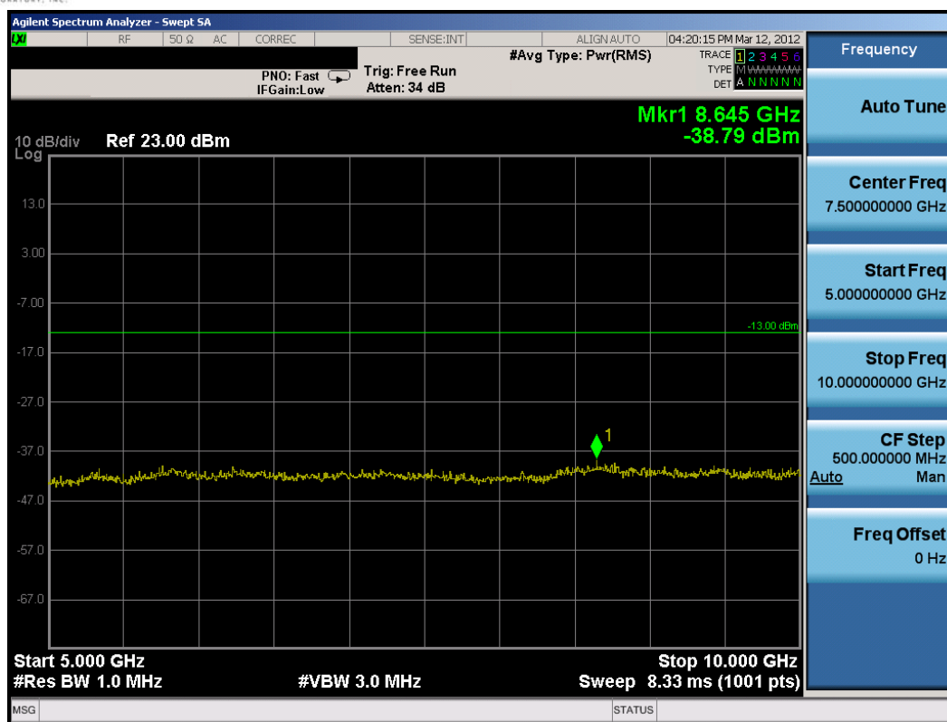
Plot 8-30. Conducted Spurious Plot (3MHz QPSK – RB Size 1, RB Offset 0 – High Channel)
