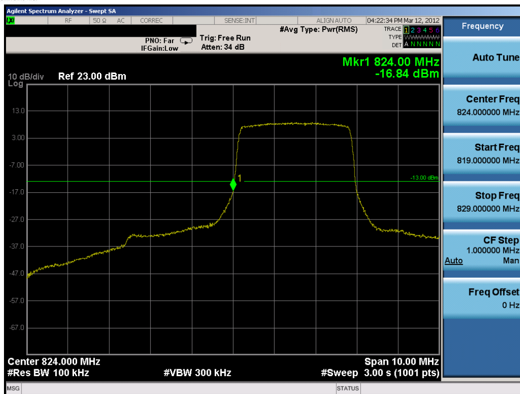
Plot 8-4. Lower Band Edge Plot (3MHz QPSK – RB Size 15, Offset 0)
