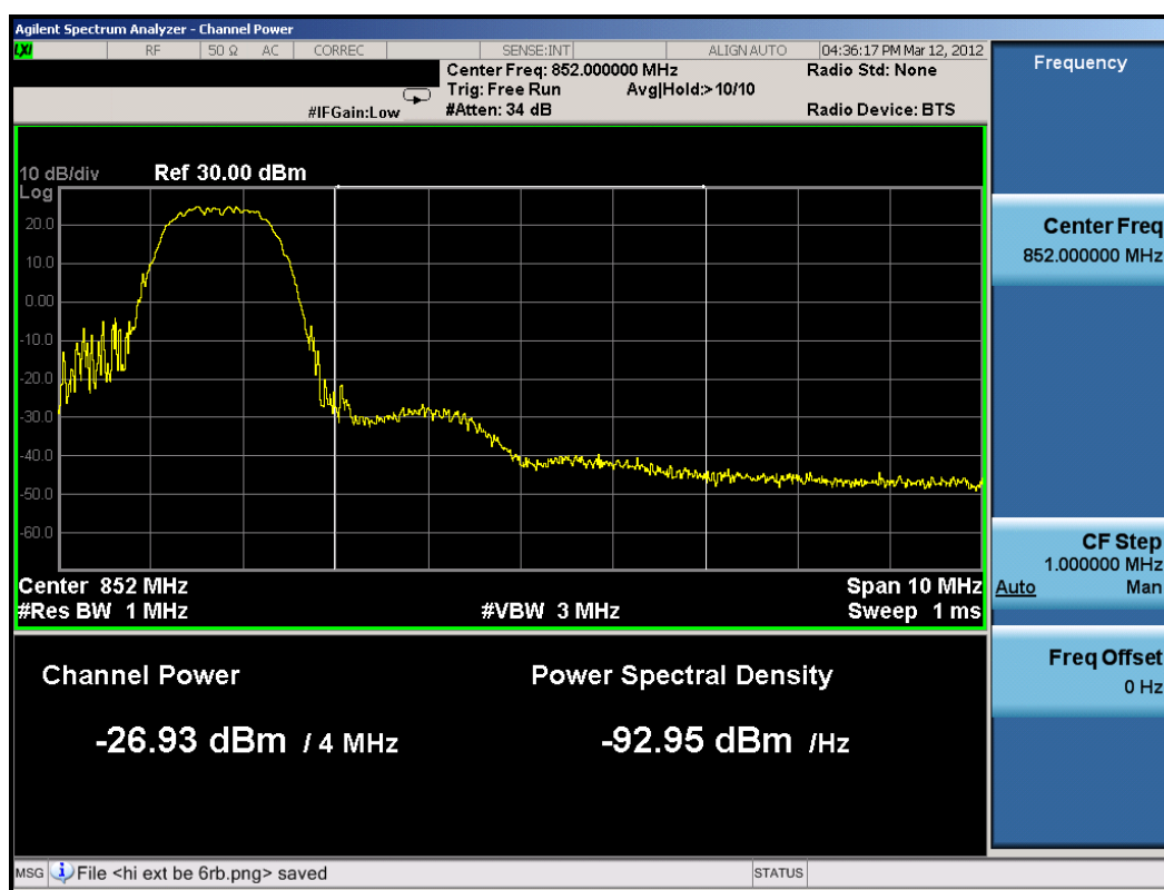
Plot 8-43. Upper Extended Band Edge Plot (1.4MHz QPSK – RB Size 1, Offset 5)
