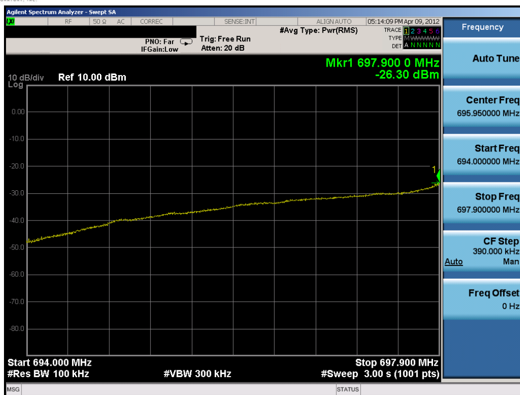
Plot 7-26. Lower Extended Band Edge Plot (5MHz 16QAM – RB Size 25)
