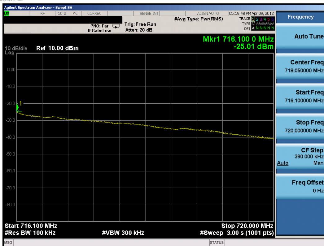
Plot 7-30. Upper Extended Band Edge Plot (5MHz 16QAM – RB Size 25)
