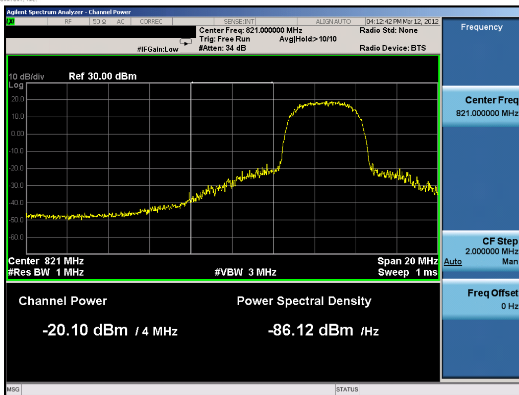
Plot 8-10. Lower Extended Band Edge Plot (3MHz QPSK – RB Size 15, Offset 0)
