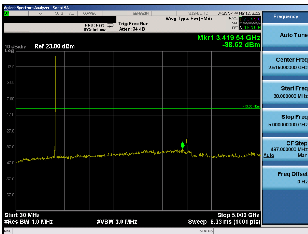
Plot 8-21. Conducted Spurious Plot (1.4MHz QPSK – RB Size 1, RB Offset 0 – Mid Channel)
