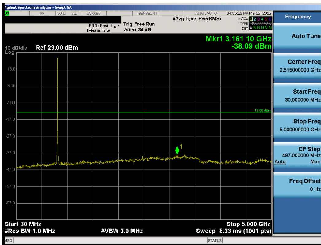
Plot 8-27. Conducted Spurious Plot (3MHz QPSK – RB Size 1, RB Offset 0 – Mid Channel)
