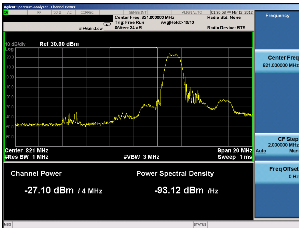
Plot 8-11. Lower Extended Band Edge Plot (5MHz QPSK – RB Size 1, Offset 0)
