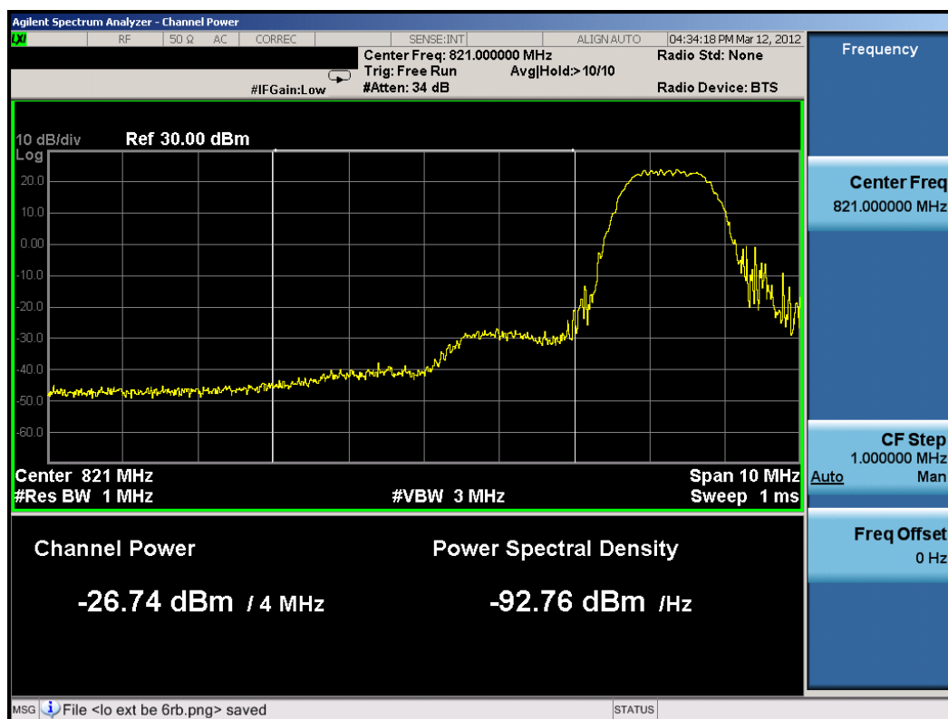
Plot 8-7. Lower Extended Band Edge Plot (1.4MHz QPSK – RB Size 1, Offset 0)
