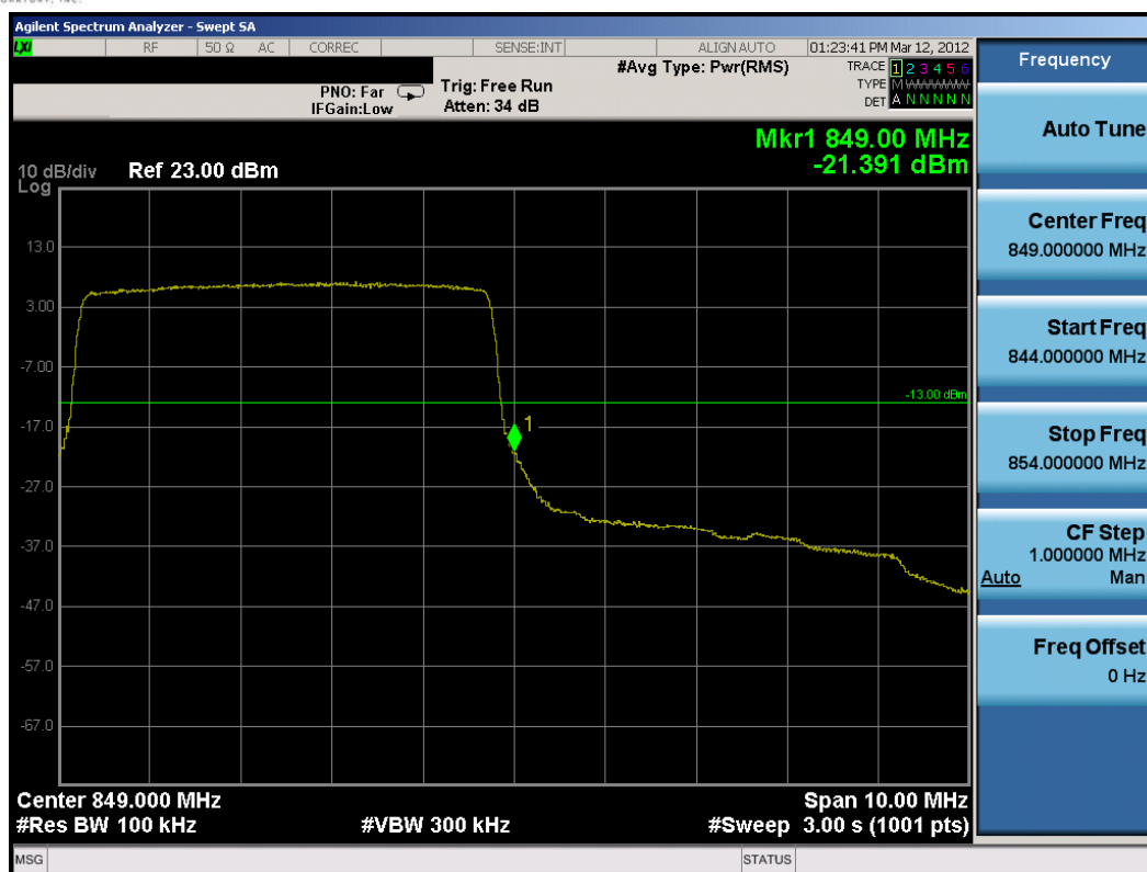
Plot 8-42. Upper Band Edge Plot (5MHz QPSK – RB Size 25, Offset 0)
