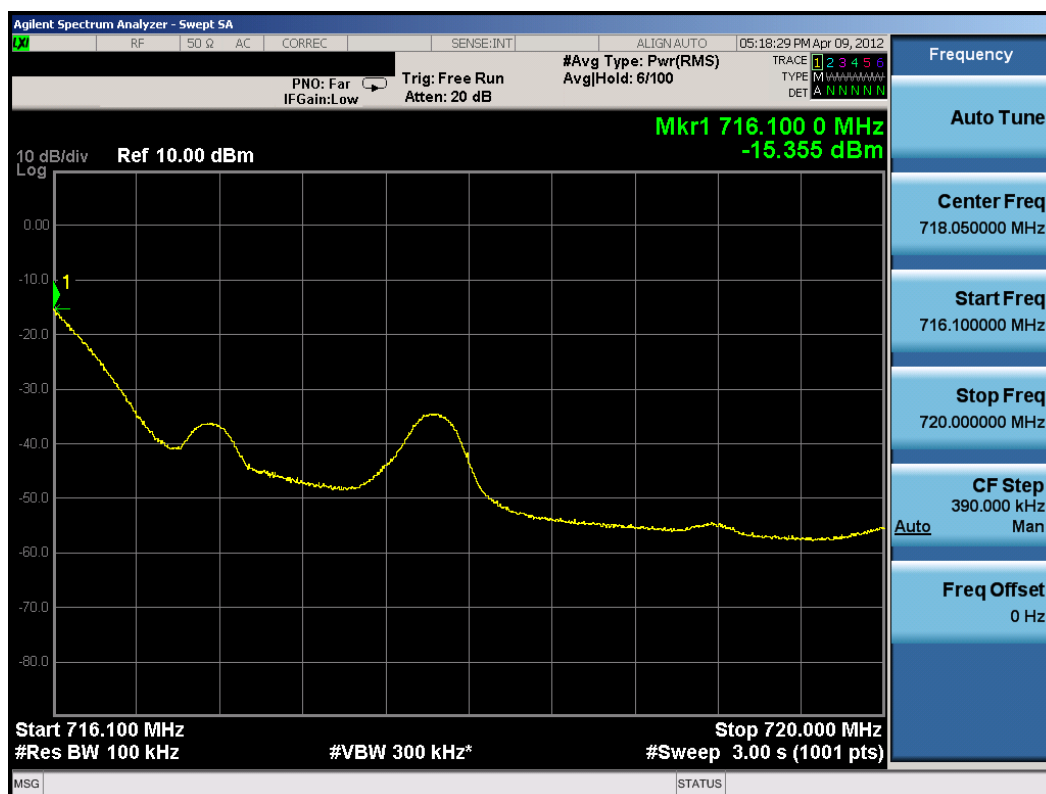
Plot 7-31. Upper Extended Band Edge Plot (5MHz QPSK – RB Size 1)
