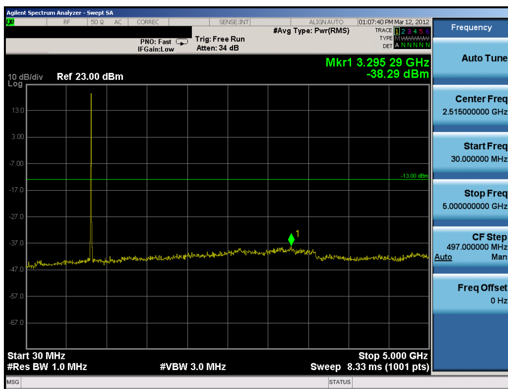
Plot 8-33. Conducted Spurious Plot (5MHz QPSK – RB Size 1, RB Offset 0 – Mid Channel)
