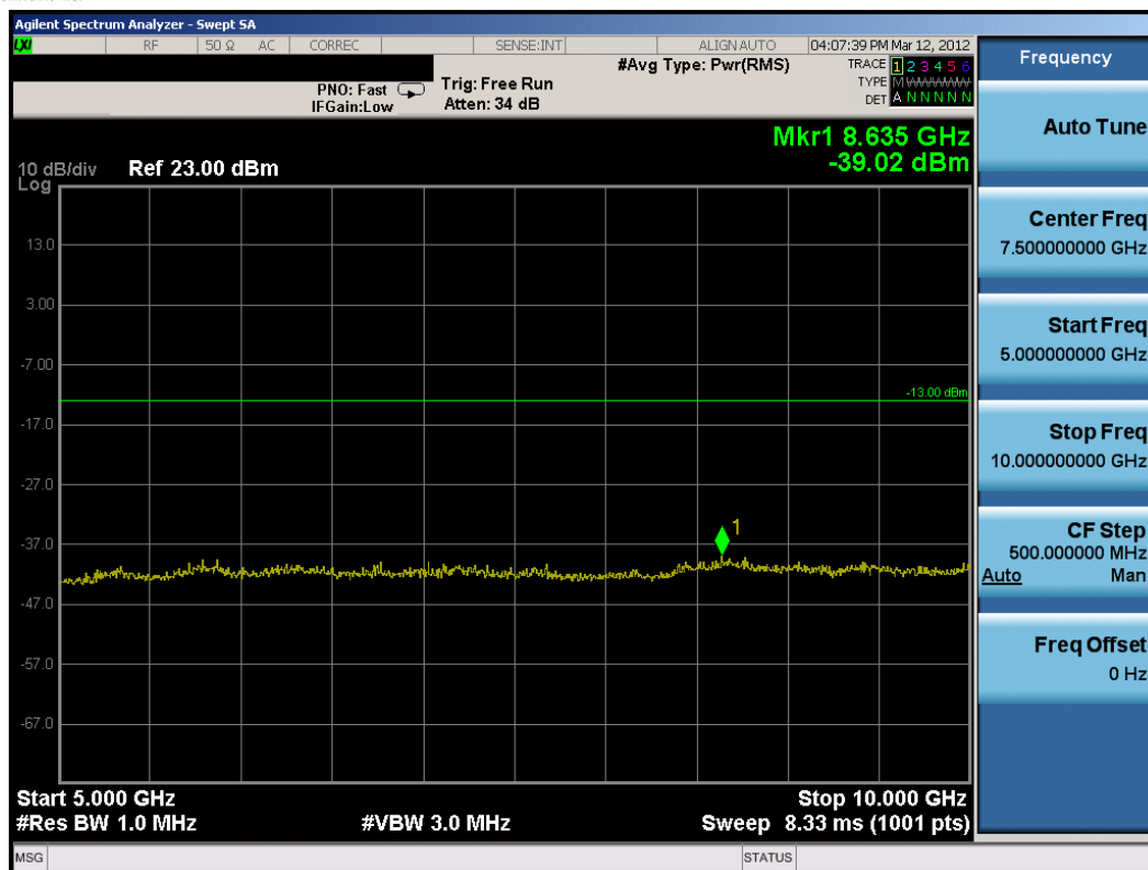
Plot 8-26. Conducted Spurious Plot (3MHz QPSK – RB Size 1, RB Offset 0 – Low Channel)
