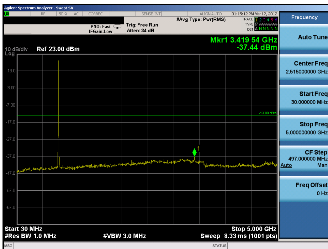
Plot 8-31. Conducted Spurious Plot (5MHz QPSK – RB Size 1, RB Offset 0 – Low Channel)
