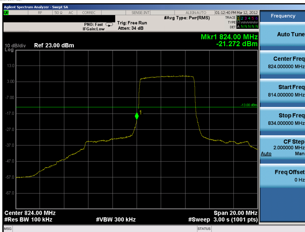
Plot 8-6. Lower Band Edge Plot (5MHz QPSK – RB Size 25, Offset 0)
