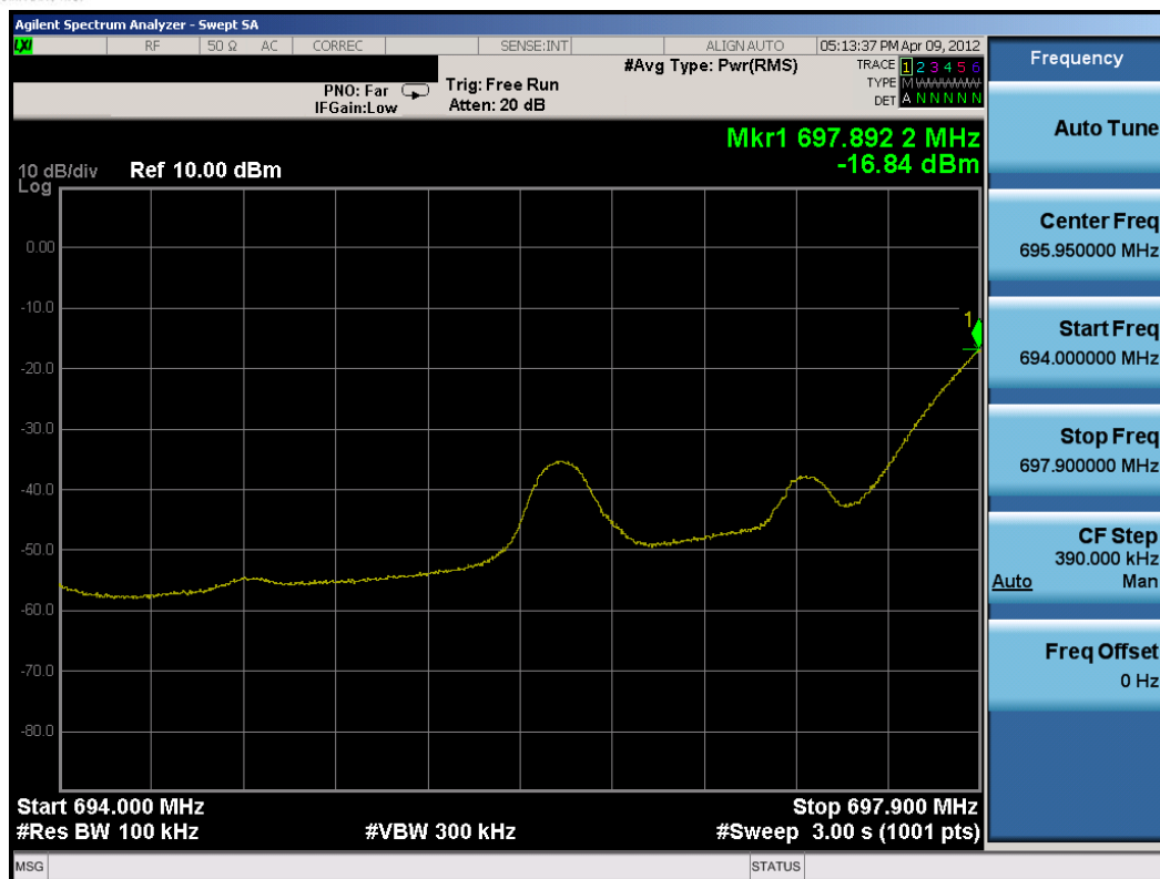
Plot 7-28. Lower Extended Band Edge Plot (5MHz 16QAM – RB Size 1)
