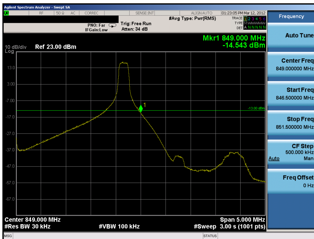
Plot 8-41. Upper Band Edge Plot (5MHz QPSK – RB Size 1, Offset 24)
