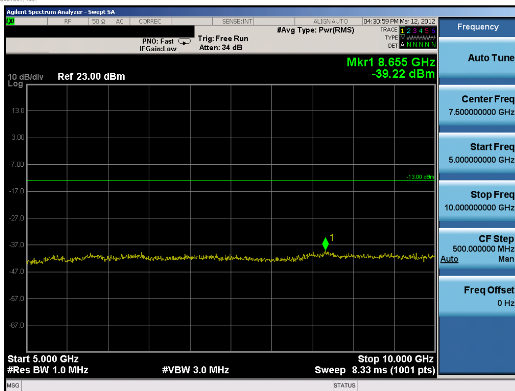
Plot 8-20. Conducted Spurious Plot (1.4MHz QPSK – RB Size 1, RB Offset 0 – Low Channel)
