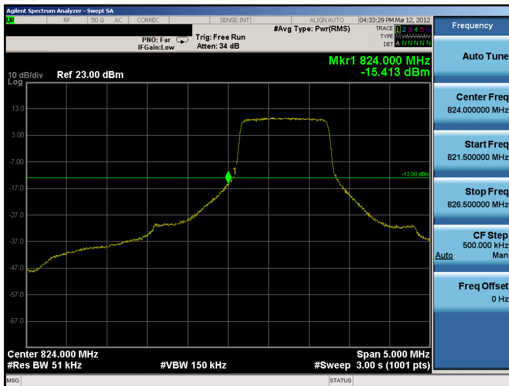
Plot 8-2. Lower Band Edge Plot (1.4MHz QPSK – RB Size 6, Offset 0)
