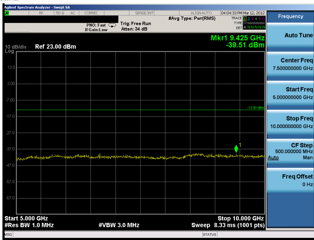
Plot 8-28. Conducted Spurious Plot (3MHz QPSK – RB Size 1, RB Offset 0 – Mid Channel)
