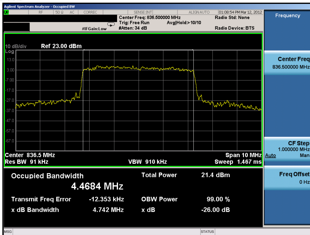
Plot 8-18. Occupied Bandwidth Plot (5MHz 16-QAM – RB Size 25)
