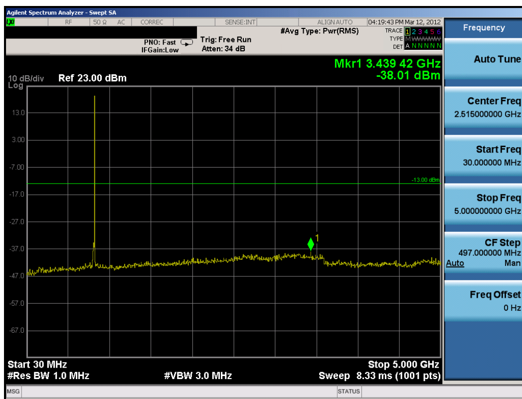
Plot 8-29. Conducted Spurious Plot (3MHz QPSK – RB Size 1, RB Offset 0 – High Channel)
