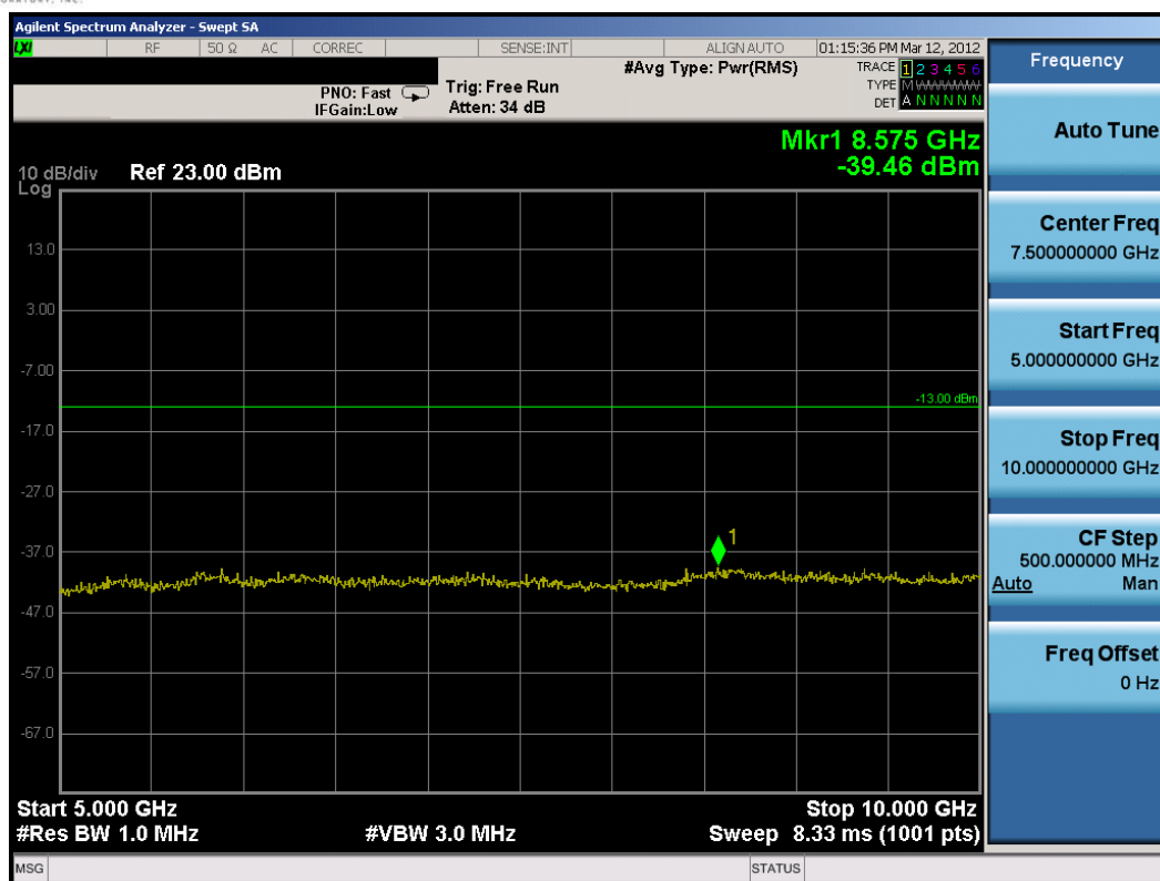
Plot 8-32. Conducted Spurious Plot (5MHz QPSK – RB Size 1, RB Offset 0 – Low Channel)
