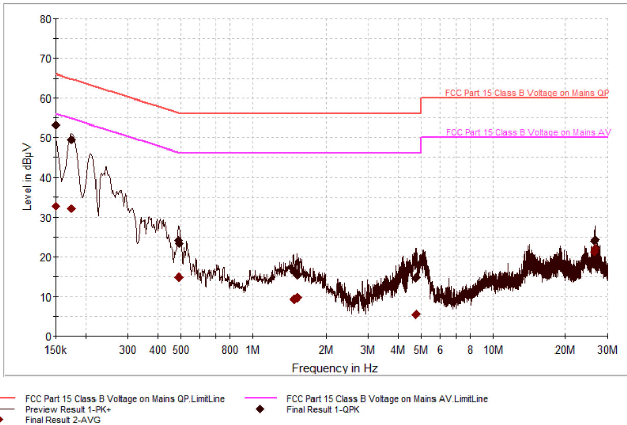
Plot 7-2. Line-Conducted Test Plot (N)
