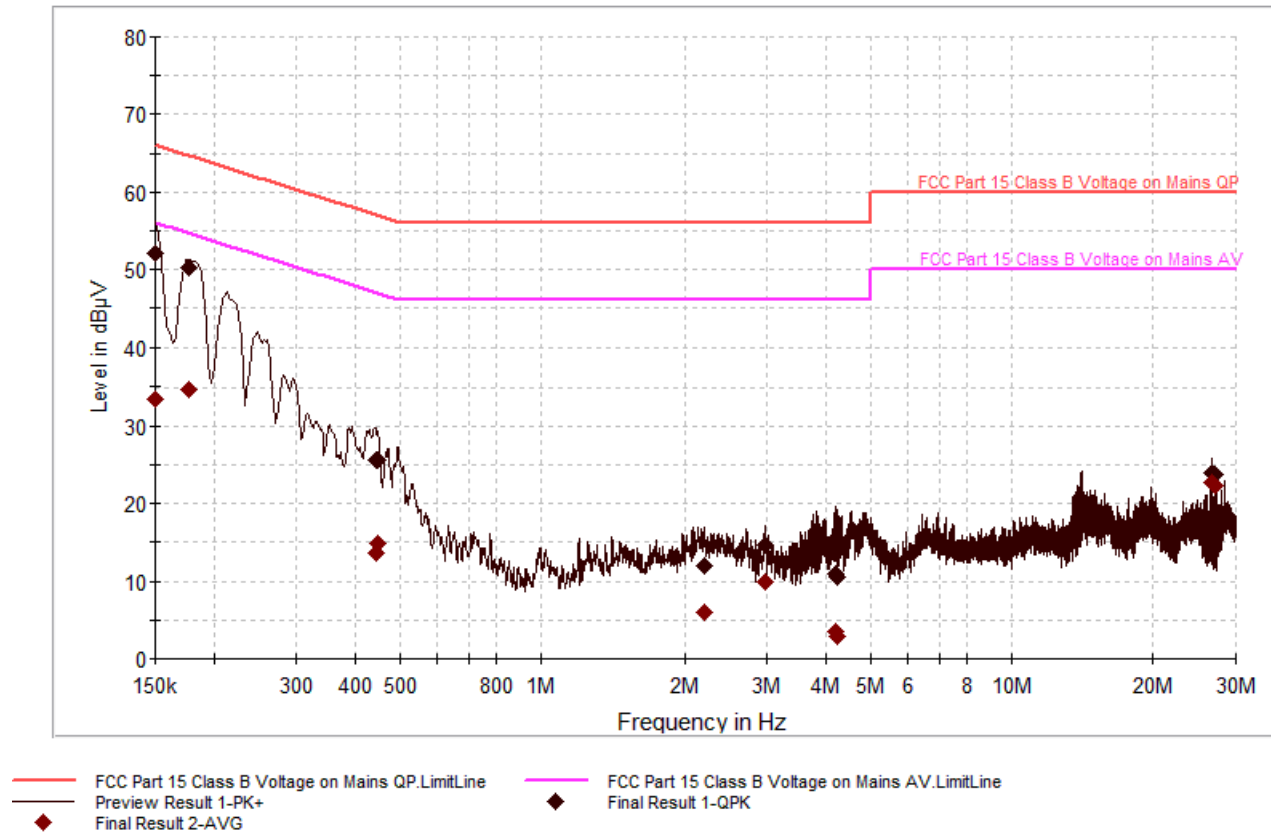
Plot 7-1. Line-Conducted Test Plot (Line 1)
