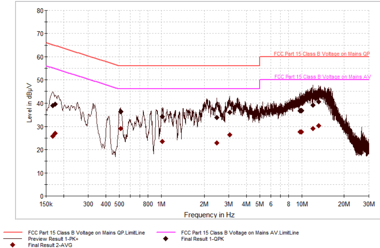
Plot 6-60. Line Conducted Plot with 802.11a (UNII Band 3) N
