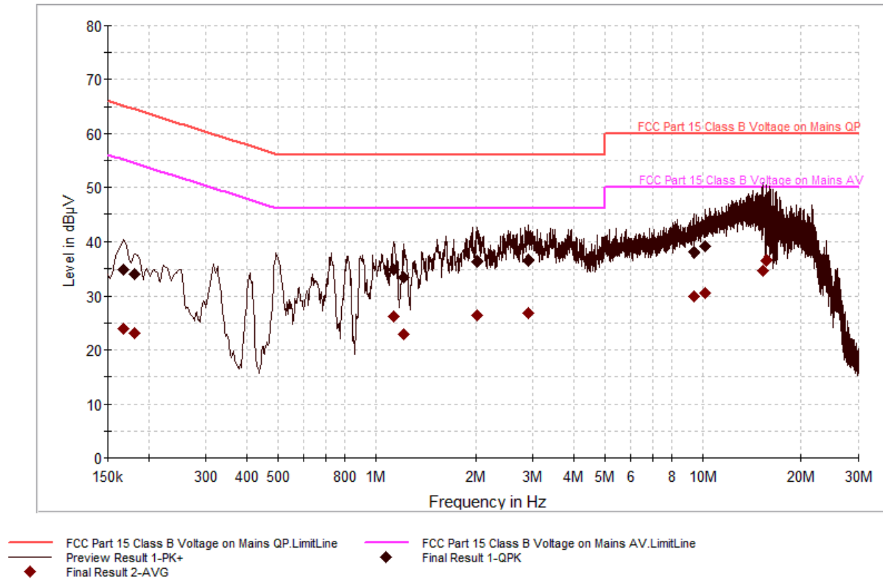
Plot 6-58. Line Conducted Plot with 802.11a (UNII Band 2) N
