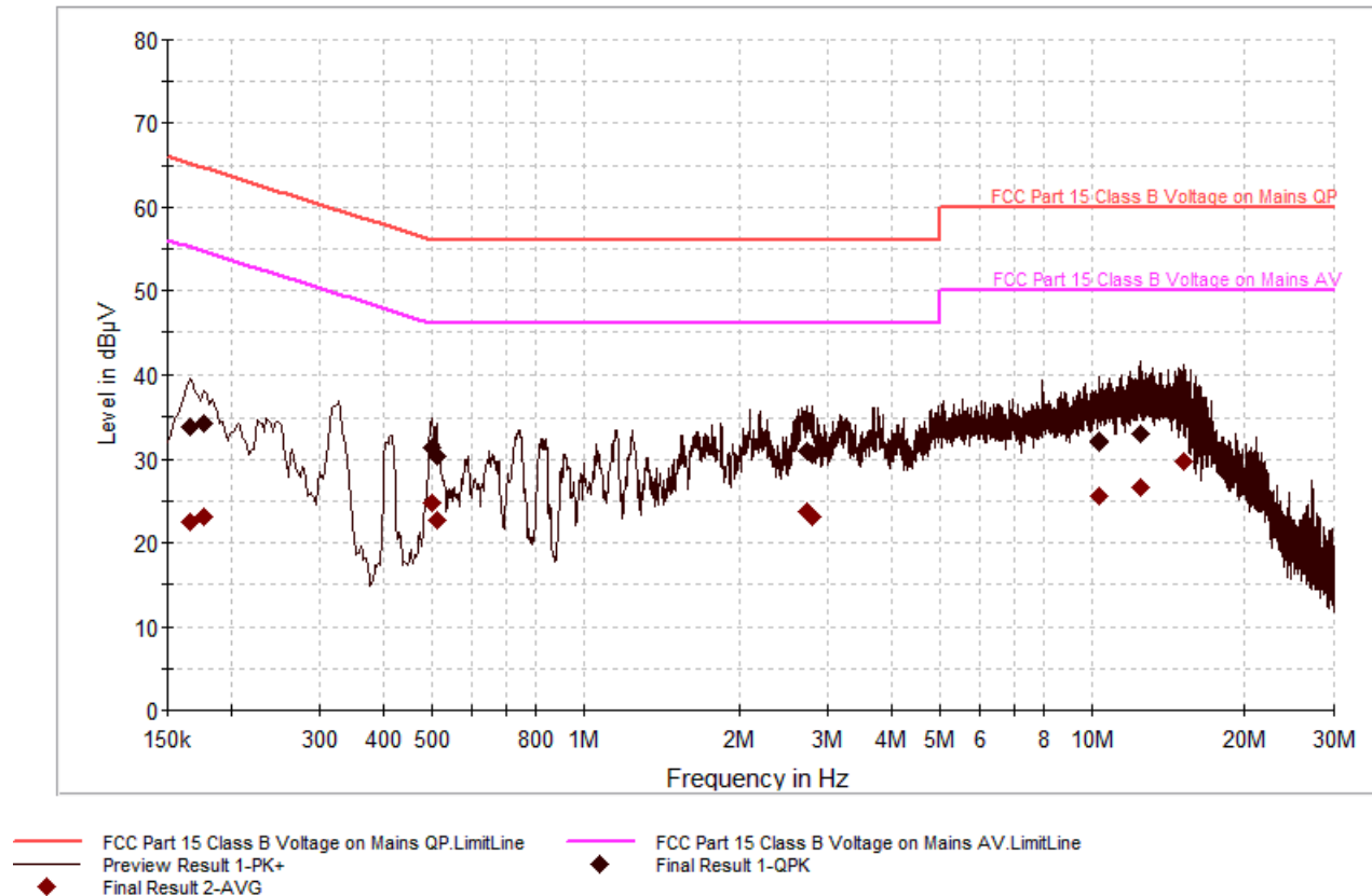
Plot 6-57. Line Conducted Plot with 802.11a (UNII Band 2) Line 1
