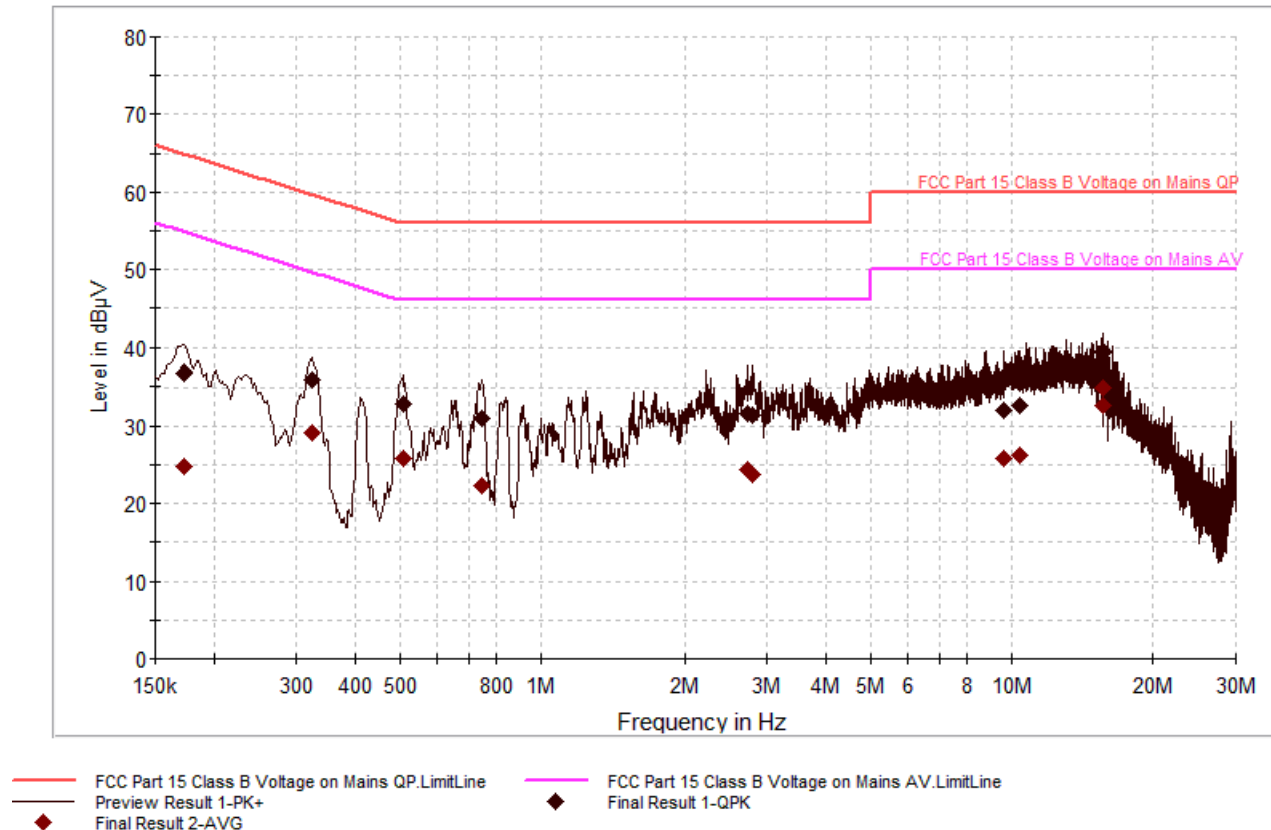
Plot 6-55. Line Conducted Plot with 802.11a (UNII Band 1) Line 1
