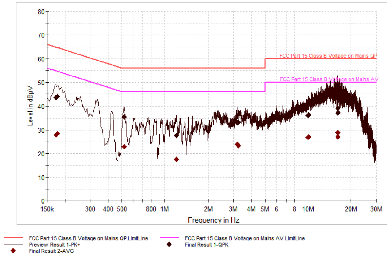
Plot 6-59. Line Conducted Plot with 802.11a (UNII Band 3) Line 1
