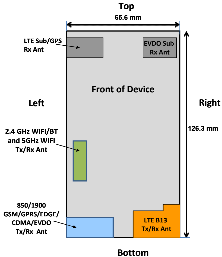
Figure 1-2 DUT Antenna Locations
