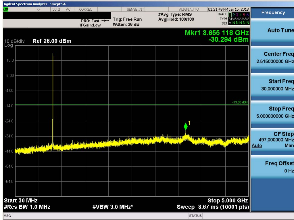
Plot 7-56. Conducted Spurious Plot (Cellular WCDMA Mode – Ch. 4183)
