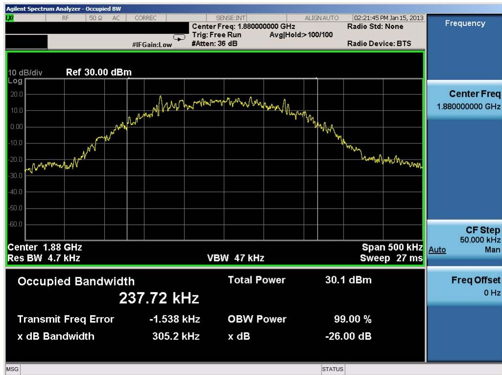
Plot 7-27. Occupied Bandwidth Plot (EDGE1900 Mode – Ch. 661)
