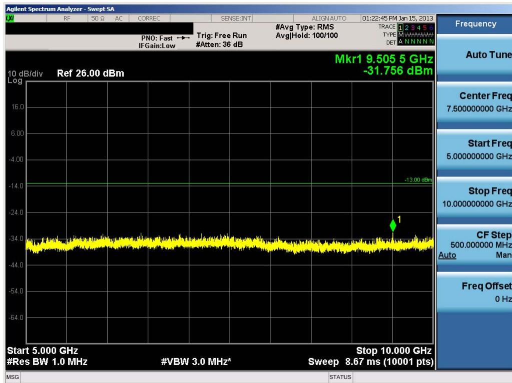
Plot 7-53. Conducted Spurious Plot (Cellular WCDMA Mode – Ch. 4132)
