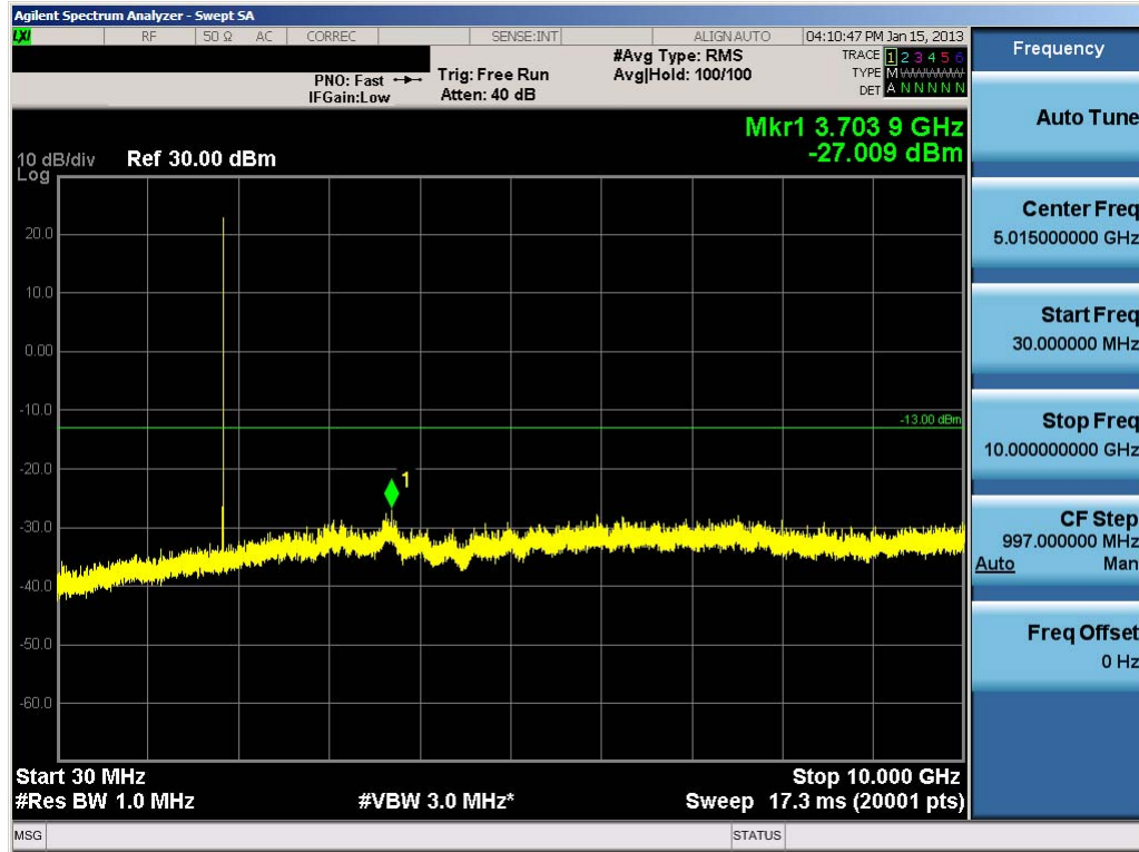
Plot 7-40. Conducted Spurious Plot (PCS CDMA Mode – Ch. 25)
