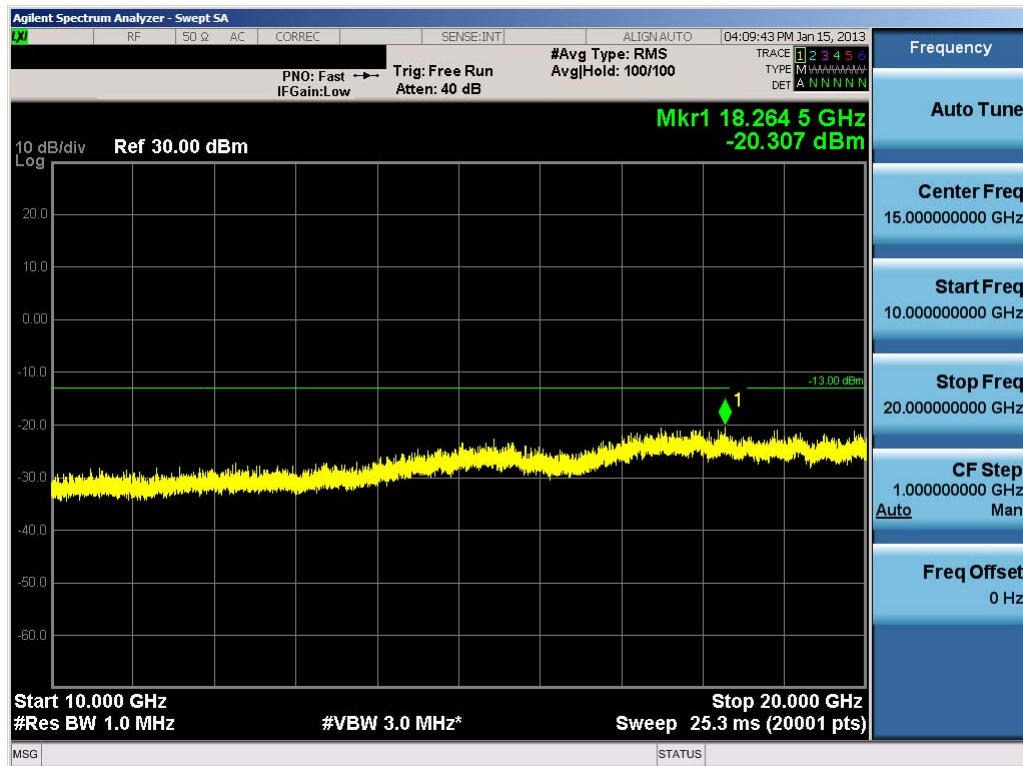
Plot 7-49. Conducted Spurious Plot (PCS CDMA Mode – Ch. 1175)
