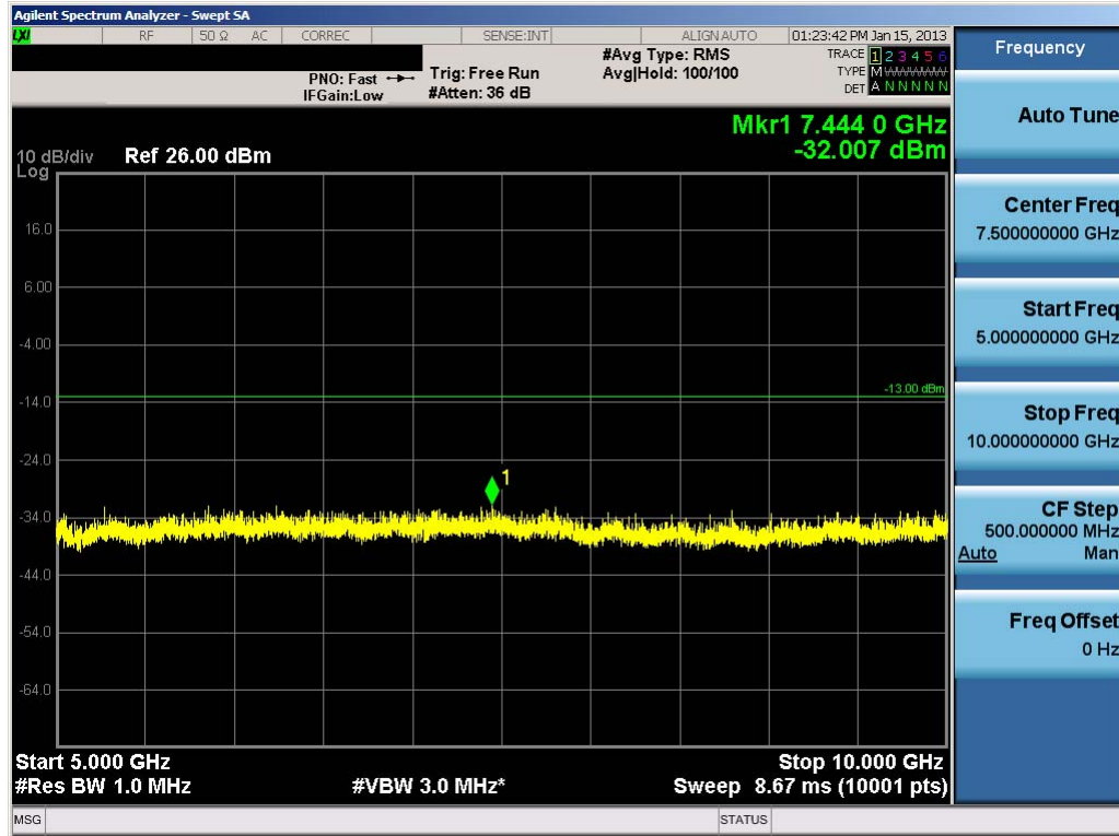
Plot 7-60. Conducted Spurious Plot (Cellular WCDMA Mode – Ch. 4233)
