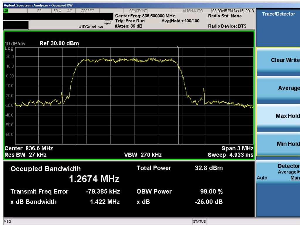
Plot 7-35. Occupied Bandwidth Plot (Cellular CDMA Mode – Ch. 384)
