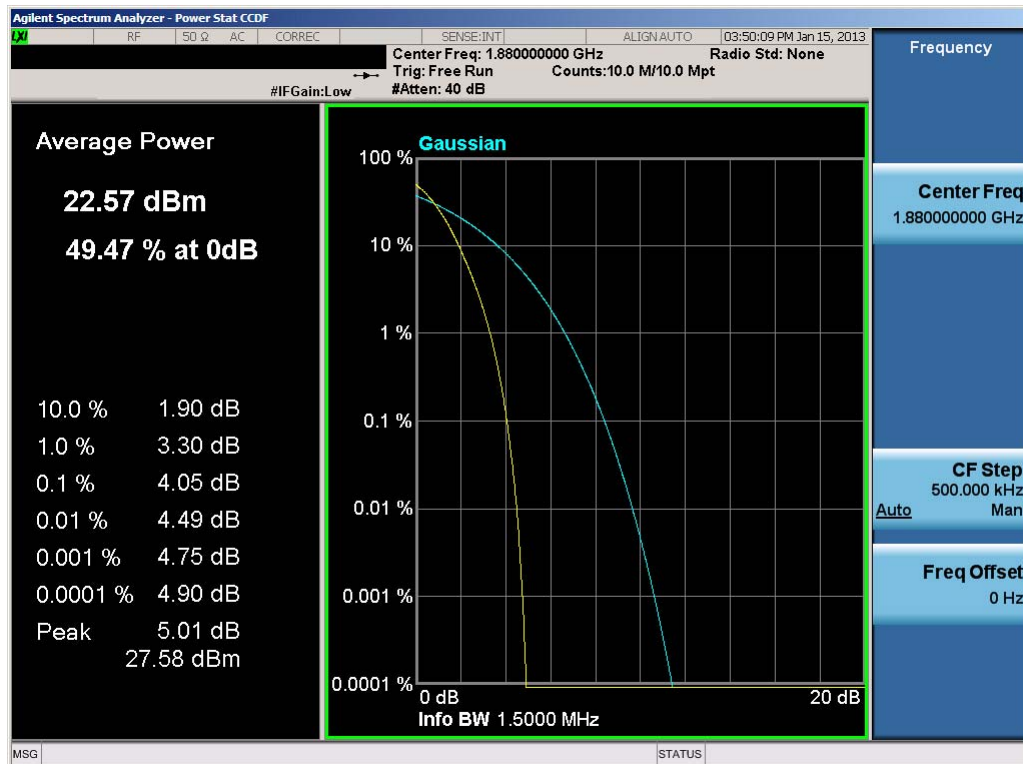
Plot 7-47. Peak-Average Ratio Plot (PCS CDMA Mode – Ch. 600)
