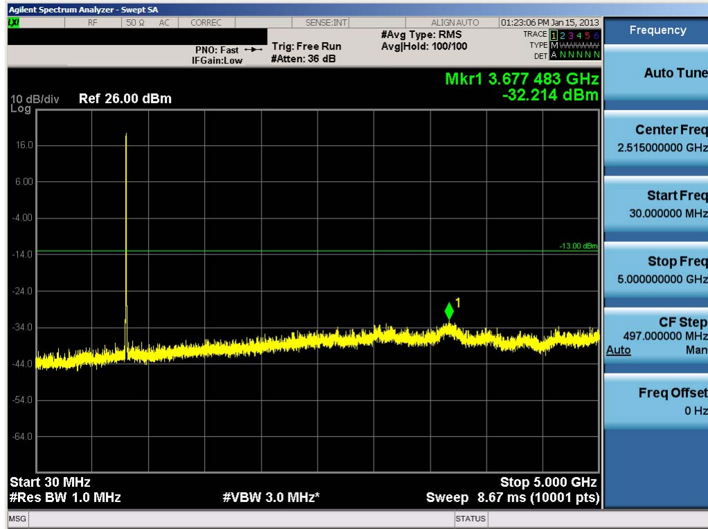
Plot 7-52. Conducted Spurious Plot (Cellular WCDMA Mode – Ch. 4132)
