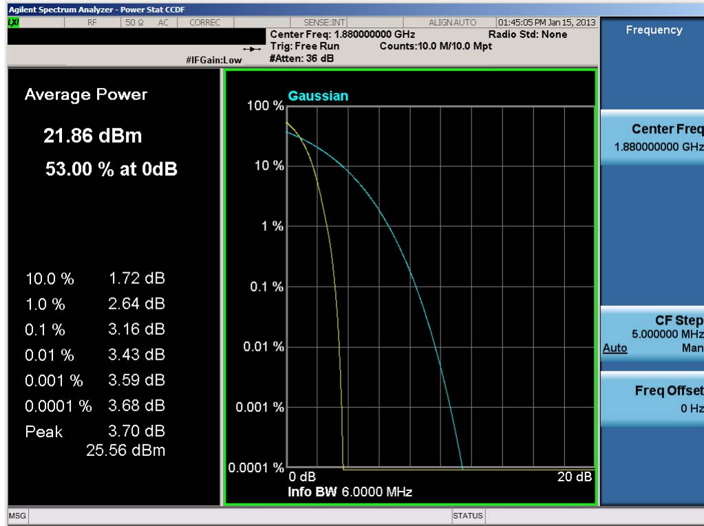
Plot 7-70. Peak-Average Ratio Plot (PCS WCDMA Mode – Ch. 9400)
