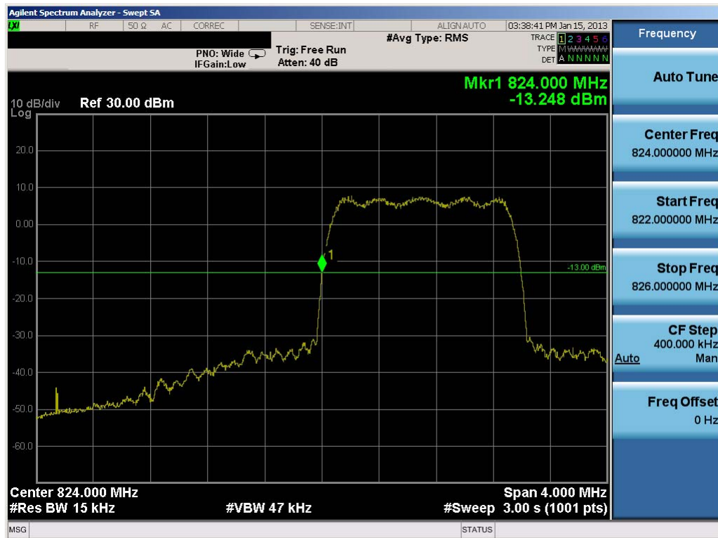
Plot 7-31. Band Edge Plot (Cellular CDMA Mode – Ch. 1013)
