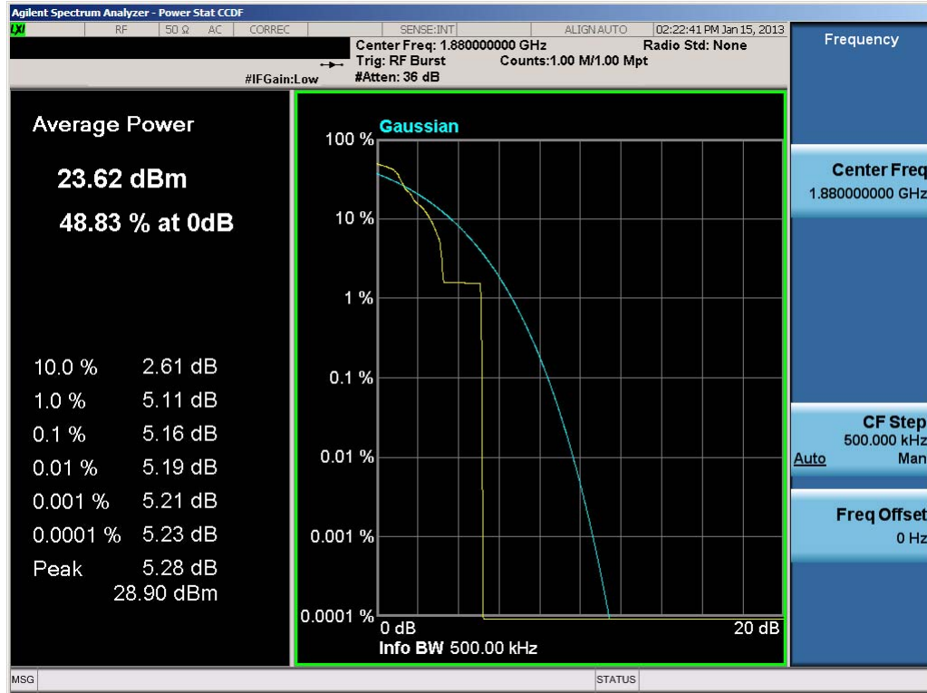
Plot 7-28. Peak-Average Ratio Plot (EDGE1900 Mode – Ch. 661)
