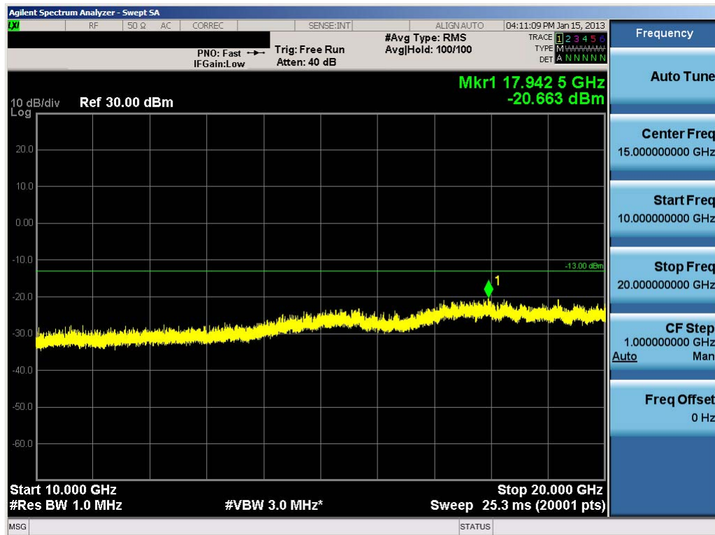
Plot 7-41. Conducted Spurious Plot (PCS CDMA Mode – Ch. 25)
