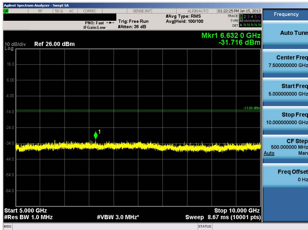
Plot 7-57. Conducted Spurious Plot (Cellular WCDMA Mode – Ch. 4183)
