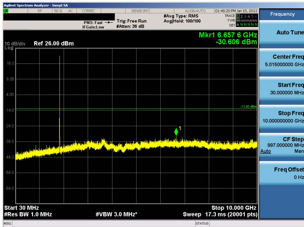
Plot 7-63. Conducted Spurious Plot (PCS WCDMA Mode – Ch. 9262)
