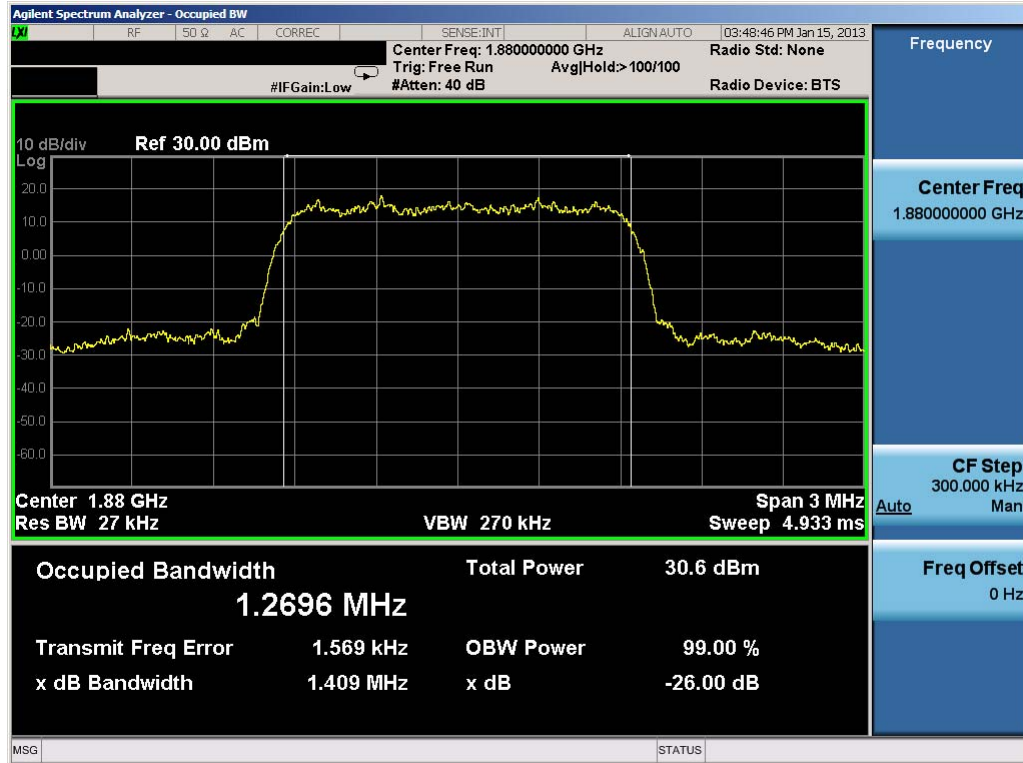
Plot 7-46. Occupied Bandwidth Plot (PCS CDMA Mode – Ch. 600)
