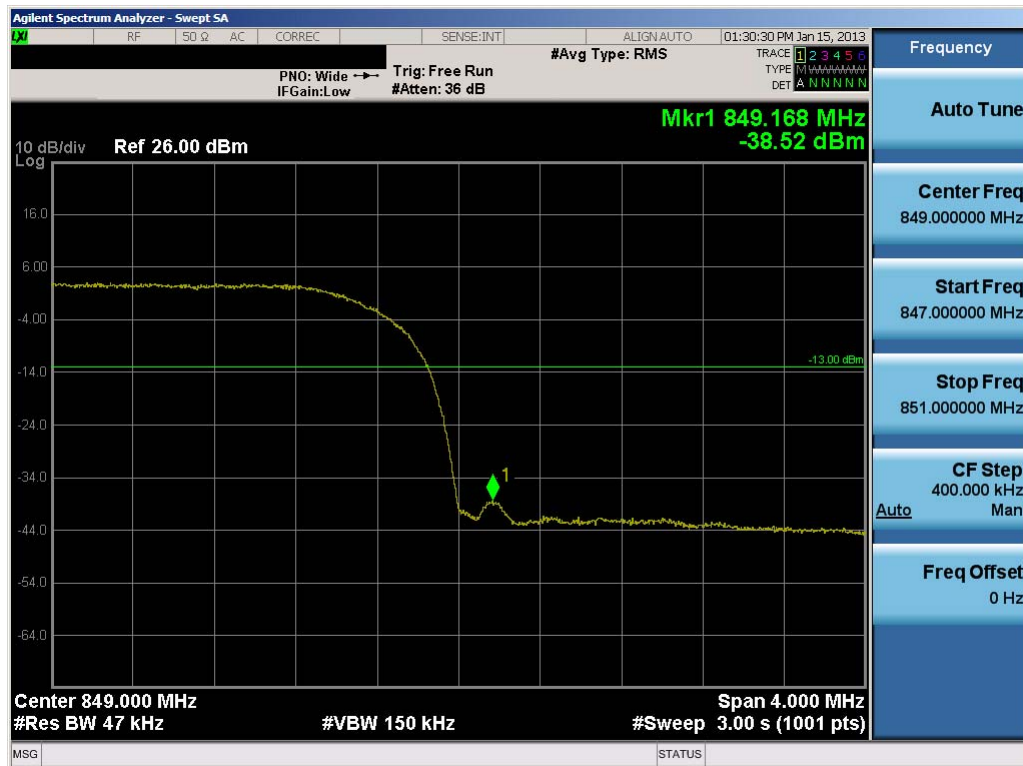
Plot 7-61. Band Edge Plot (Cellular WCDMA Mode – Ch. 4233)
