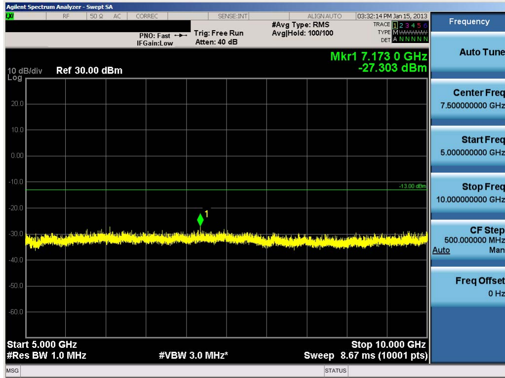
Plot 7-34. Conducted Spurious Plot (Cellular CDMA Mode – Ch. 384)
