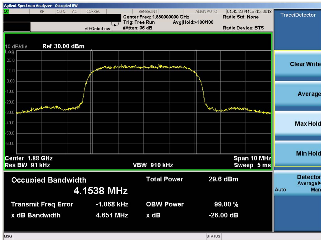
Plot 7-69. Occupied Bandwidth Plot (PCS WCDMA Mode – Ch. 9400)
