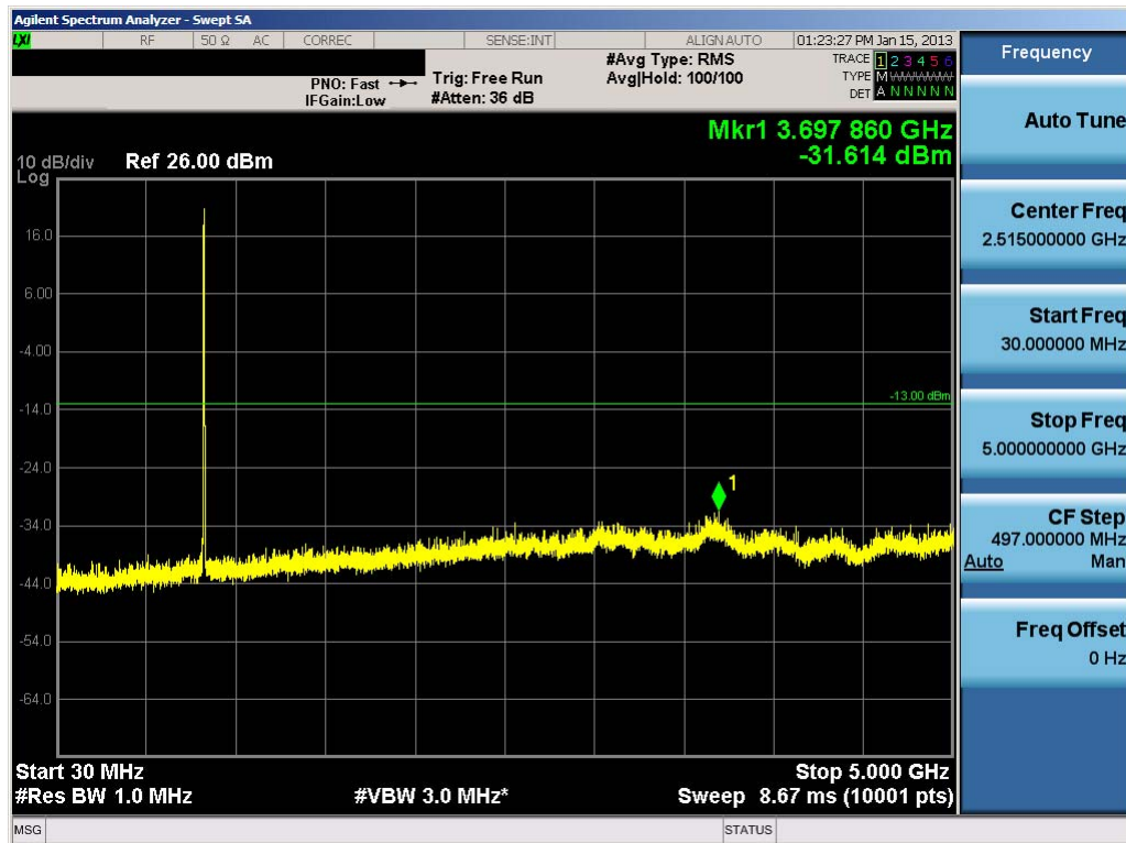
Plot 7-59. Conducted Spurious Plot (Cellular WCDMA Mode – Ch. 4233)
