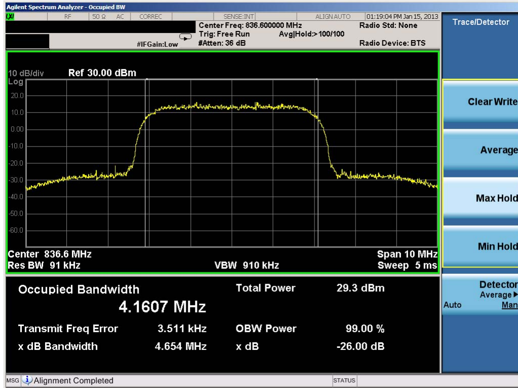
Plot 7-58. Occupied Bandwidth Plot (Cellular WCDMA Mode – Ch. 4183)
