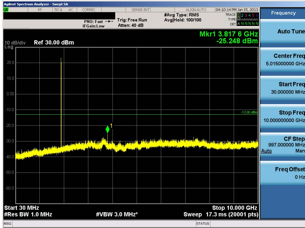
Plot 7-48. Conducted Spurious Plot (PCS CDMA Mode – Ch. 1175)
