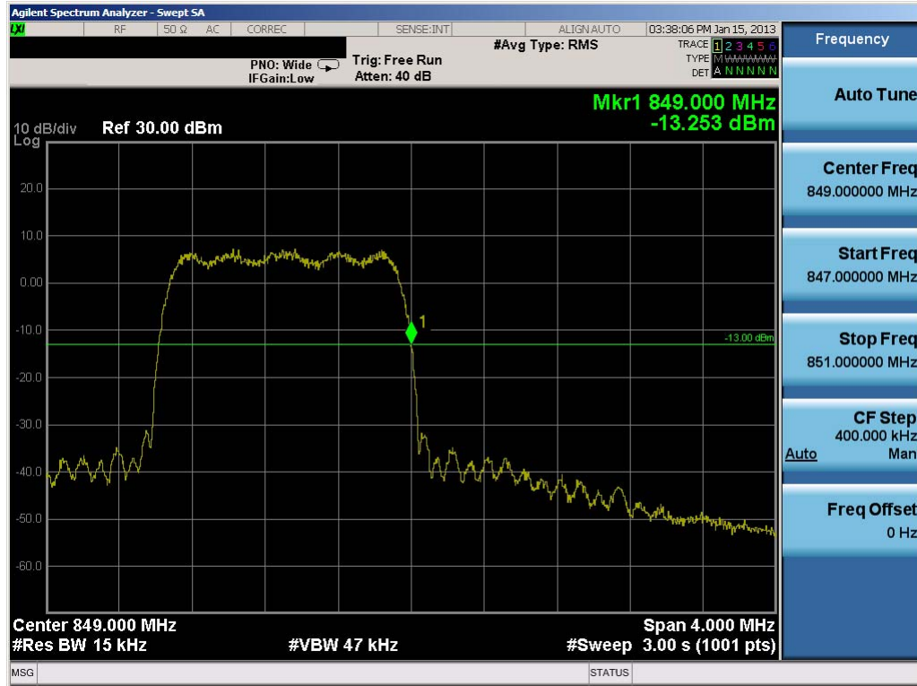
Plot 7-38. Band Edge Plot (Cellular CDMA Mode – Ch. 777)
