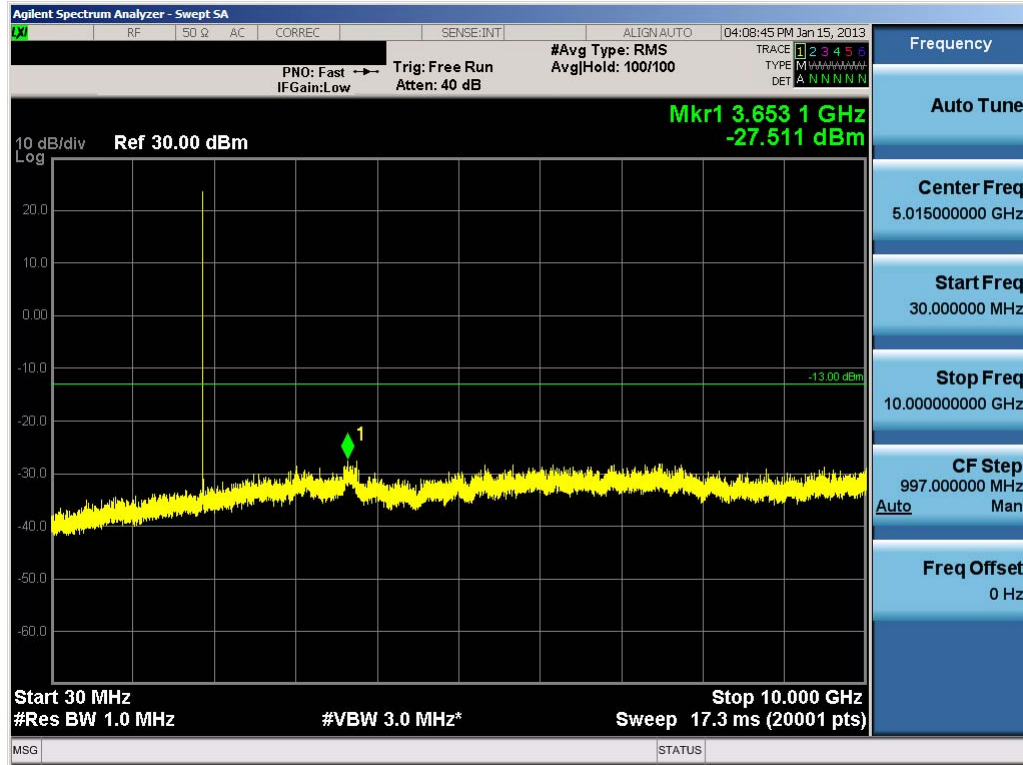
Plot 7-44. Conducted Spurious Plot (PCS CDMA Mode – Ch. 600)
