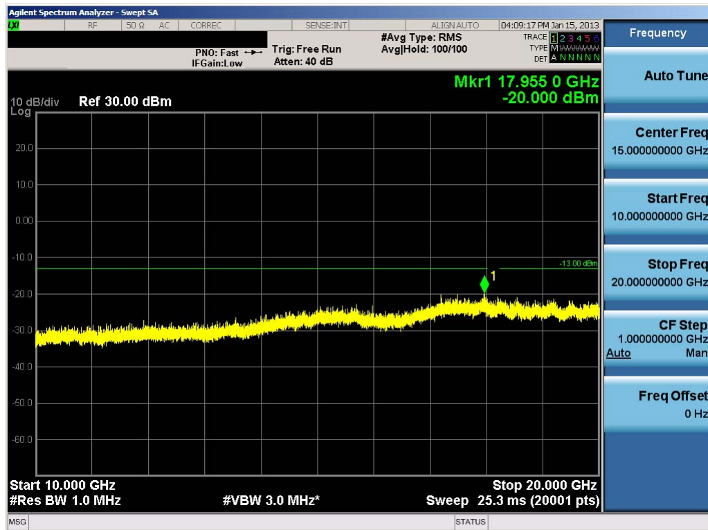
Plot 7-45. Conducted Spurious Plot (PCS CDMA Mode – Ch. 600)
