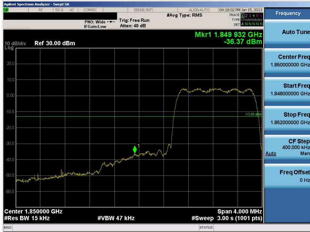
Plot 7-42. Band Edge Plot (PCS CDMA Mode – Ch. 25)
