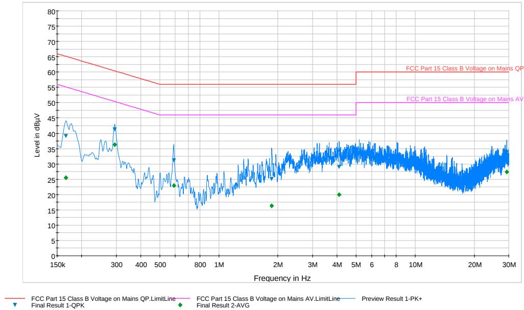
Plot 6-58. Line Conducted Plot with 802.11a UNII Band 3 (L1)
