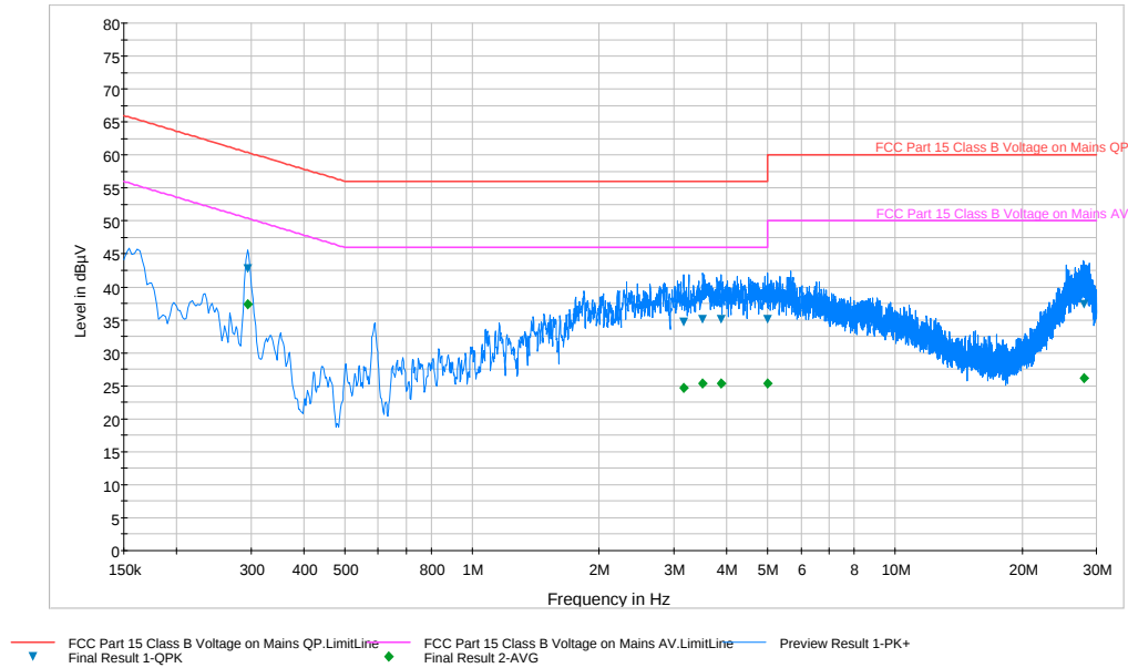
Plot 6-55. Line Conducted Plot with 802.11a UNII Band 1 (N)
