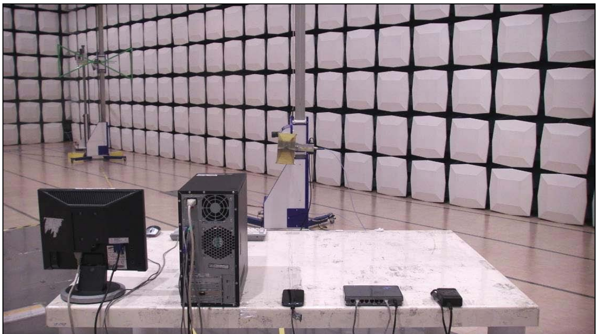
[ Radiated Disturbance for Above 1 GHz – Rear ]
