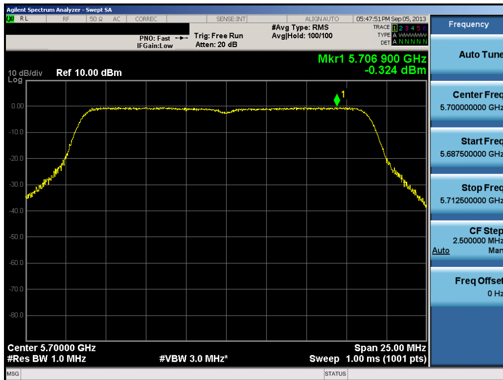
Plot 6-50. Peak Power Spectral Density Plot (20MHz BW 802.11a/n (UNII Band 3) – Ch. 140)
