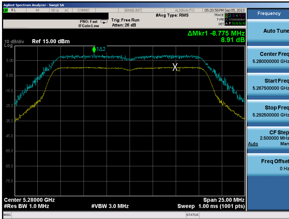
Plot 6-54. Peak Excursion Ratio Plot (802.11a)
