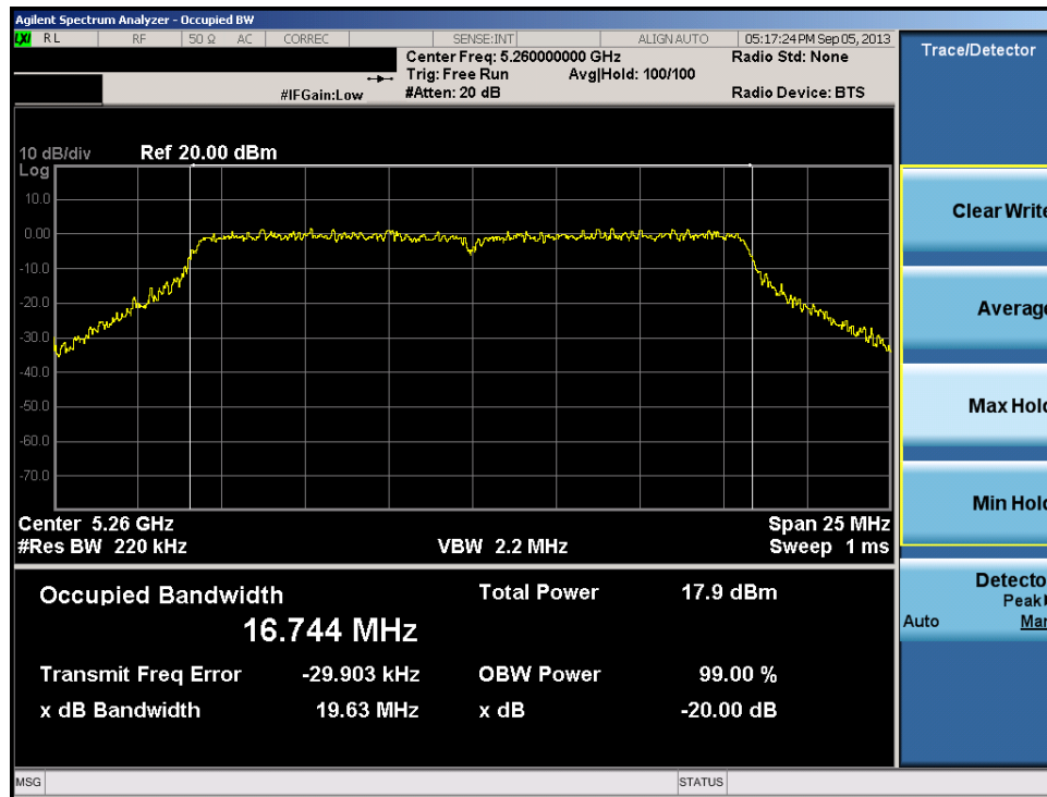
Plot 6-26. 20dB Bandwidth Plot (20MHz BW 802.11a (UNII Band 2) – Ch. 52)
