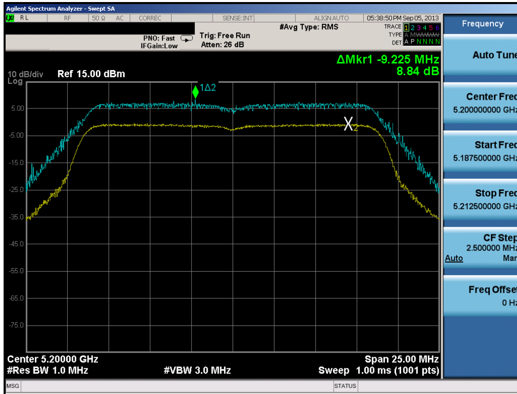
Plot 6-55. Peak Excursion Ratio Plot (20MHz BW 802.11n)
