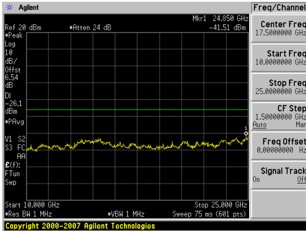
Plot 6-42. Conducted Spurious Plot (802.11g – Ch. 1)
