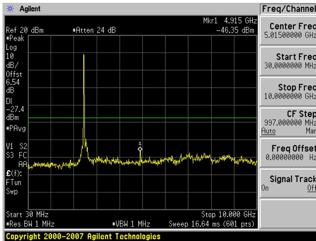
Plot 6-41. Conducted Spurious Plot (802.11g – Ch. 1)
