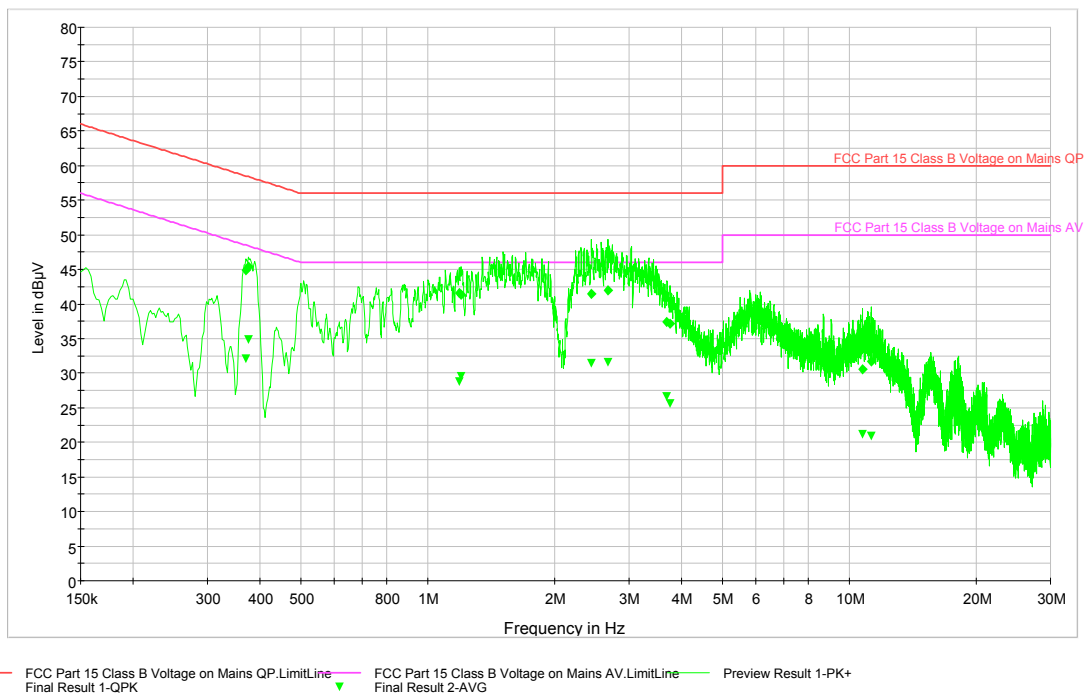
Plot 6-16. Line Conducted Plot with Bluetooth LE (N)
