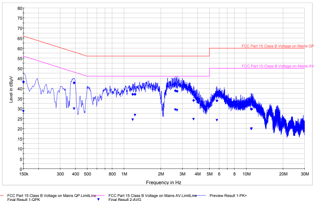
Plot 6-15. Line Conducted Plot with Bluetooth LE (L1)
