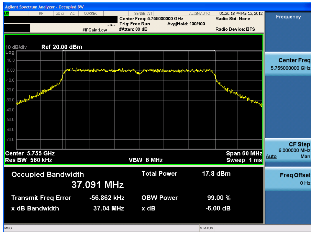
Plot 6-16. 6dB Bandwidth Plot (802.11n (5.8GHz – 40MHz BW) – Ch. 151)
