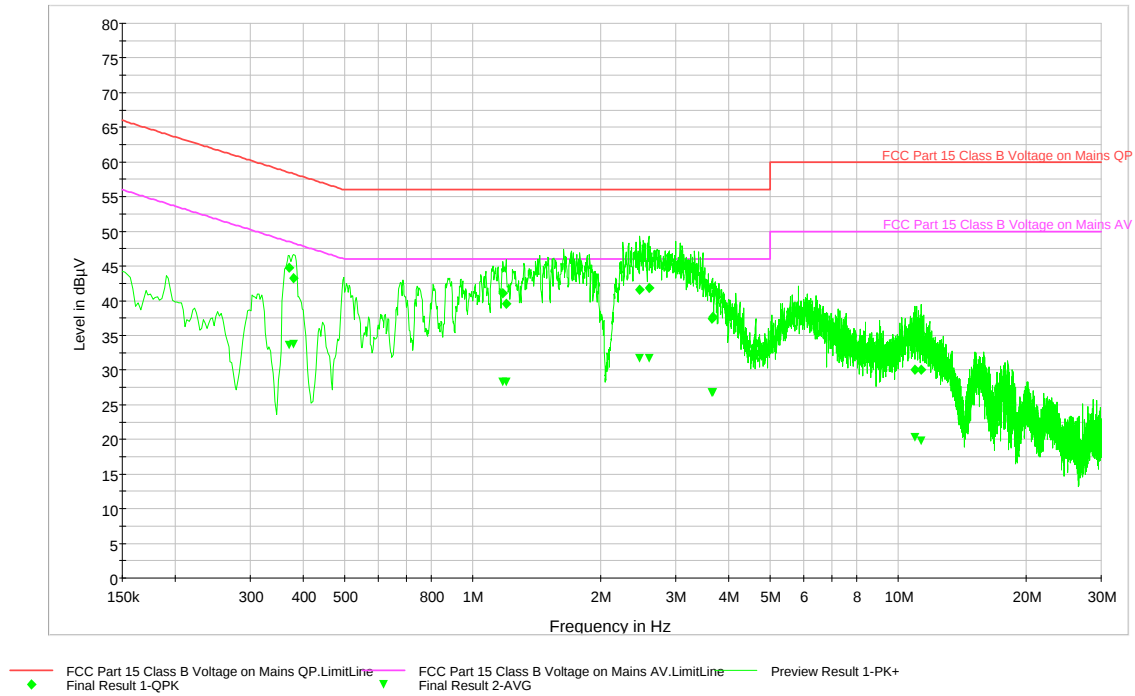
Plot 6-63. Line Conducted Data with 802.11b (LN)
