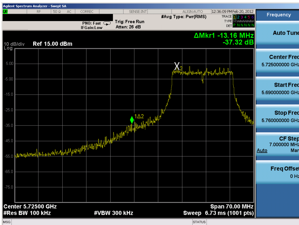
Plot 6-43. Band Edge Plot (802.11n (5.8GHz – 20MHz BW) – Ch. 149)
