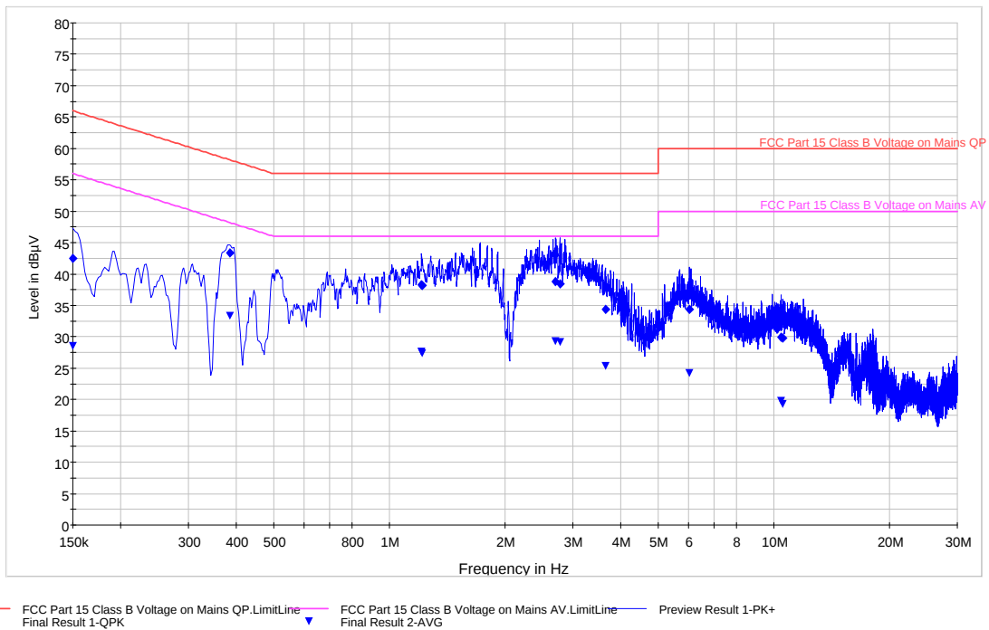
Plot 6-62. Line Conducted Plot with 802.11b (L1)
