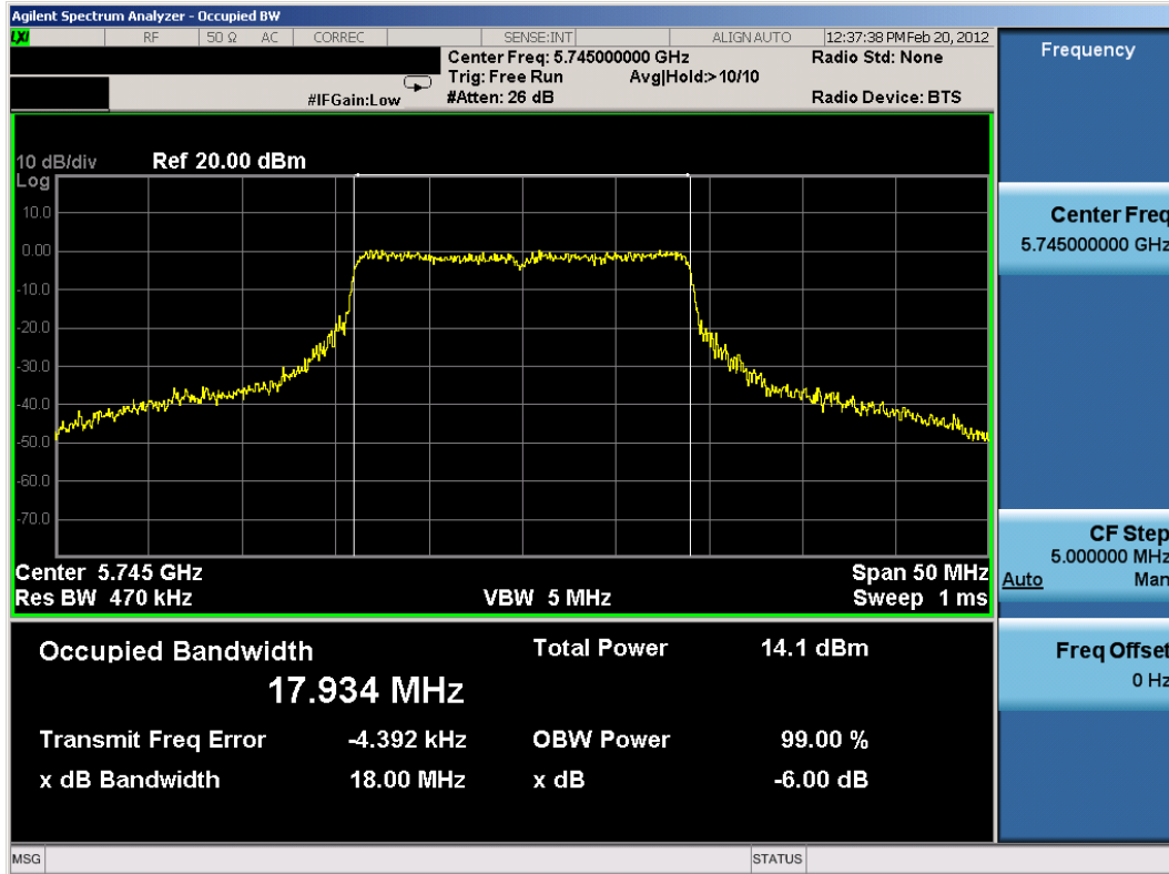
Plot 6-13. 6dB Bandwidth Plot (802.11n (5.8GHz – 20MHz BW) – Ch. 149)
