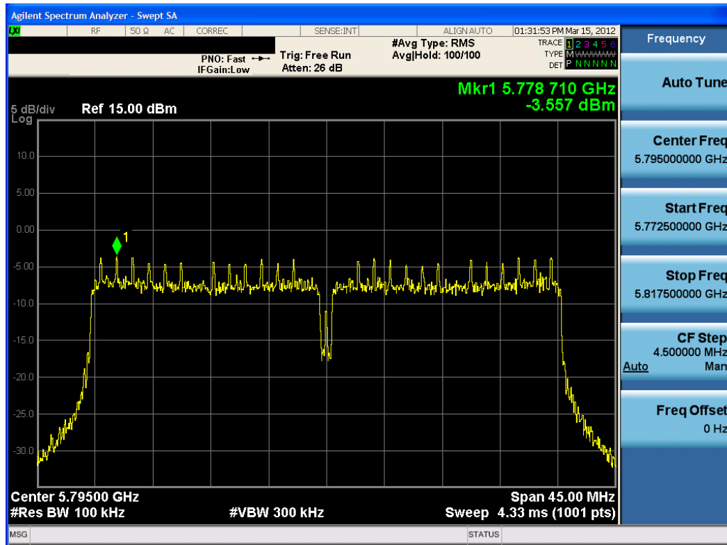
Plot 6-34. Power Spectral Density Plot (802.11n (5.8GHz – 40MHz BW) – Ch. 159)
