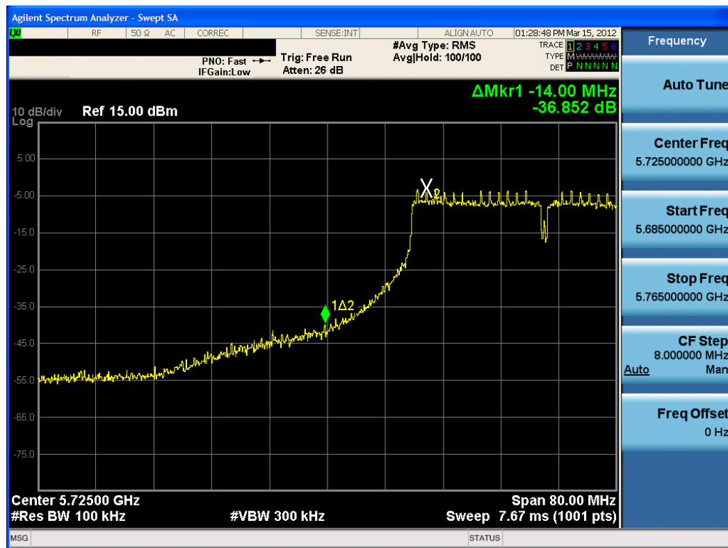
Plot 6-45. Band Edge Plot (802.11n (5.8GHz – 40MHz BW) – Ch. 151)
