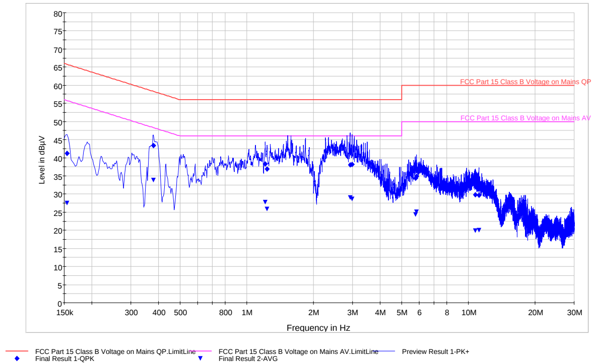
Plot 6-64. Line Conducted Plot with 802.11a (L1)
