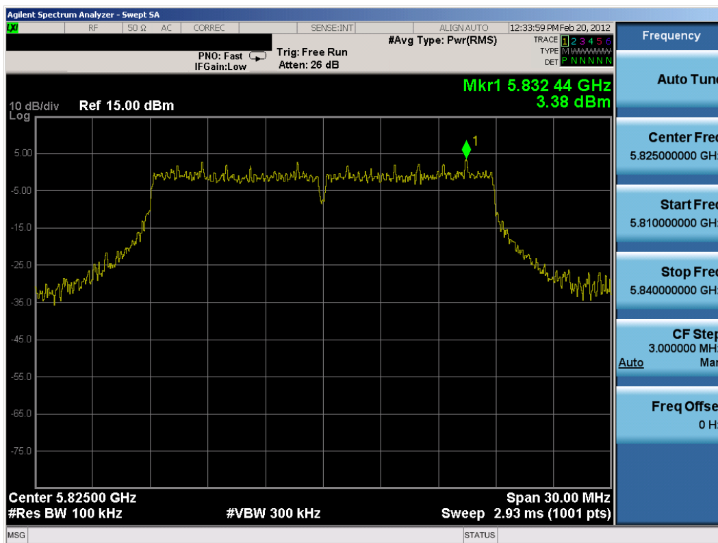
Plot 6-32. Power Spectral Density Plot (802.11n (5.8GHz – 20MHz BW) – Ch. 165)
