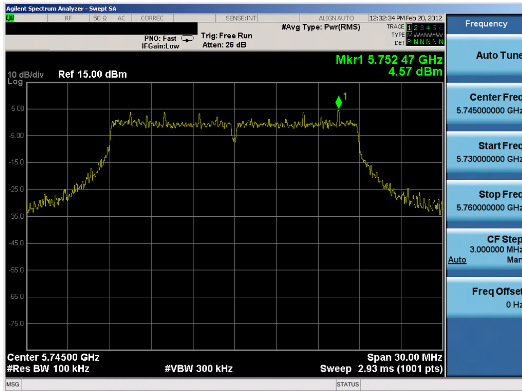
Plot 6-30. Power Spectral Density Plot (802.11n (5.8GHz – 20MHz BW) – Ch. 149)
