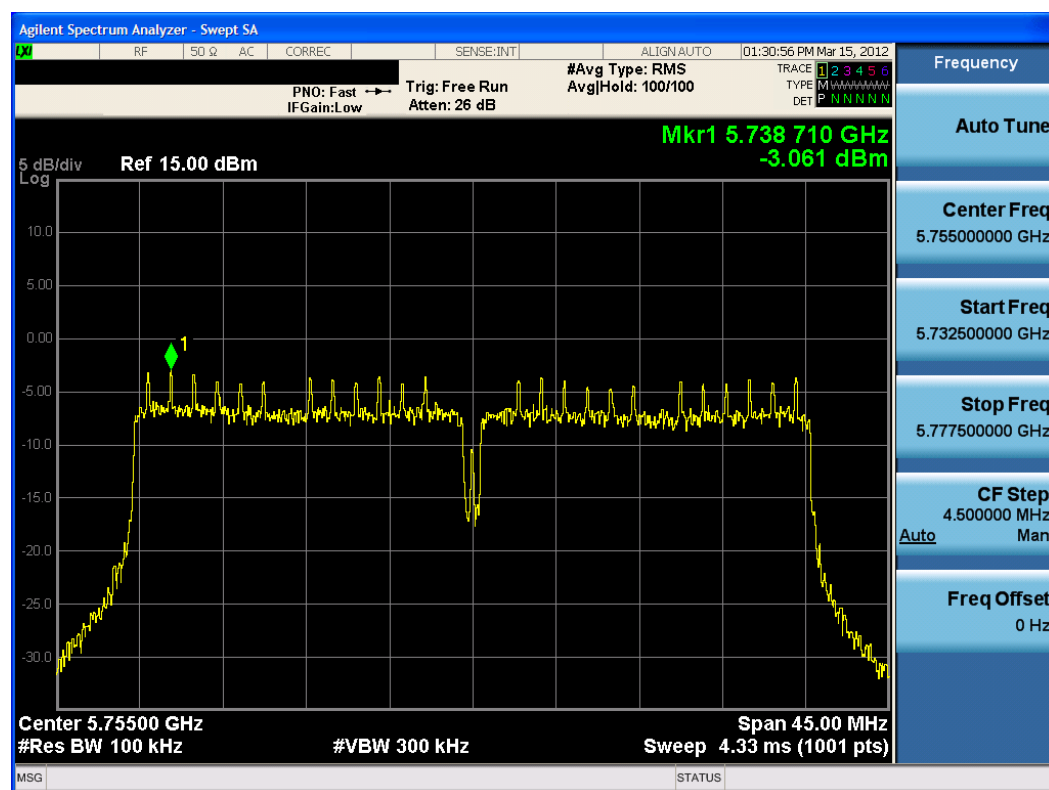
Plot 6-33. Power Spectral Density Plot (802.11n (5.8GHz – 40MHz BW) – Ch. 151)
