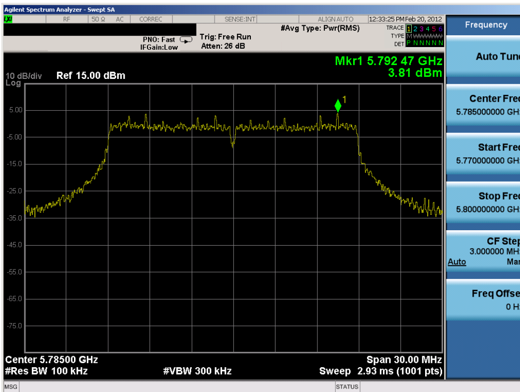
Plot 6-31. Power Spectral Density Plot (802.11n (5.8GHz – 20MHz BW) – Ch. 157)
