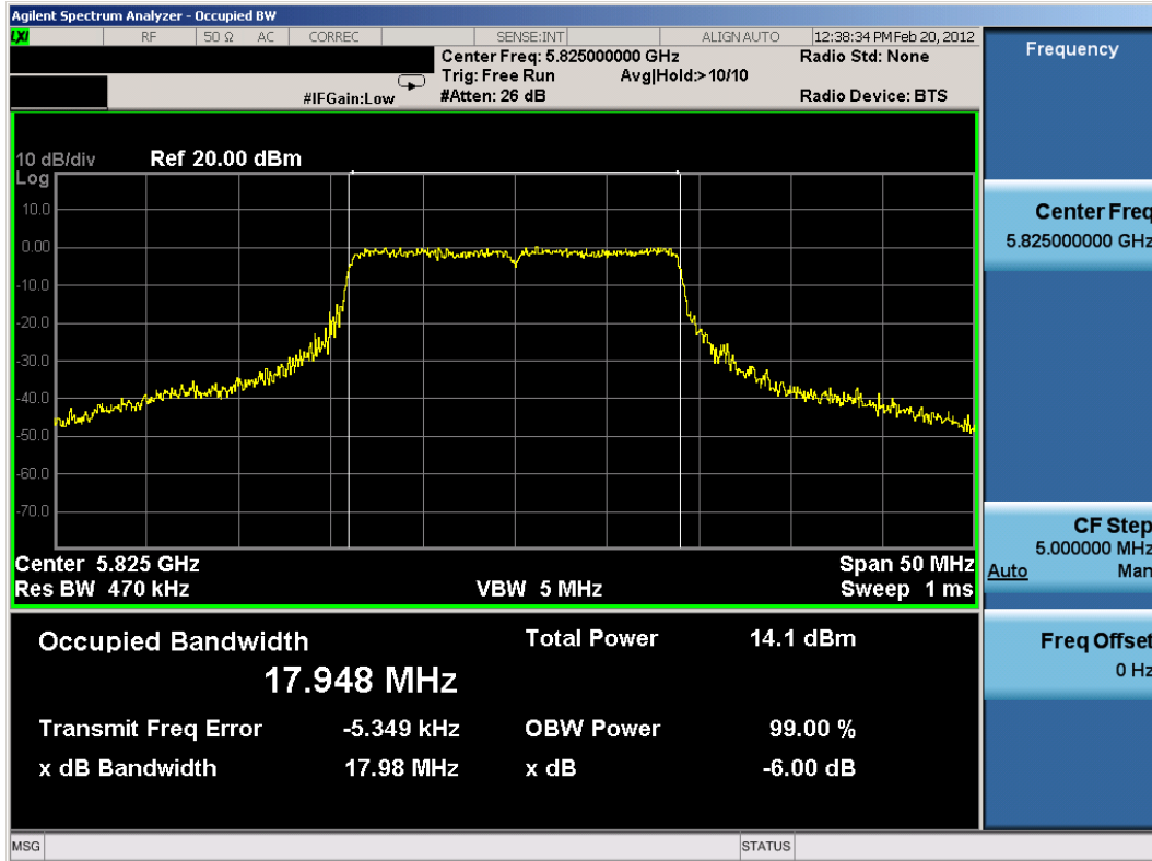
Plot 6-15. 6dB Bandwidth Plot (802.11n (5.8GHz – 20MHz BW) – Ch. 165)
