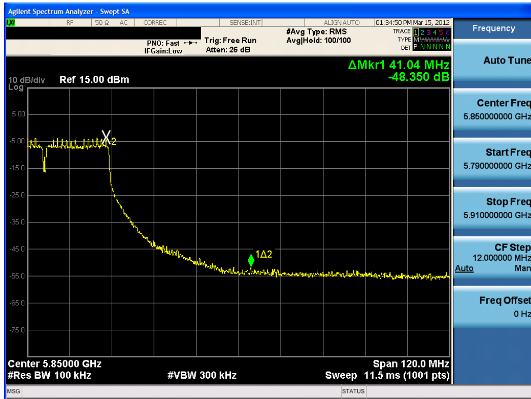
Plot 6-46. Band Edge Plot (802.11n (5.8GHz – 40MHz BW) – Ch. 159)
