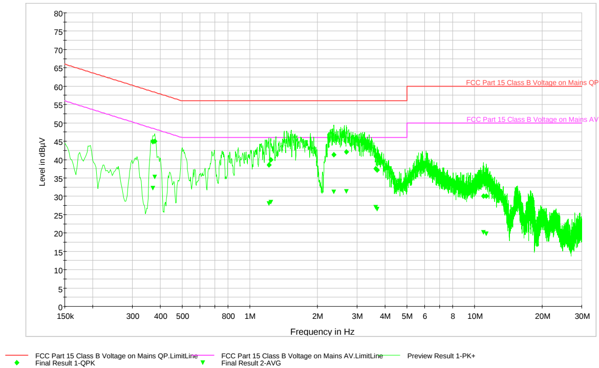
Plot 6-65. Line Conducted Data with 802.11a (LN)
