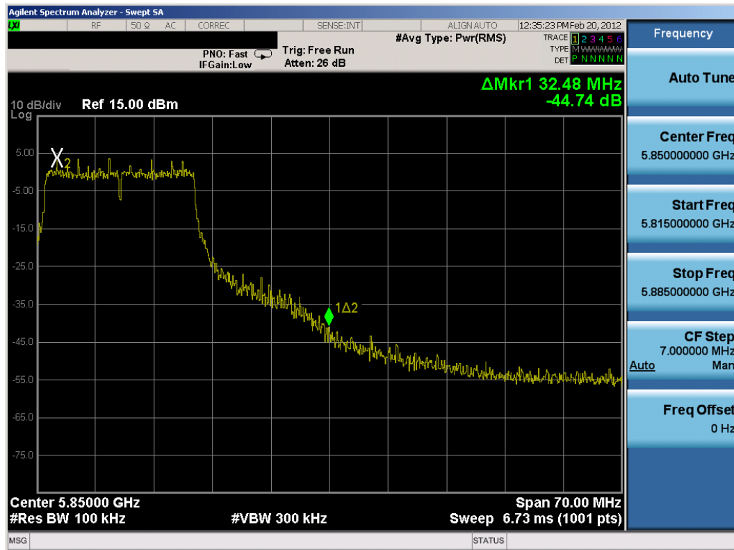
Plot 6-44. Band Edge Plot (802.11n (5.8GHz – 20MHz BW) – Ch. 165)
