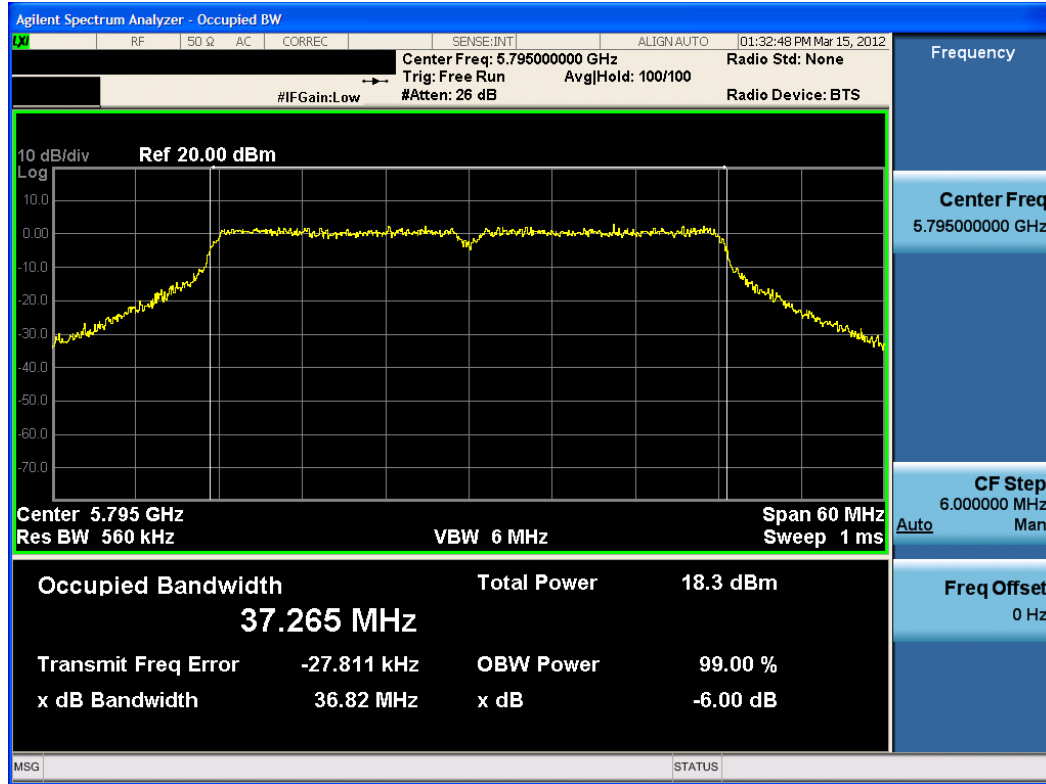
Plot 6-17. 6dB Bandwidth Plot (802.11n (5.8GHz – 40MHz BW) – Ch. 159)
