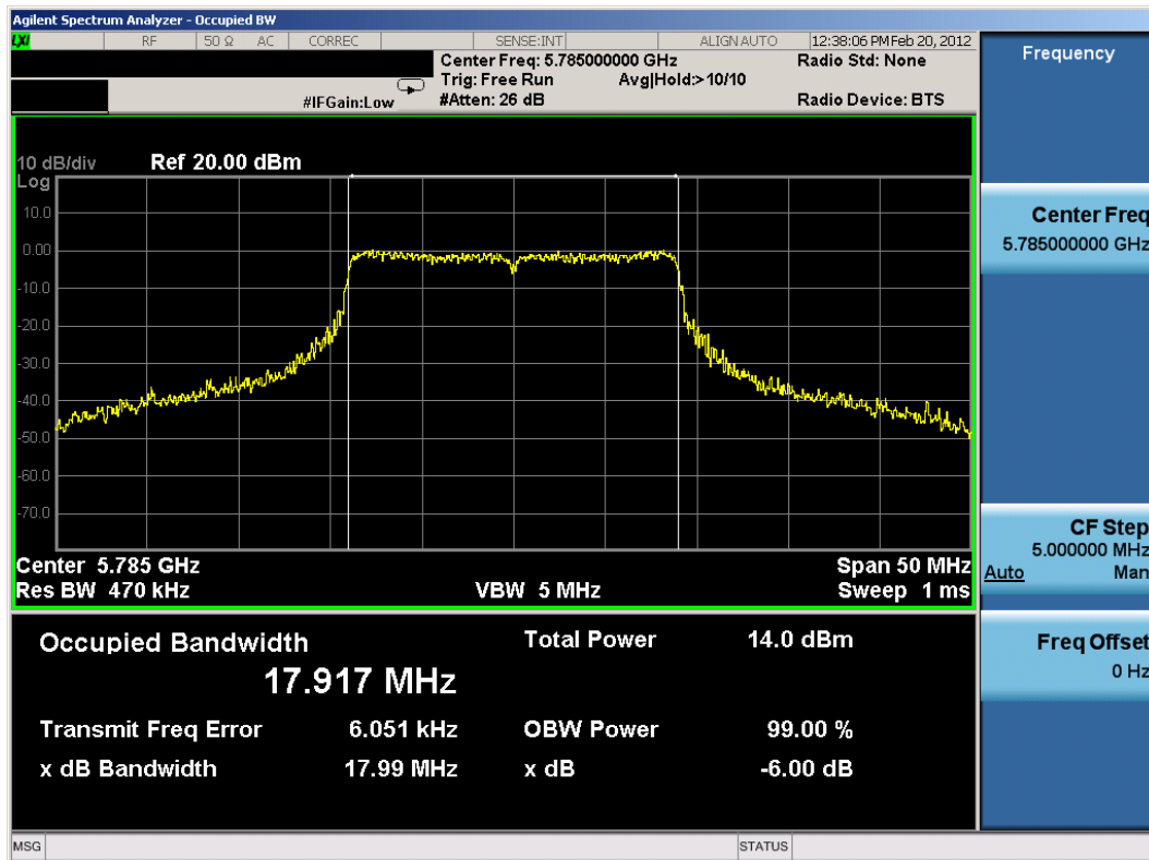
Plot 6-14. 6dB Bandwidth Plot (802.11n (5.8GHz – 20MHz BW) – Ch. 157)
