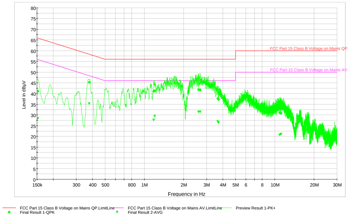
Plot 6-78. Line Conducted Plot with 802.11a (UNII Band 1) (LN)
