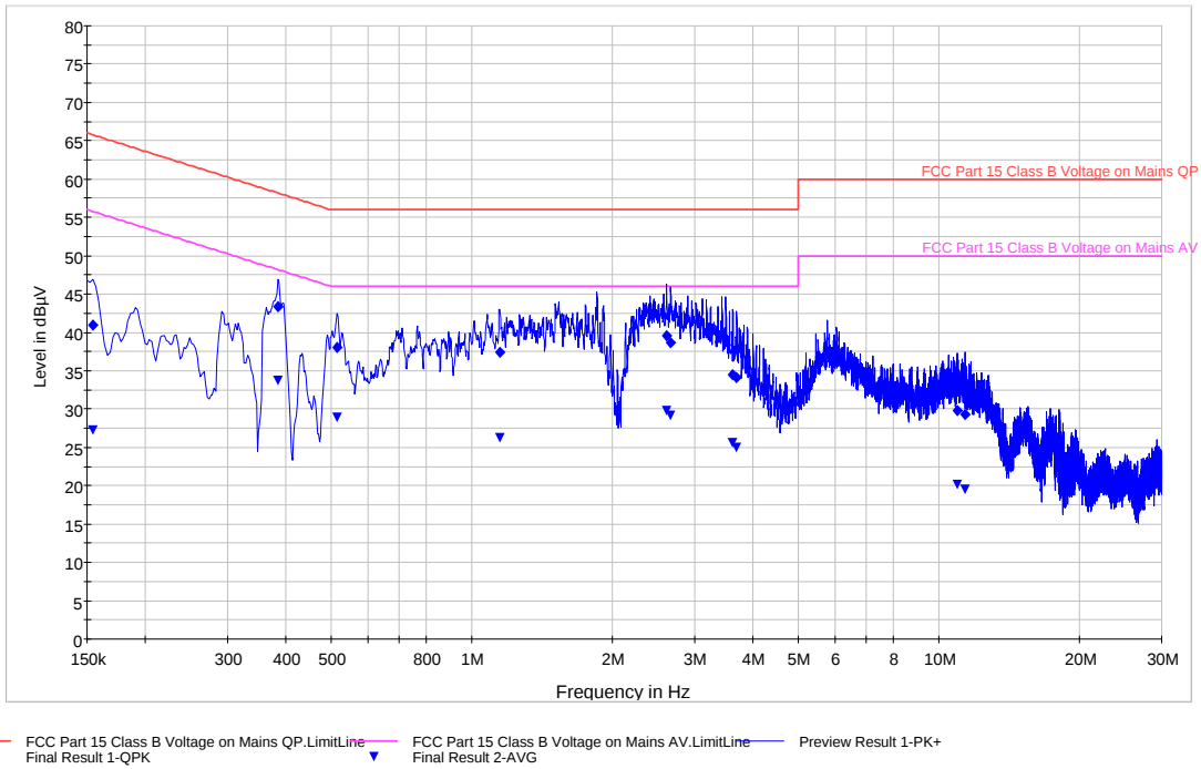
Plot 6-77. Line Conducted Plot with 802.11a (UNII Band 1) (L1)
