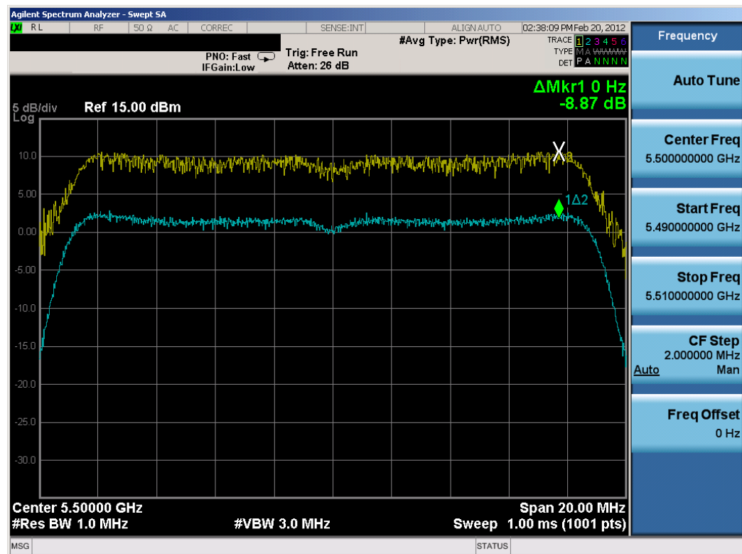
Plot 6-71. Peak Excursion Ratio Plot (802.11n – 20MHz BW (UNII Band 3) – Ch. 100)
