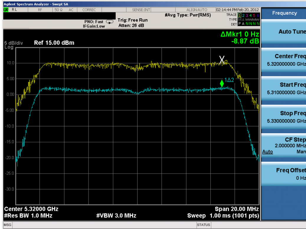
Plot 6-62. Peak Excursion Ratio Plot (802.11a (UNII Band 2) – Ch. 64)
