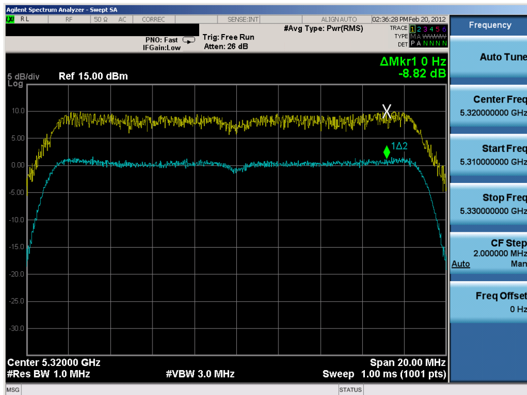
Plot 6-65. Peak Excursion Ratio Plot (802.11n – 20MHz BW (UNII Band 2) – Ch. 64)
