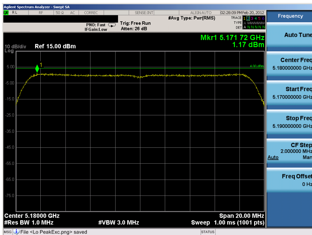
Plot 6-30. Peak Power Spectral Density Plot (802.11n – 20MHz BW (UNII Band 1) – Ch. 36)
