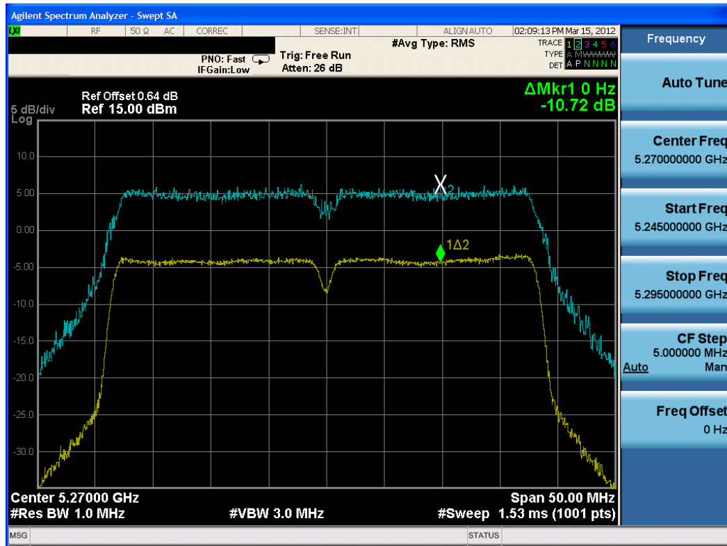
Plot 6-66. Peak Excursion Ratio Plot (802.11n – 40MHz BW (UNII Band 2) – Ch. 54)
