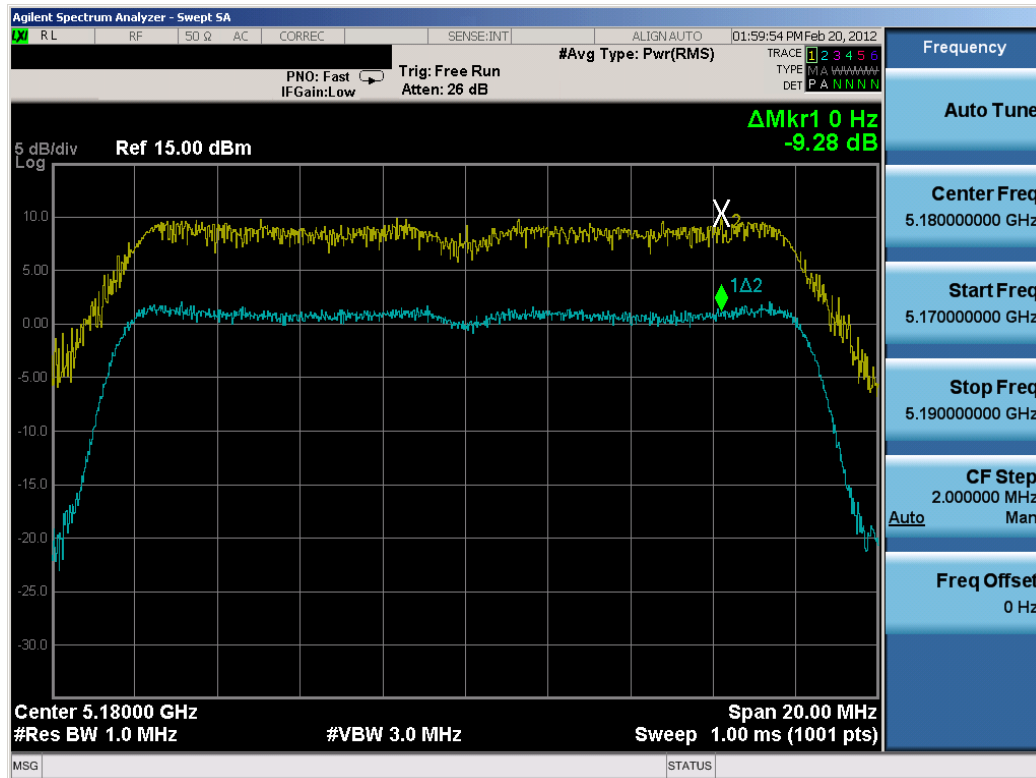
Plot 6-52. Peak Excursion Ratio Plot (802.11a (UNII Band 1) – Ch. 36)
