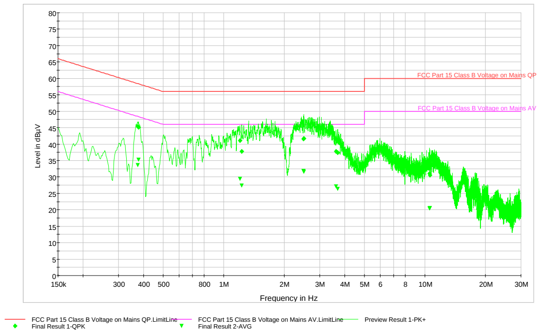
Plot 6-82. Line Conducted Data with 802.11a (UNII Band 3) (LN)
