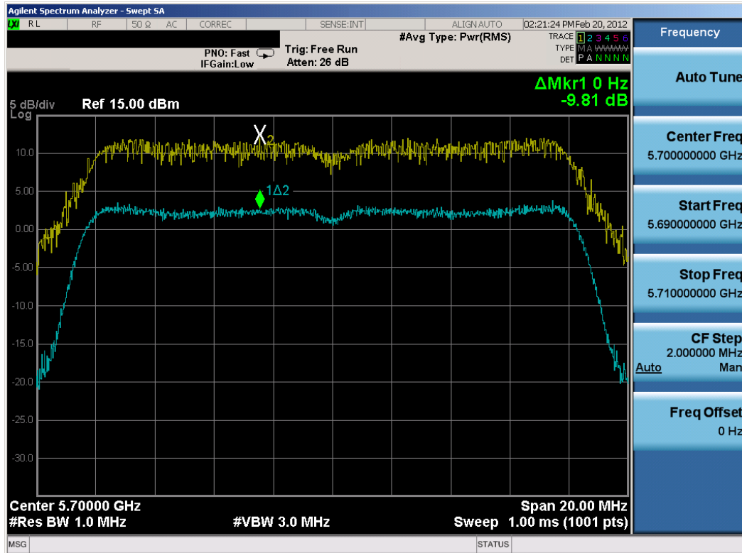
Plot 6-70. Peak Excursion Ratio Plot (802.11a (UNII Band 3) – Ch. 140)
