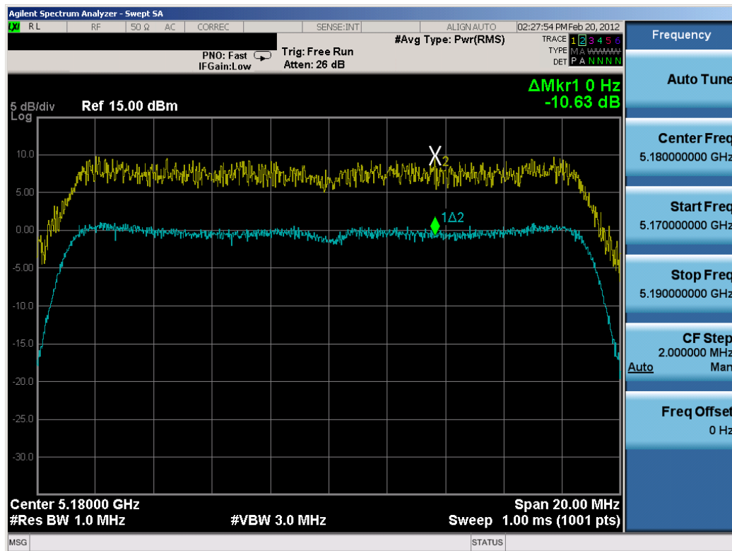
Plot 6-55. Peak Excursion Ratio Plot (802.11n - 20MHz BW (UNII Band 1) – Ch. 36)
