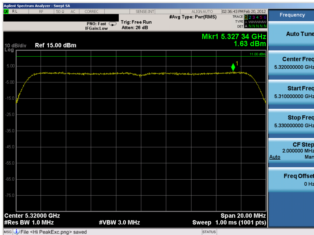
Plot 6-40. Peak Power Spectral Density Plot (802.11n – 20MHz BW (UNII Band 2) – Ch. 64)
