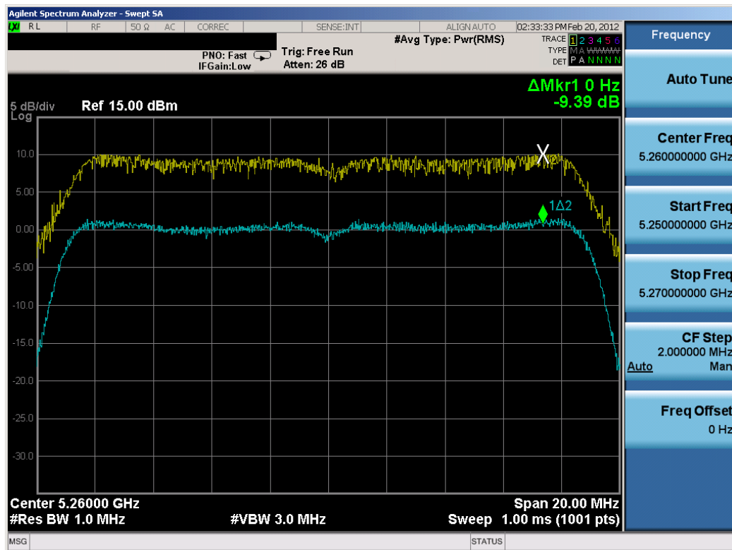
Plot 6-63. Peak Excursion Ratio Plot (802.11n – 20MHz BW (UNII Band 2) – Ch. 52)
