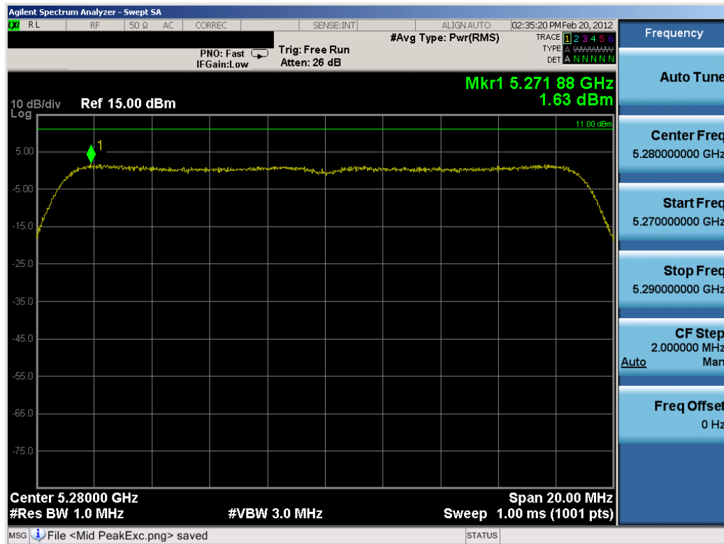
Plot 6-39. Peak Power Spectral Density Plot (802.11n – 20MHz BW (UNII Band 2) – Ch. 56)
