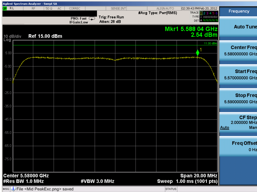
Plot 6-47. Peak Power Spectral Density Plot (802.11n – 20MHz BW (UNII Band 3) – Ch. 116)
