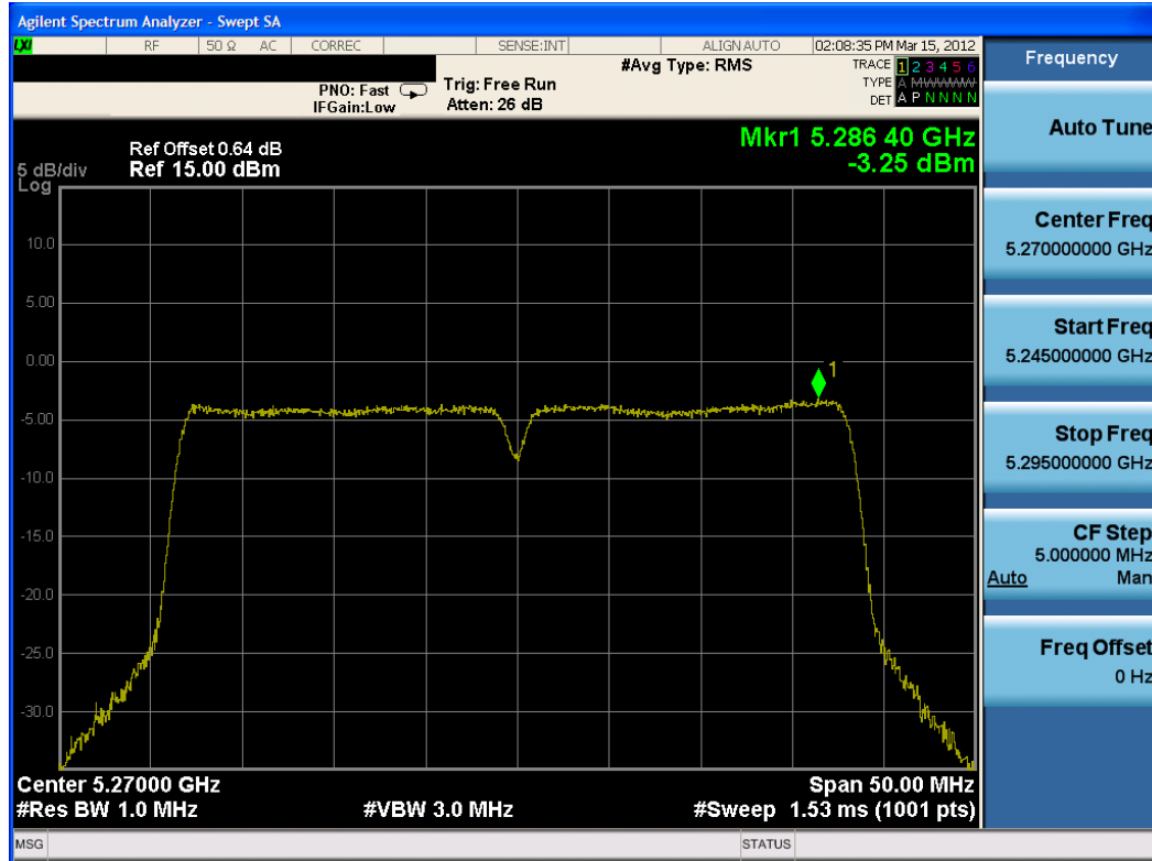
Plot 6-41. Peak Power Spectral Density Plot (802.11n – 40MHz BW (UNII Band 2) – Ch. 54)
