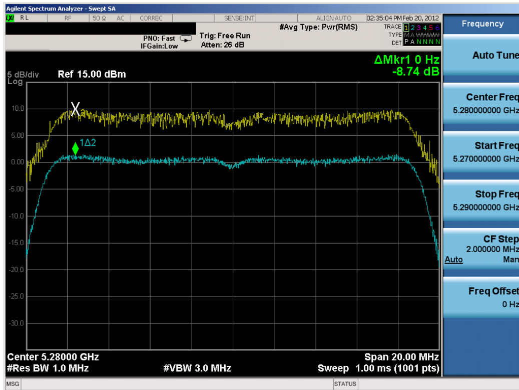
Plot 6-64. Peak Excursion Ratio Plot (802.11n – 20MHz BW (UNII Band 2) – Ch. 56)
