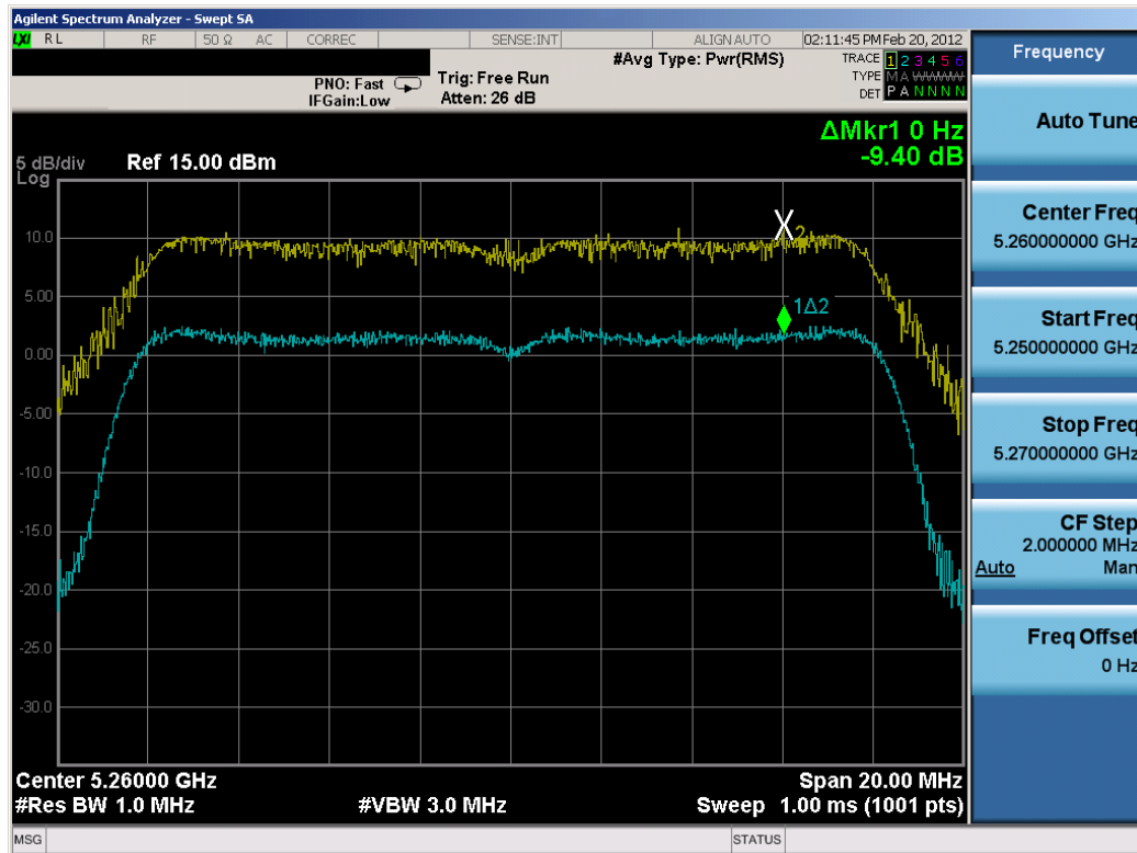
Plot 6-60. Peak Excursion Ratio Plot (802.11a (UNII Band 2) – Ch. 52)
