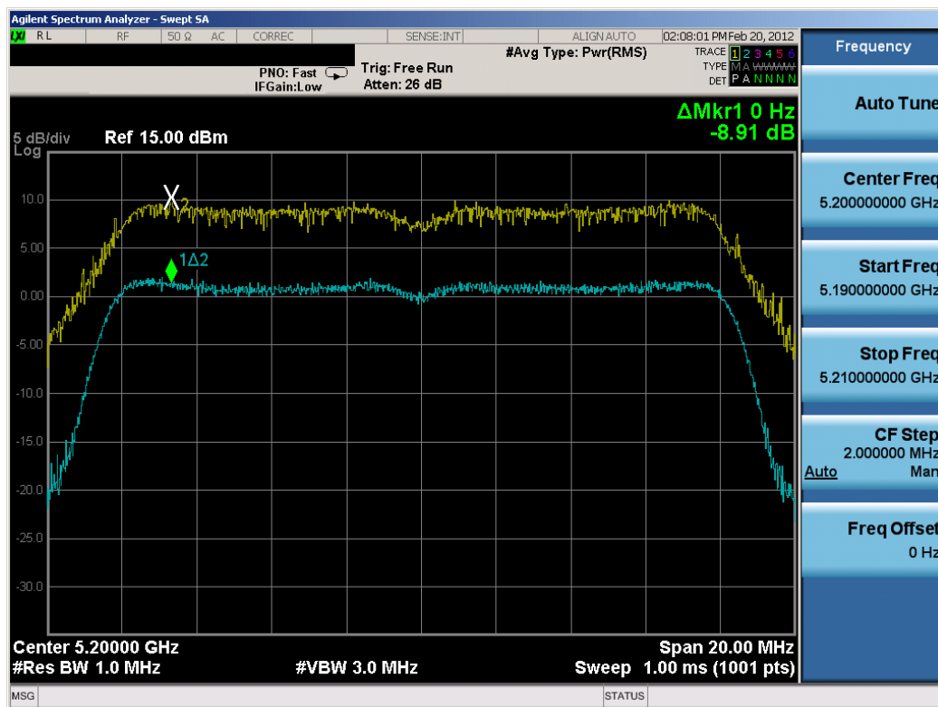
Plot 6-53. Peak Excursion Ratio Plot (802.11a (UNII Band 1) – Ch. 40)
