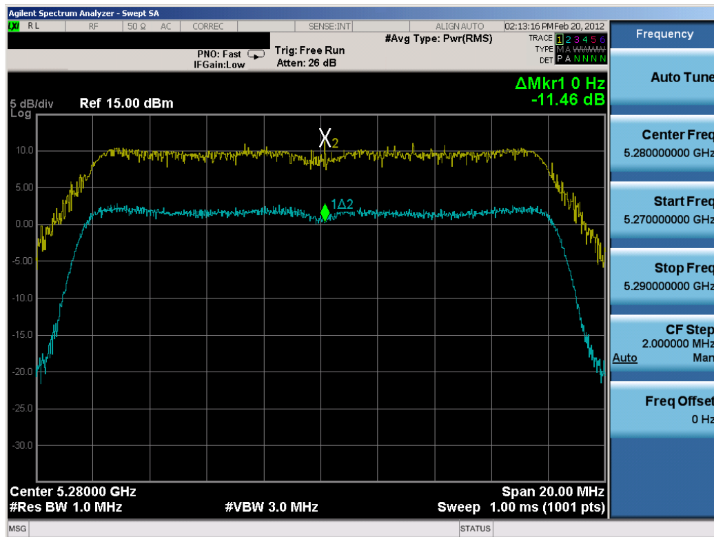
Plot 6-61. Peak Excursion Ratio Plot (802.11a (UNII Band 2) – Ch. 56)
