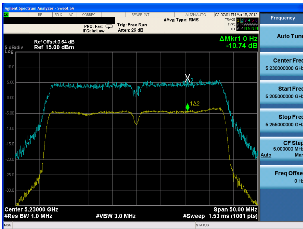
Plot 6-59. Peak Excursion Ratio Plot (802.11n – 40MHz BW (UNII Band 1) – Ch. 46)
