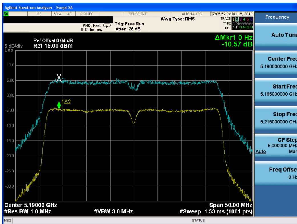
Plot 6-58. Peak Excursion Ratio Plot (802.11n – 40MHz BW (UNII Band 1) – Ch. 38)
