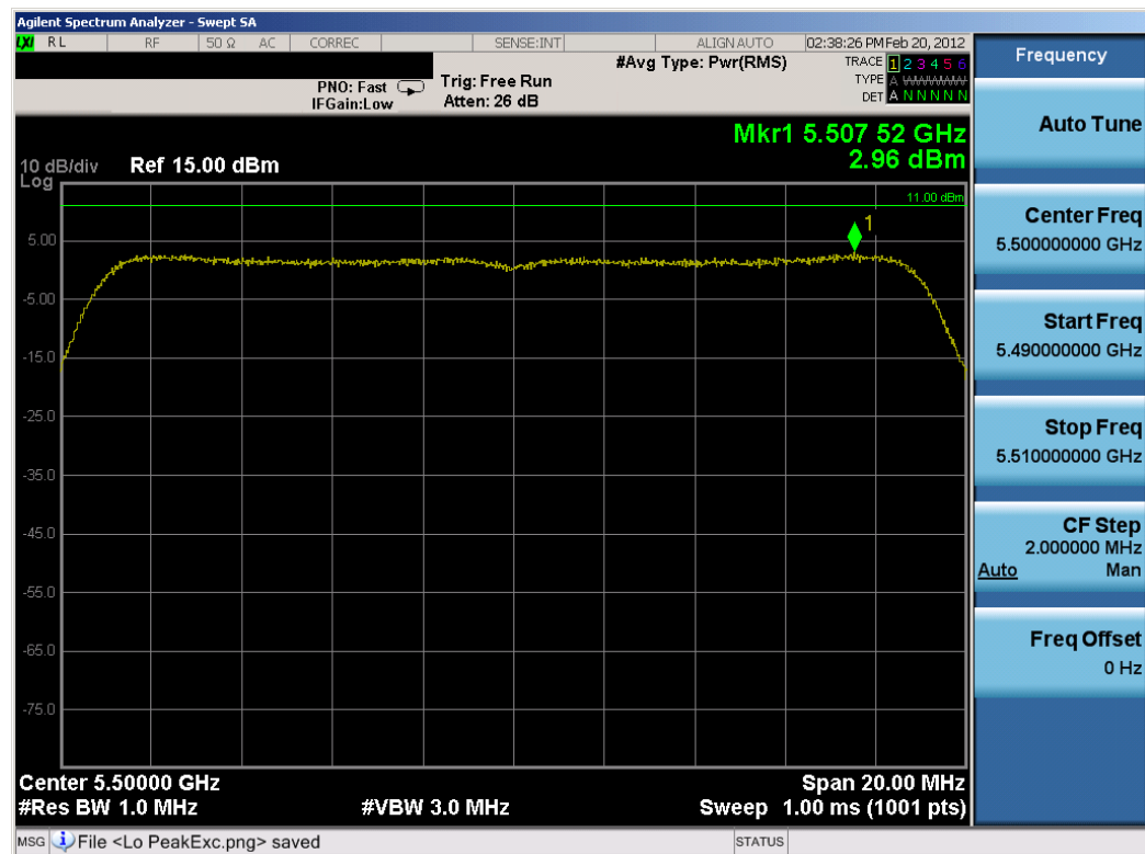
Plot 6-46. Peak Power Spectral Density Plot (802.11n – 20MHz BW (UNII Band 3) – Ch. 100)
