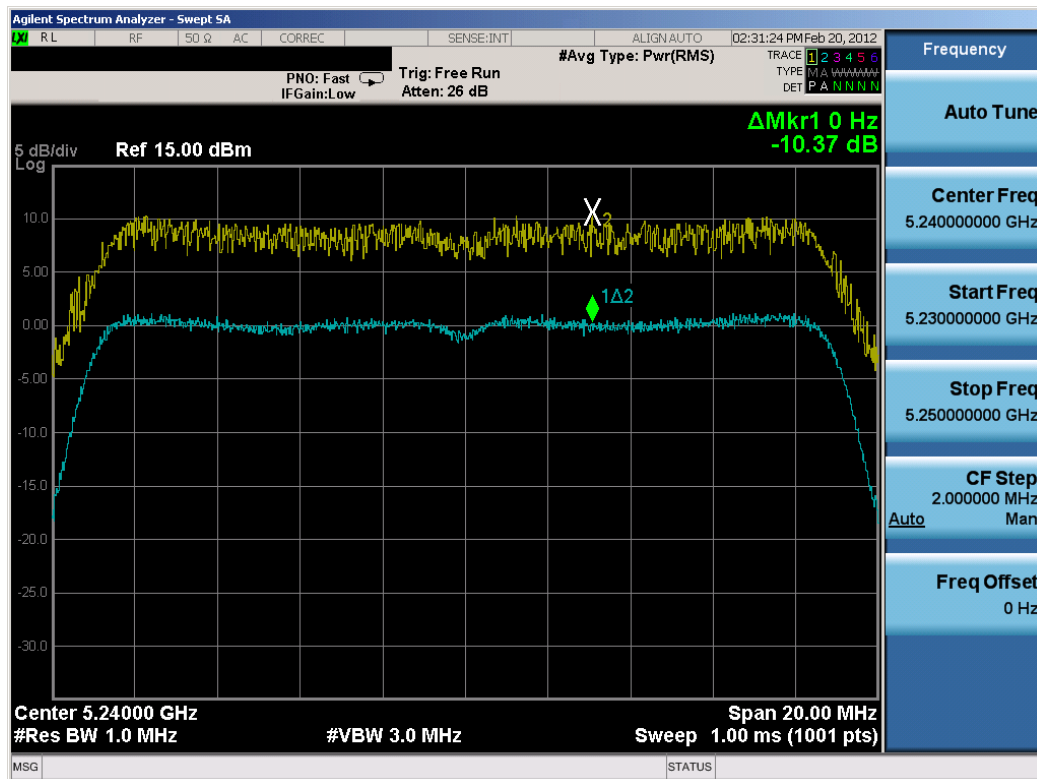
Plot 6-57. Peak Excursion Ratio Plot (802.11n – 20MHz BW (UNII Band 1) – Ch. 48)
