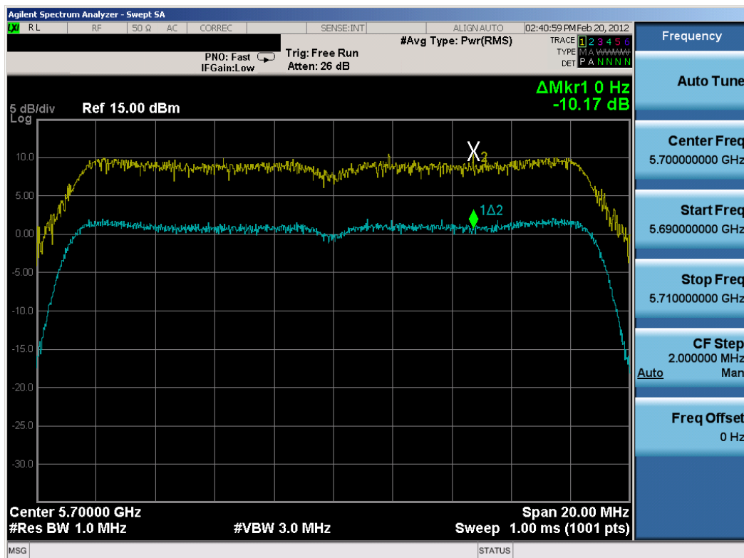
Plot 6-73. Peak Excursion Ratio Plot (802.11n – 20MHz BW (UNII Band 3) – Ch. 140)
