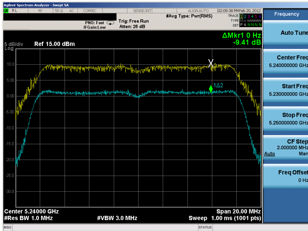
Plot 6-54. Peak Excursion Ratio Plot (802.11a (UNII Band 1) – Ch. 48)
