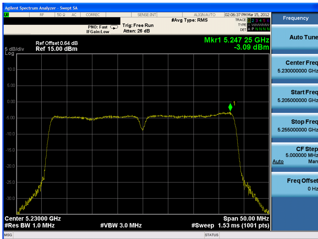
Plot 6-34. Peak Power Spectral Density Plot (802.11n – 40MHz BW (UNII Band 1) – Ch. 46)
