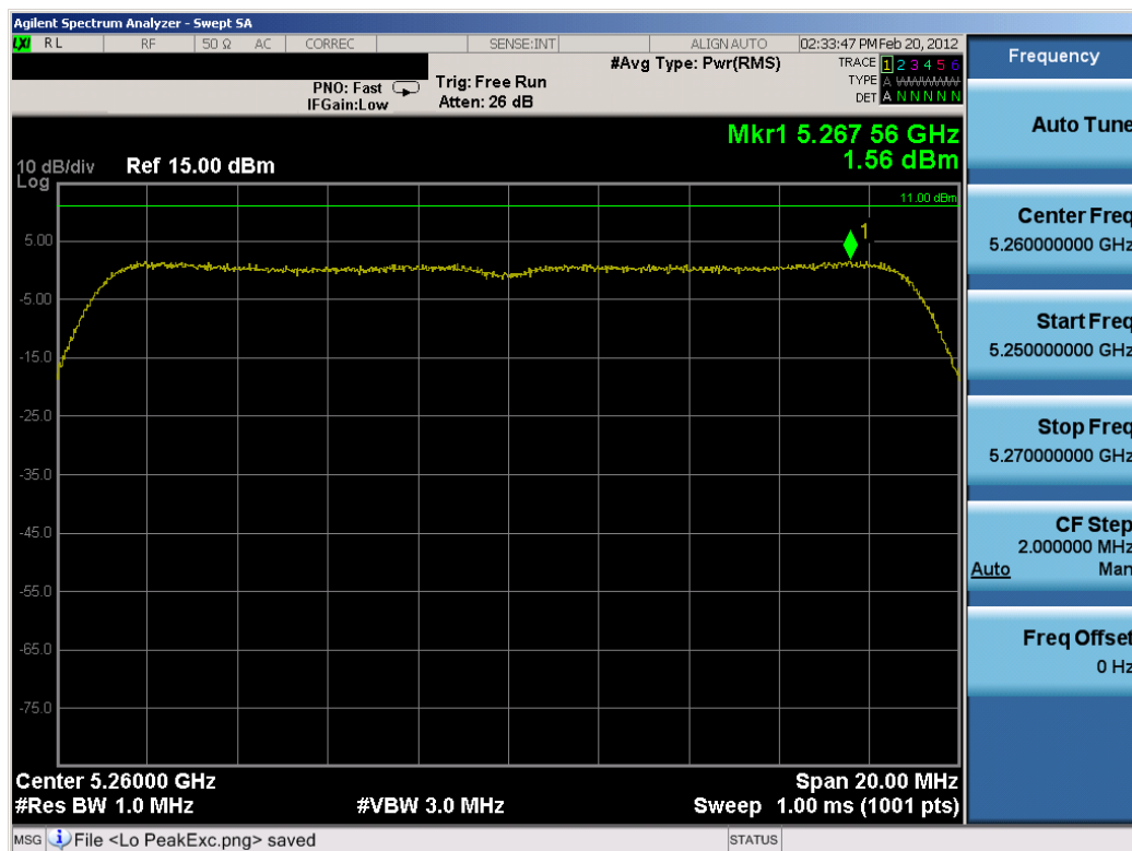
Plot 6-38. Peak Power Spectral Density Plot (802.11n – 20MHz BW (UNII Band 2) – Ch. 52)
