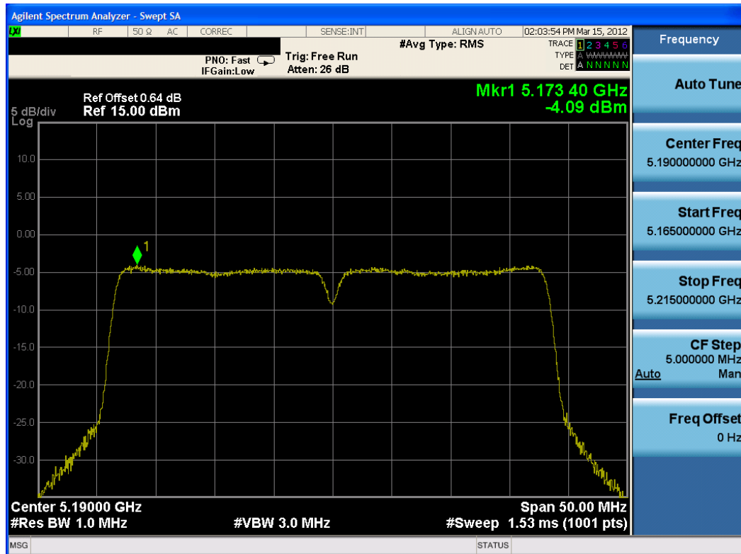
Plot 6-33. Peak Power Spectral Density Plot (802.11n – 40MHz BW (UNII Band 1) – Ch. 38)
