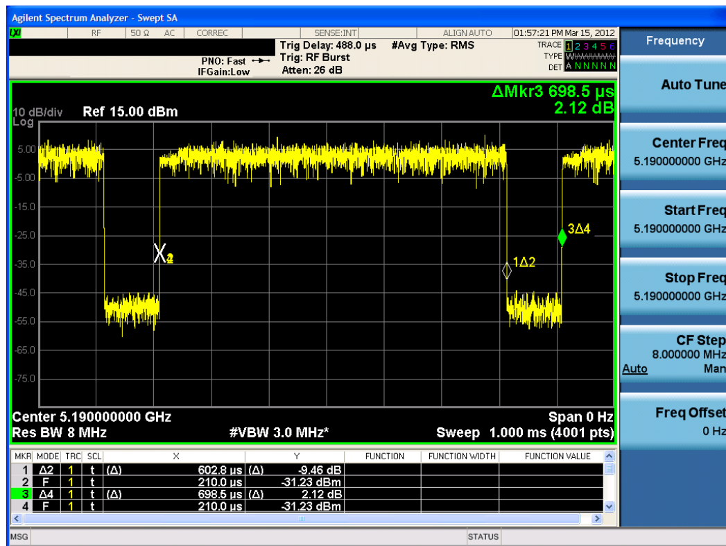
Plot 6-26. Pulse Width for 40MHz 802.11n Signal at MCS0 Data Rate
