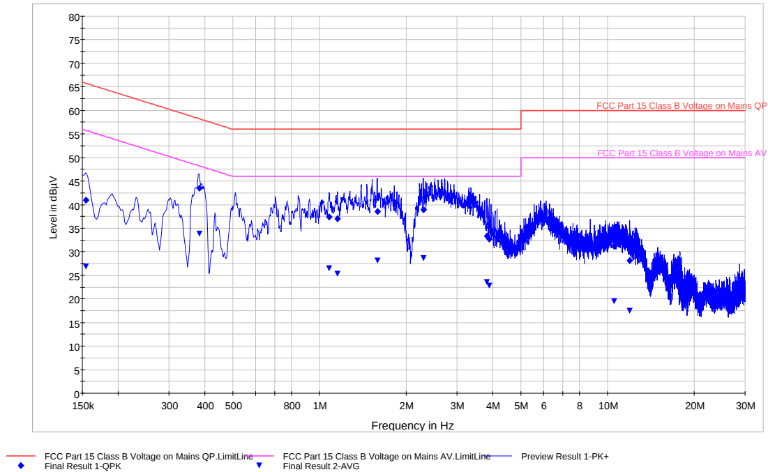
Plot 6-81. Line Conducted Plot with 802.11a (UNII Band 3) (L1)
