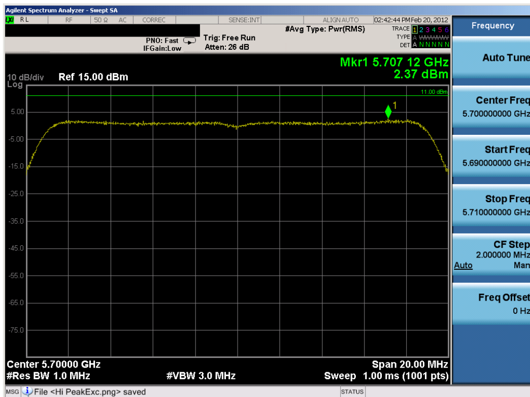
Plot 6-48. Peak Power Spectral Density Plot (802.11n – 20MHz BW (UNII Band 3) – Ch. 140)
