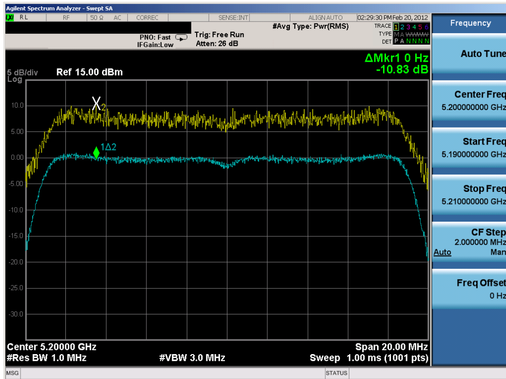
Plot 6-56. Peak Excursion Ratio Plot (802.11n – 20MHz BW (UNII Band 1) – Ch. 40)
