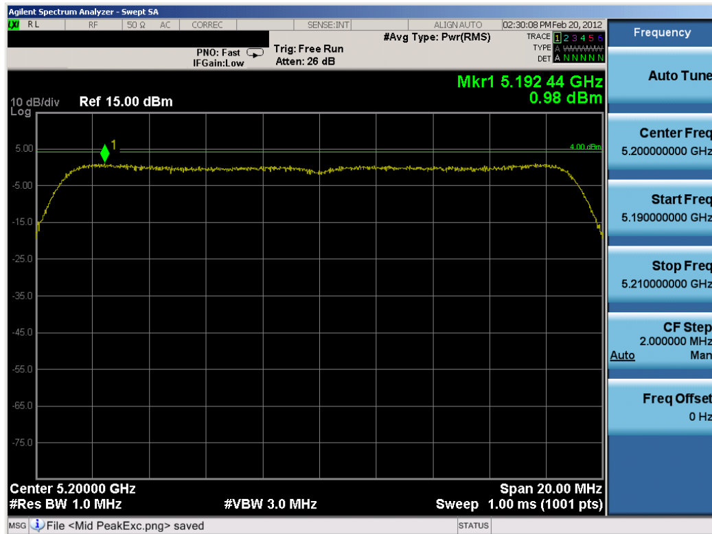
Plot 6-31. Peak Power Spectral Density Plot (802.11n – 20MHz BW (UNII Band 1) – Ch. 40)
