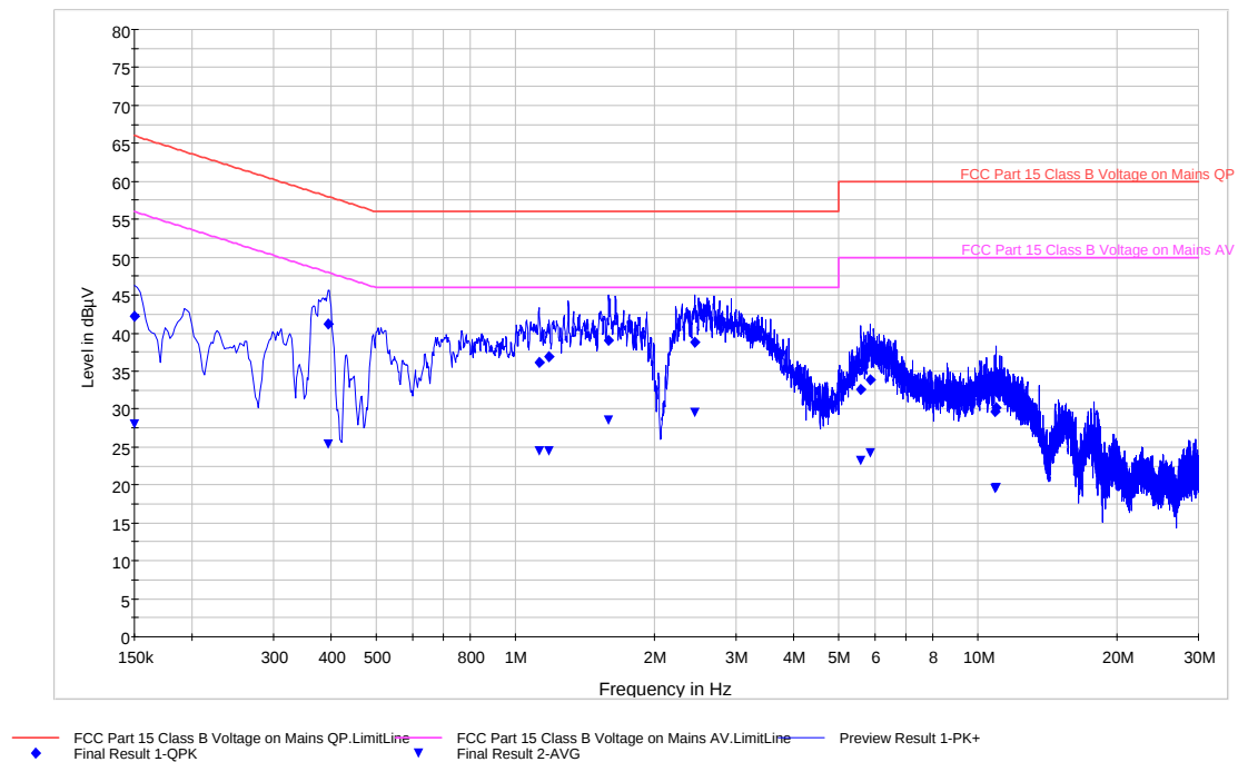
Plot 6-79. Line Conducted Plot with 802.11a (UNII Band 2) (L1)
