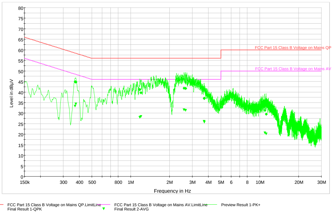
Plot 6-80. Line Conducted Plot with 802.11a (UNII Band 2) (LN)
