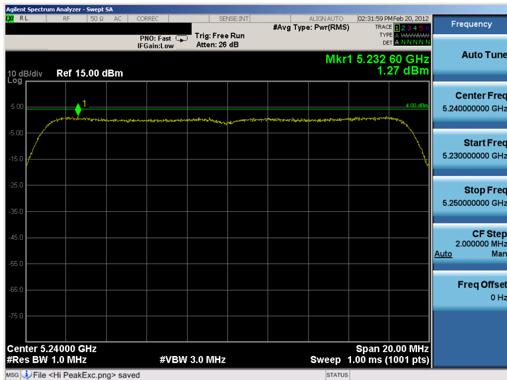
Plot 6-32. Peak Power Spectral Density Plot (802.11n – 20MHz BW (UNII Band 1) – Ch. 48)
