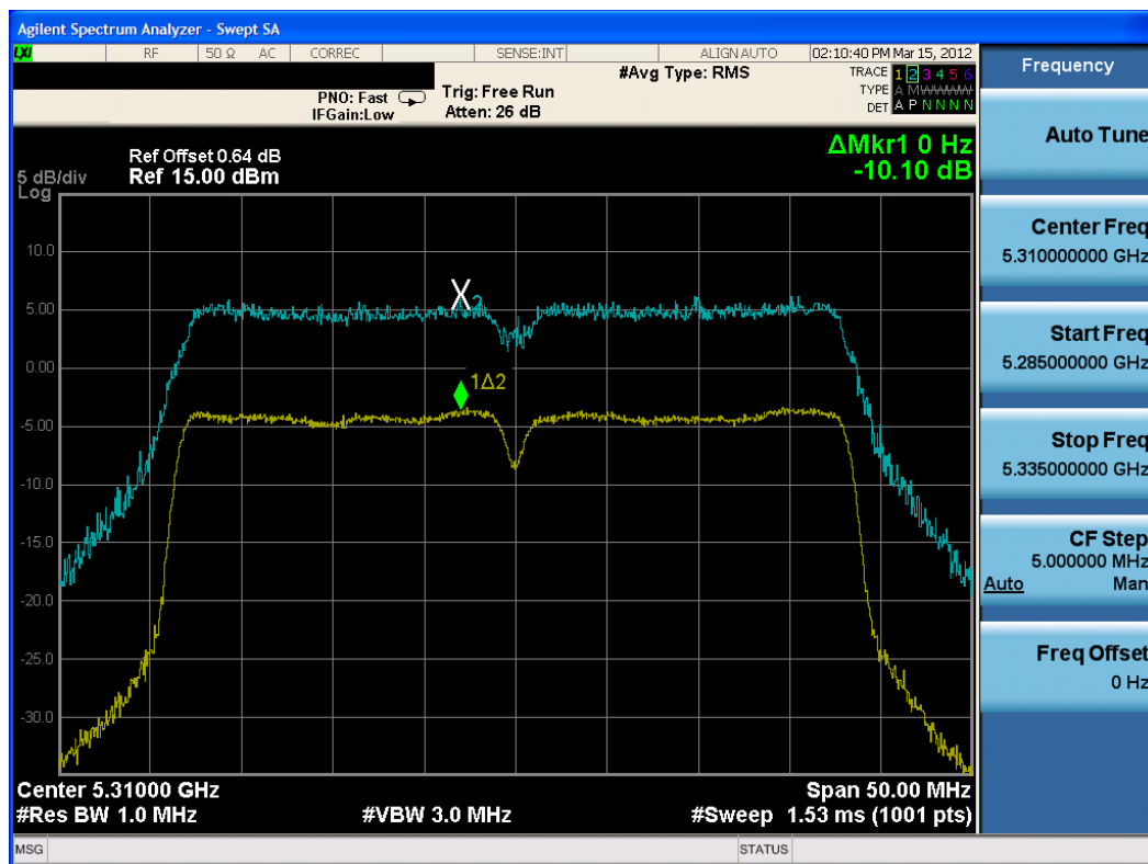
Plot 6-67. Peak Excursion Ratio Plot (802.11n – 40MHz BW (UNII Band 2) – Ch. 62)
