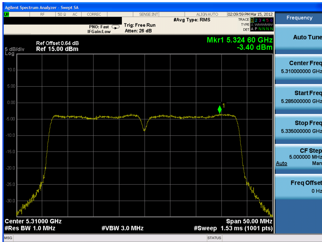
Plot 6-42. Peak Power Spectral Density Plot (802.11n – 40MHz BW (UNII Band 2) – Ch. 62)
