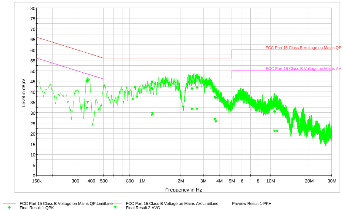
Plot 6-25. Line Conducted Data with Bluetooth (LN)
