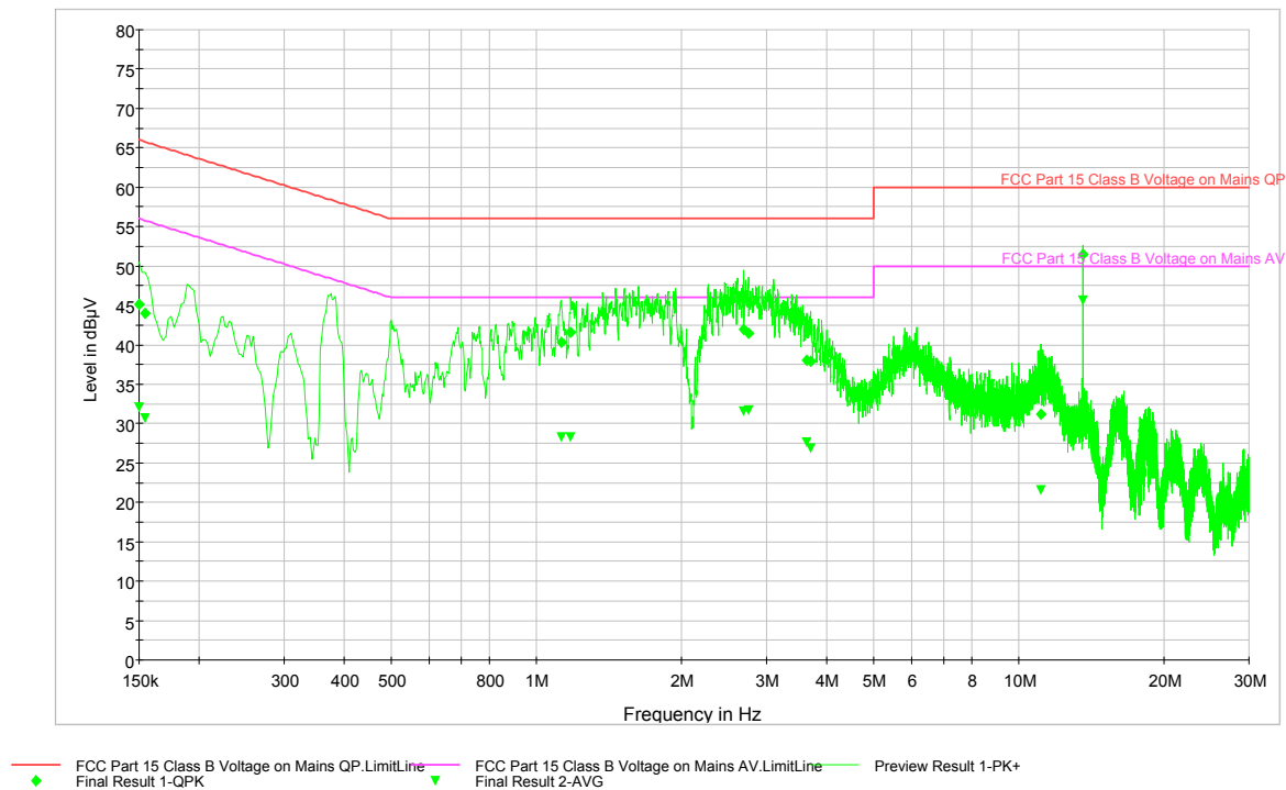
Plot 8-2. Line-Conducted Test Plot (LN)
