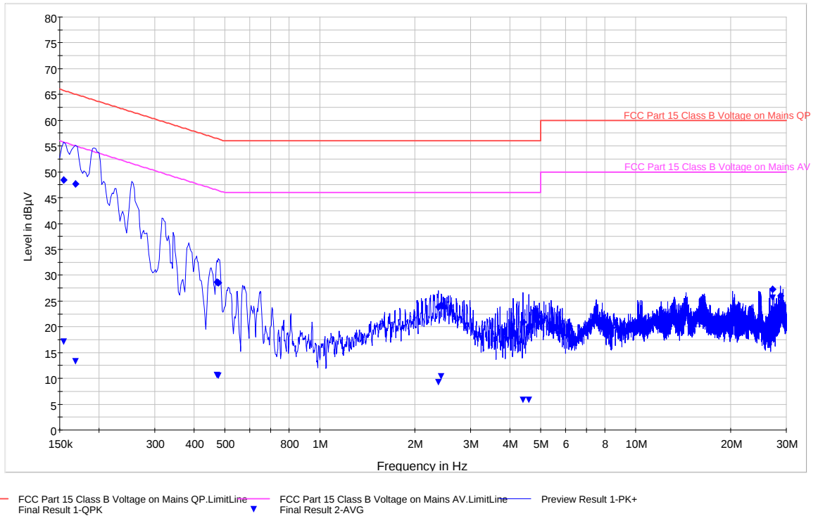
Plot 7-1. Line Conducted Test Plot (L1)
