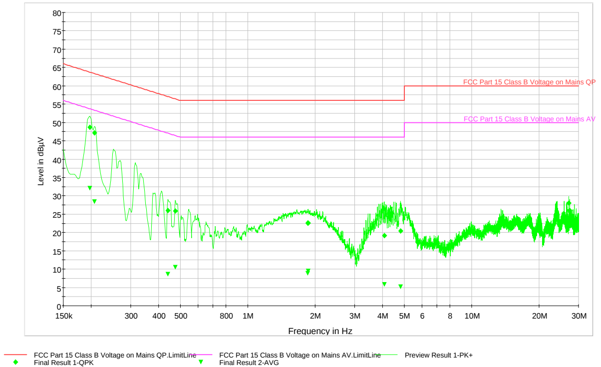
Plot 7-2. Line Conducted Test Data (LN)
