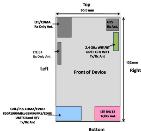
Figure 1-1 DUT Antenna Locations
