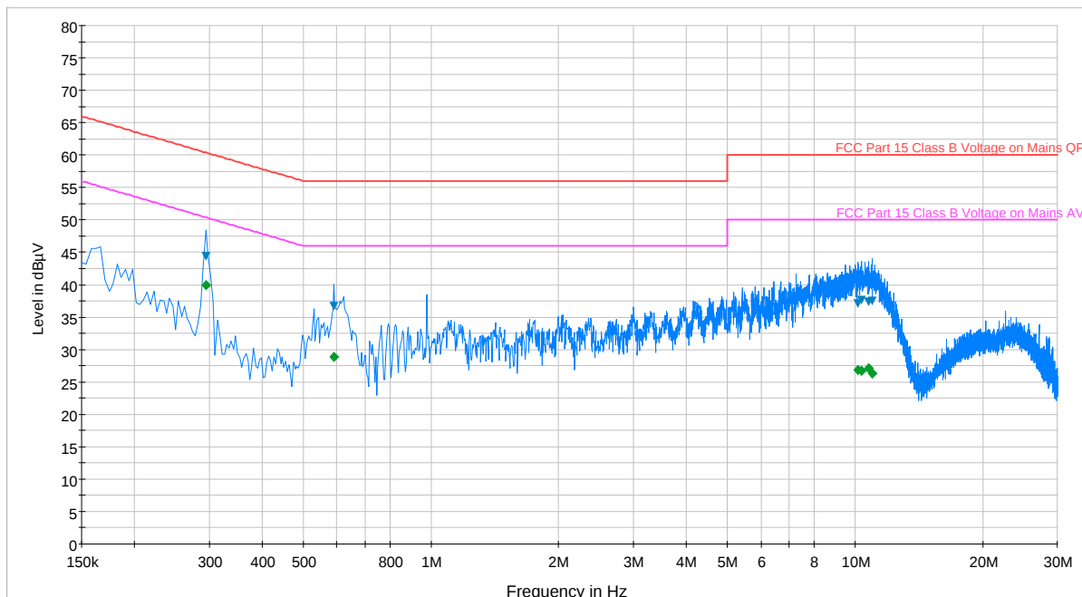
Plot 6-106. Line Conducted Plot with 802.11a UNII Band 2 (N)
