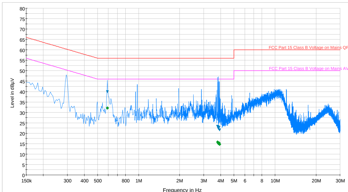
Plot 6-105. Line Conducted Plot with 802.11a UNII Band 2 (L1)
