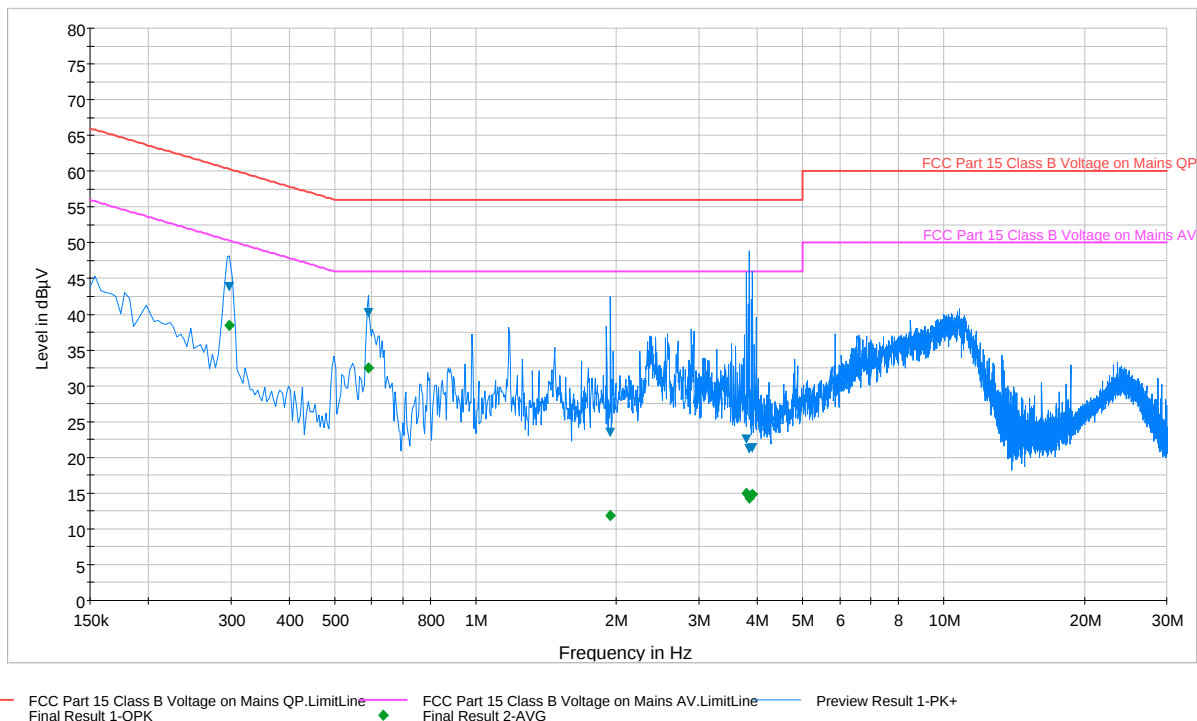
Plot 6-103. Line Conducted Plot with 802.11a UNII Band 1 (L1)
