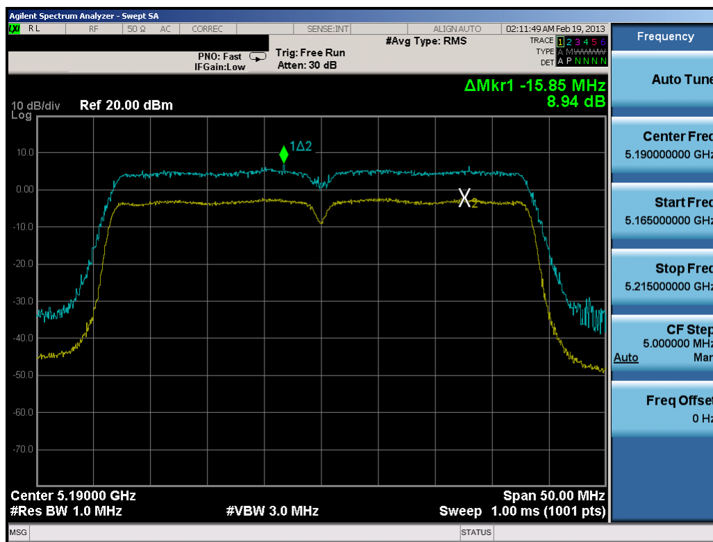
Plot 6-59. Peak Excursion Ratio Plot (40MHz BW 802.11n)
