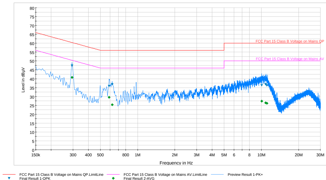
Plot 6-104. Line Conducted Plot with 802.11a UNII Band 1 (N)
