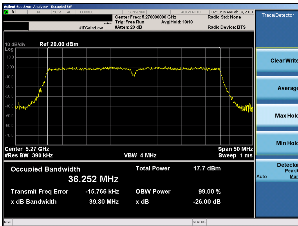
Plot 6-16. 26dB Bandwidth Plot (40MHz BW 802.11n (UNII Band 2) – Ch. 54)
