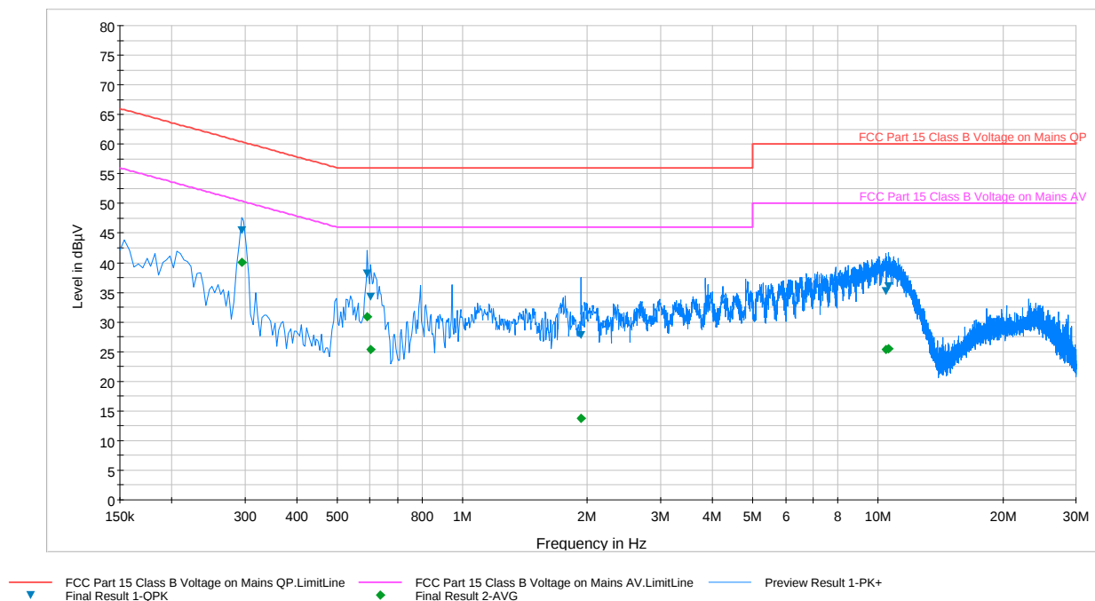
Plot 6-108. Line Conducted Plot with 802.11a UNII Band 3 (N)
