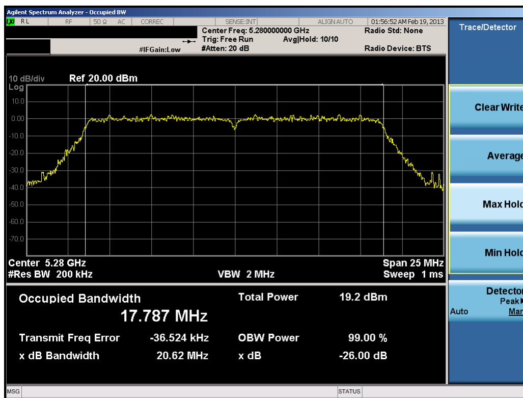
Plot 6-14. 26dB Bandwidth Plot (20MHz BW 802.11n (UNII Band 2) – Ch. 56)
