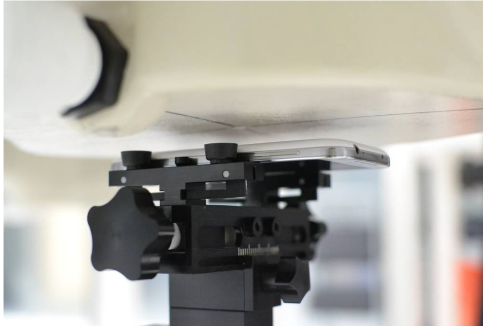
SAR Test Setup Photo 7 – Back side with Wireless Charging Cover at 1.0 cm
