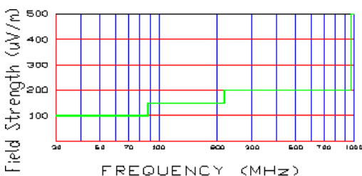
Figure 6-2. 3-Meter Limits
