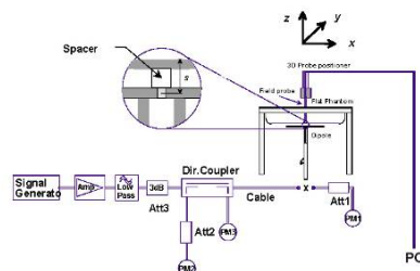
Figure 12-1 System Verification Setup Diagram
