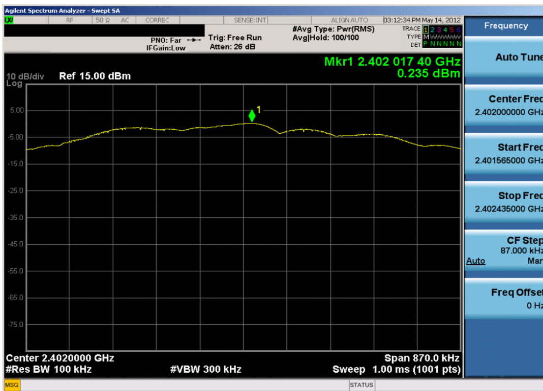
Plot 6-4. Power Spectral Density Plot (Bluetooth (LE) – Ch. 0)
