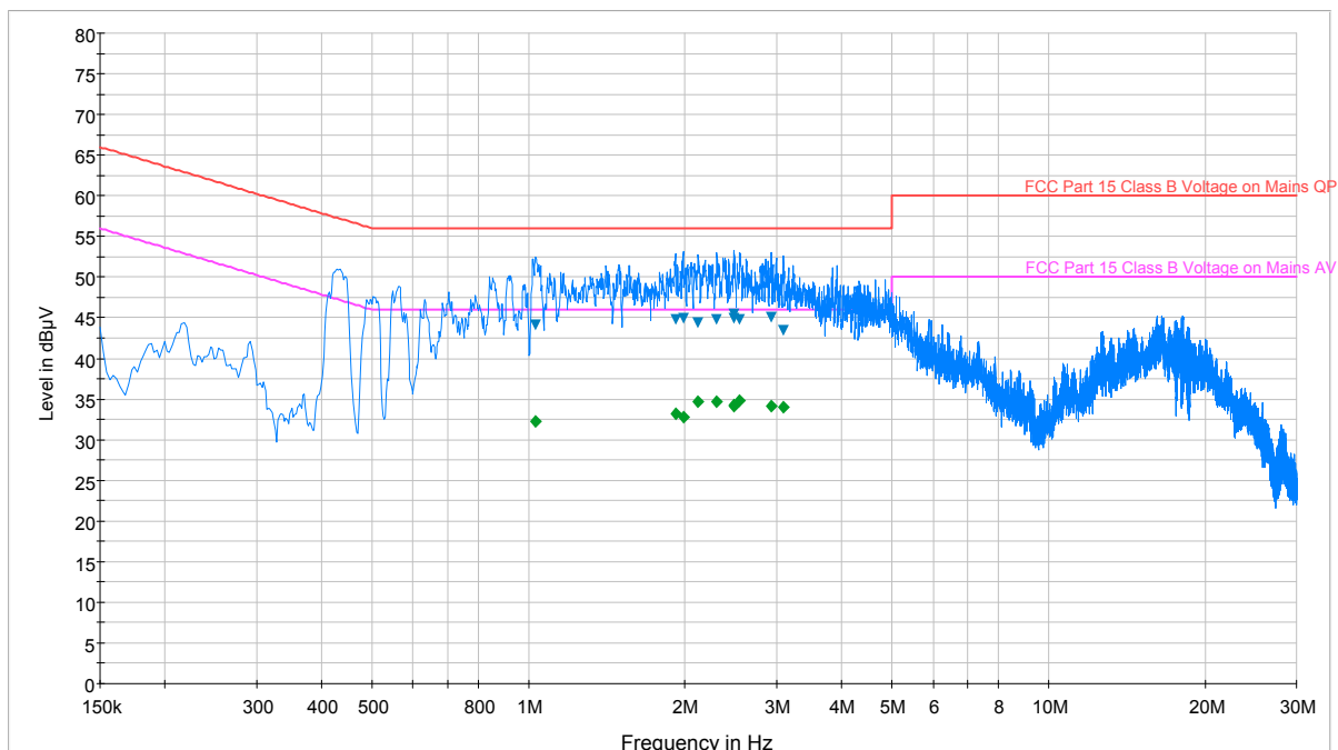
Plot 6-16. Line Conducted Plot with Bluetooth (LE, N)
