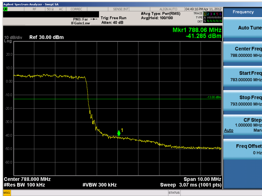
Plot 7-11. Upper Band Edge Plot (QPSK – RB Size 25, RB Offset 25)
