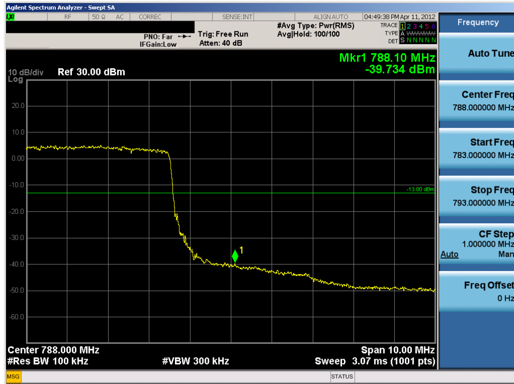
Plot 7-12. Upper Band Edge Plot (16-QAM – RB Size 25, RB Offset 25)
