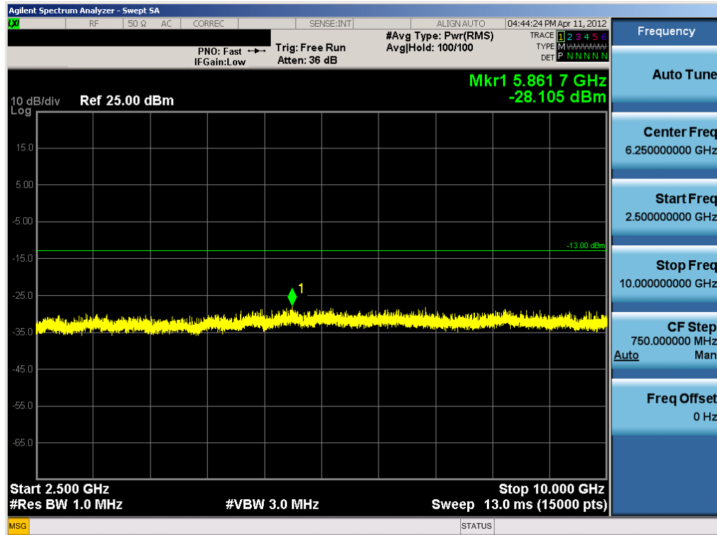
Plot 7-10. Conducted Spurious Plot (16-QAM – RB Size 1, RB Offset 0)
