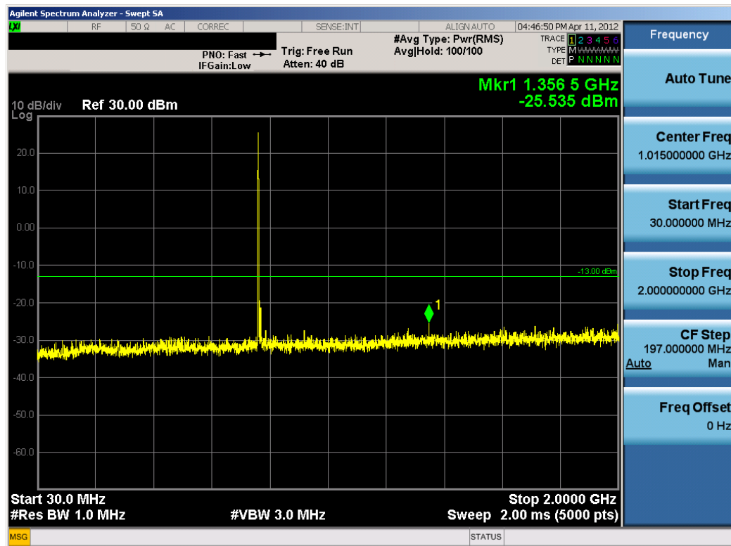
Plot 7-9. Conducted Spurious Plot (16-QAM – RB Size 1, RB Offset 0)
