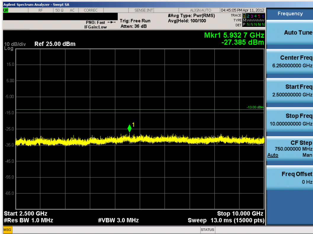
Plot 7-8. Conducted Spurious Plot (QPSK – RB Size 1, RB Offset 0)
