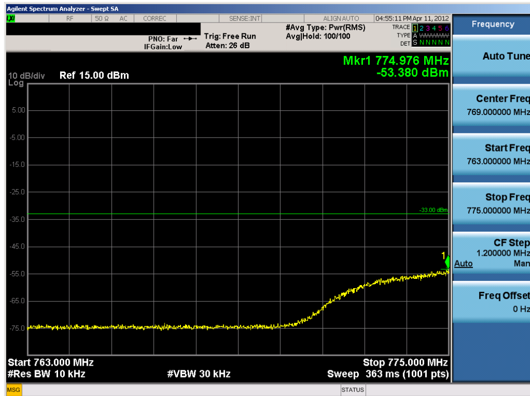
Plot 7-4. Lower Emission Mask (763 – 775MHz) Plot (16-QAM – RB Size 45, Offset 0)
