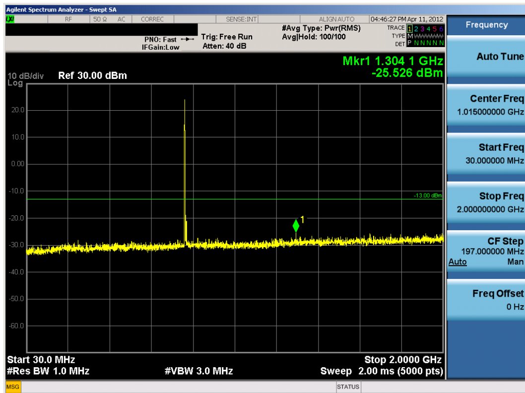
Plot 7-7. Conducted Spurious Plot (QPSK – RB Size 1, RB Offset 0)
