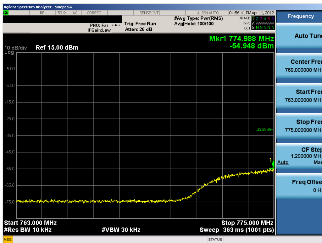
Plot 7-3. Lower Emission Mask (763 – 775MHz) Plot (QPSK – RB Size 45, Offset 0)
