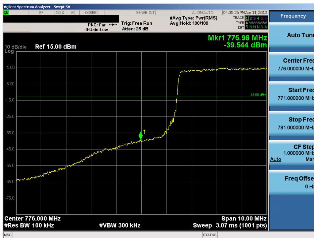
Plot 7-2. Lower Band Edge Plot (16-QAM – RB Size 25, RB Offset 0)
