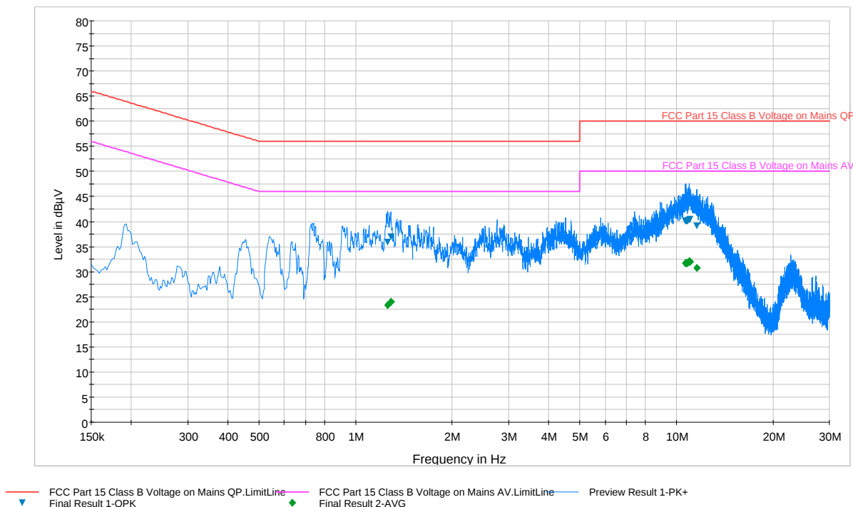
Plot 6-32. Line Conducted Plot with 802.11b (N)
