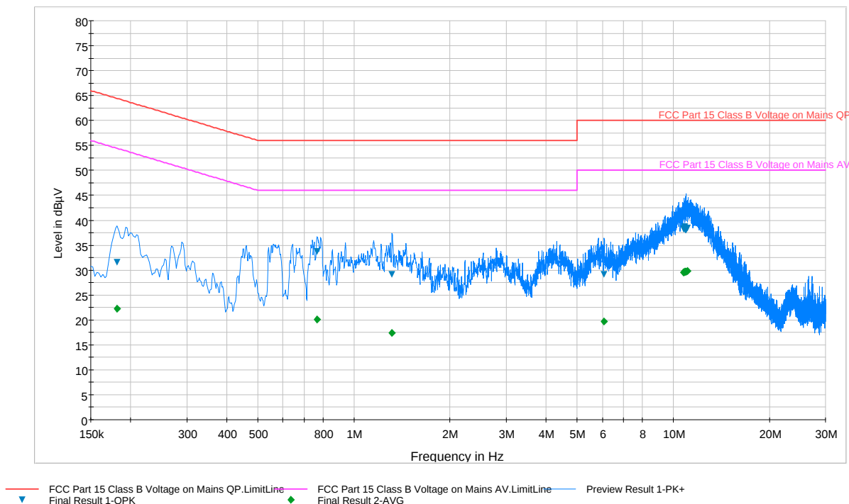
Plot 6-31. Line Conducted Plot with 802.11b (L1)
