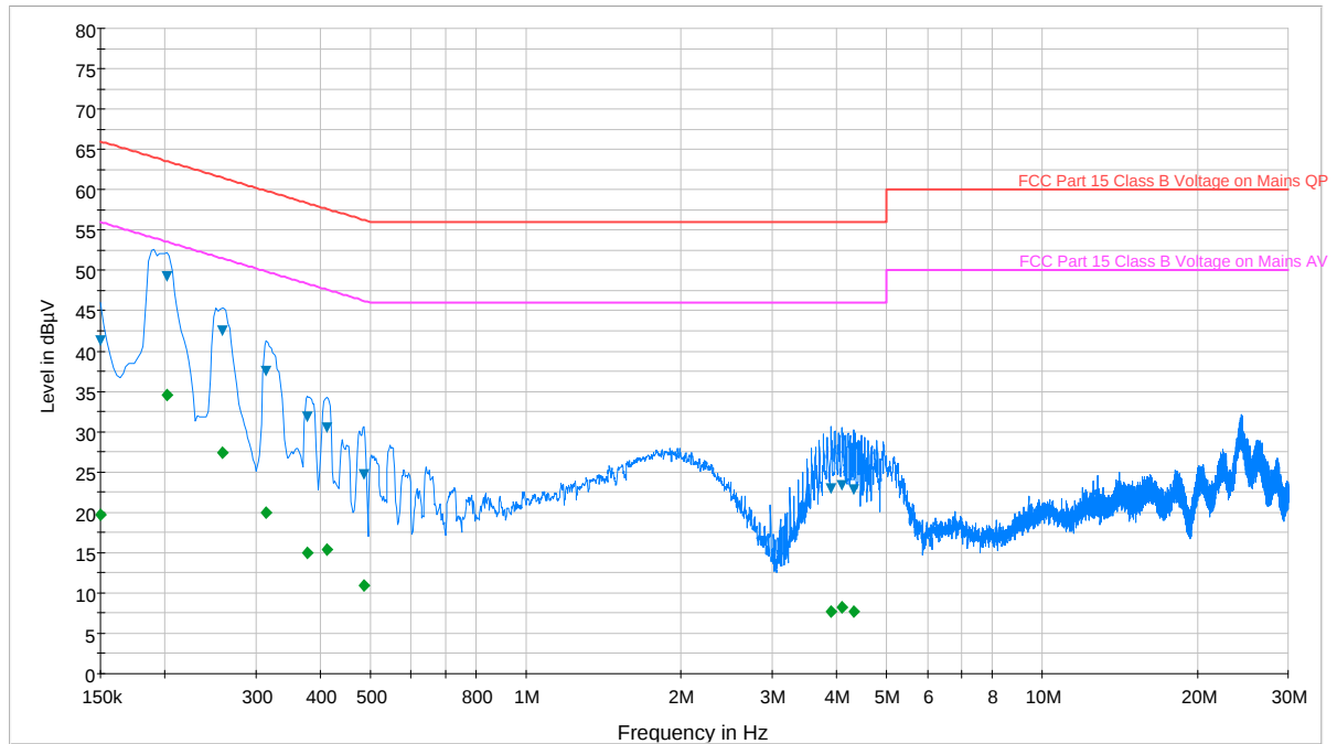
Plot 7-2. Line-Conducted Test Plot (N)
