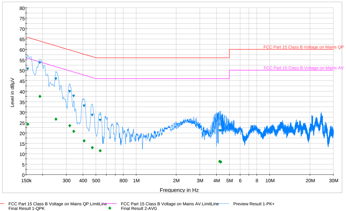
Plot 7-1. Line-Conducted Test Plot (L1)
