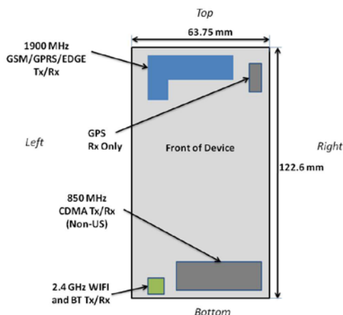
Figure 1-1 DUT Antenna Locations
