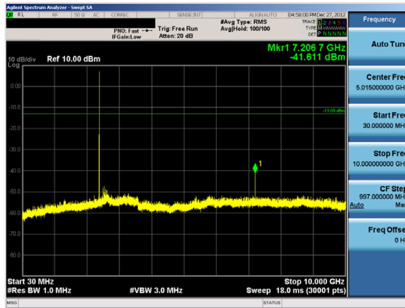
Plot 6-36. Conducted Spurious Plot (Bluetooth, 1Mbps – Ch. 0)
