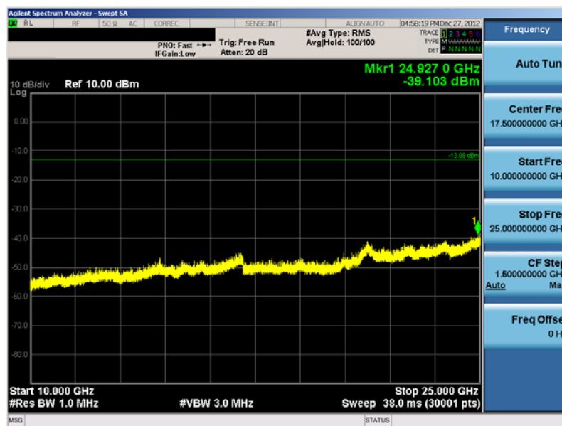
Plot 6-37. Conducted Spurious Plot (Bluetooth, 1Mbps – Ch. 0)
