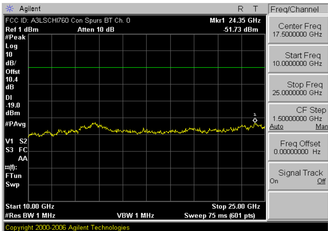
Plot 6-13. Conducted Spurious Plot (Bluetooth – Ch. 0)
