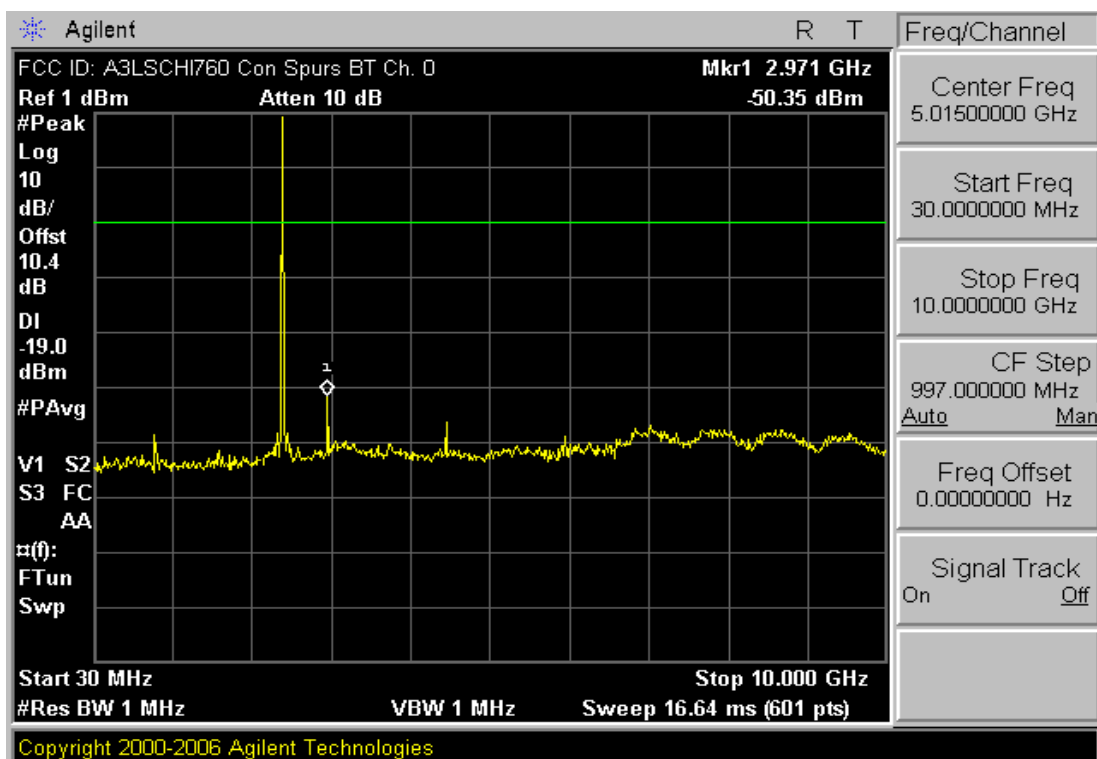
Plot 6-12. Conducted Spurious Plot (Bluetooth – Ch. 0)
