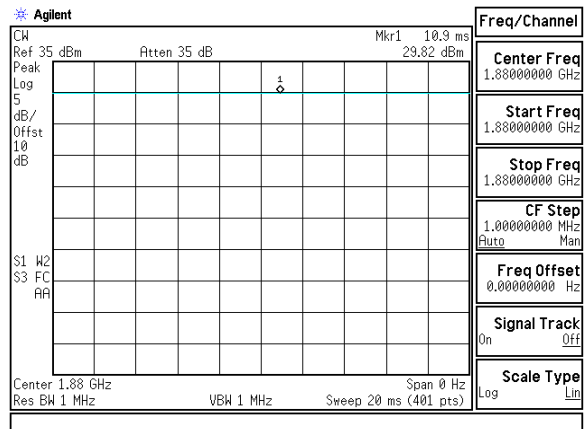
Figure 8-8 PCS CW Signal
