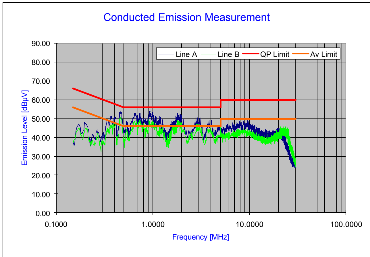
Plot 6-2. Line Conducted Plot with 802.11g
