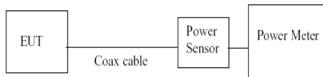
Figure 6-10. Test Instrument & Measurement Setup
