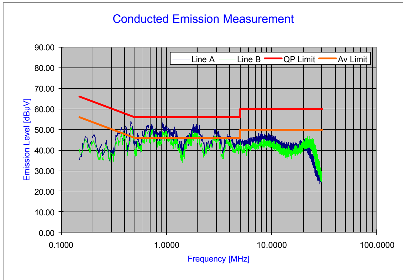
Plot 6-1. Line Conducted Plot with 802.11b
