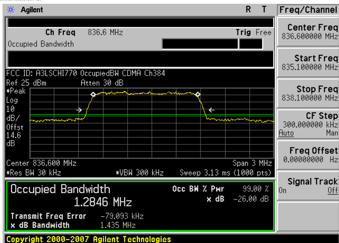
Plot 7-25. Occupied Bandwidth Plot (Cellular CDMA Mode – Ch. 384)
