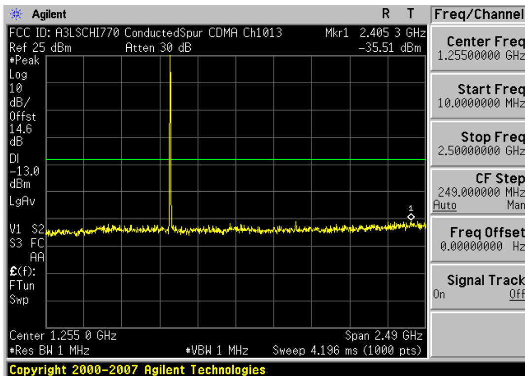
Plot 7-19. Conducted Spurious Plot (Cellular CDMA Mode – Ch. 1013)
