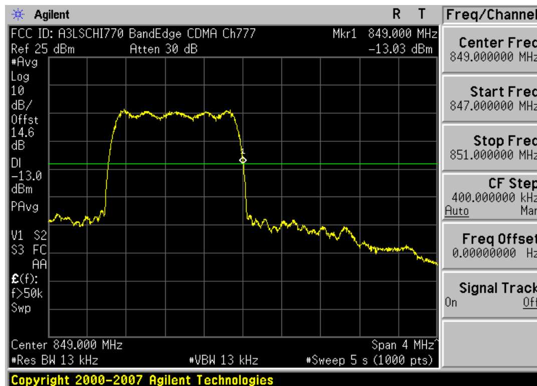
Plot 7-28. Band Edge Plot (Cellular CDMA Mode – Ch. 777)
