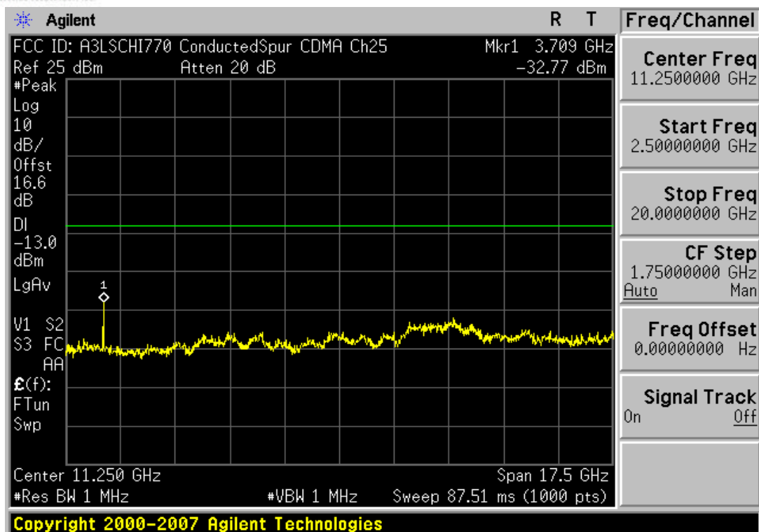
Plot 7-31. Conducted Spurious Plot (PCS CDMA Mode – Ch. 25)
