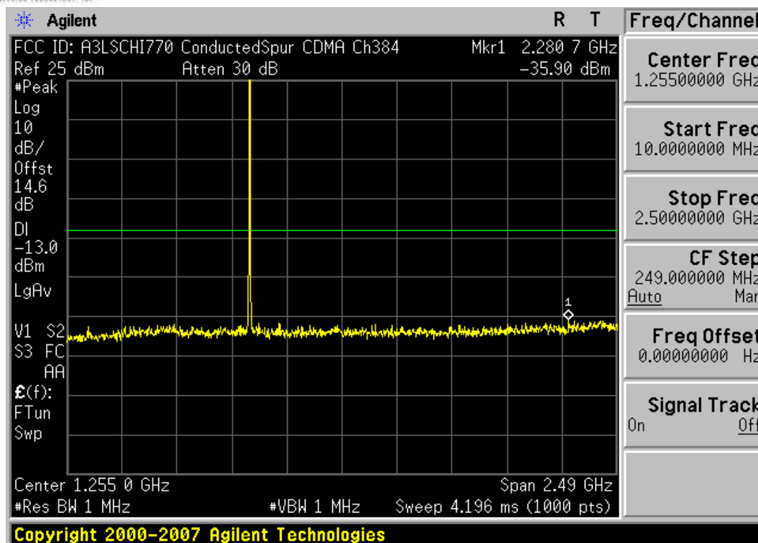
Plot 7-23. Conducted Spurious Plot (Cellular CDMA Mode – Ch. 384)
