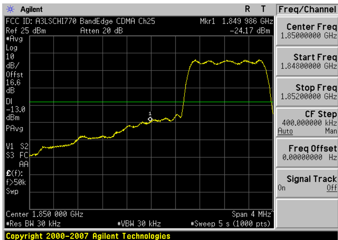
Plot 7-32. Band Edge Plot (PCS CDMA Mode – Ch. 25)
