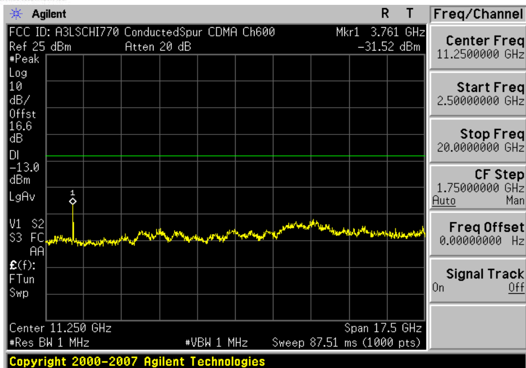
Plot 7-35. Conducted Spurious Plot (PCS CDMA Mode – Ch. 600)
