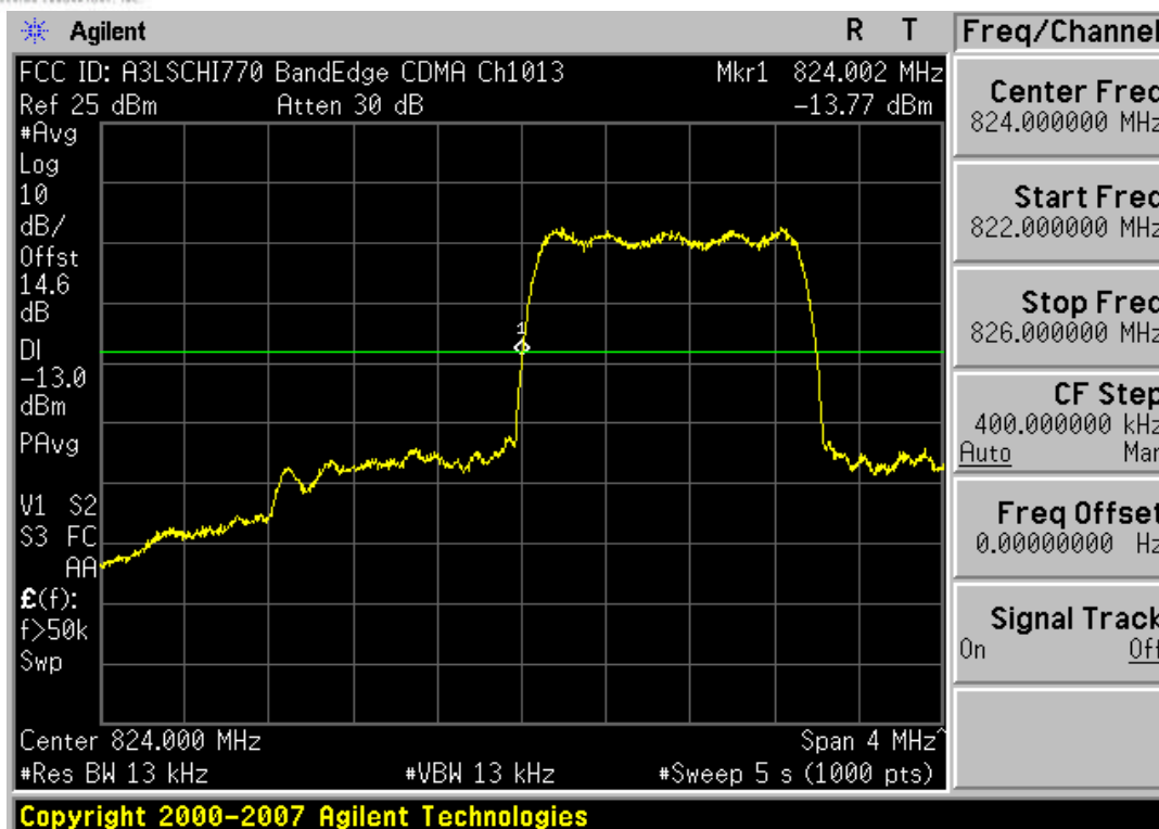
Plot 7-21. Band Edge Plot (Cellular CDMA Mode – Ch. 1013)
