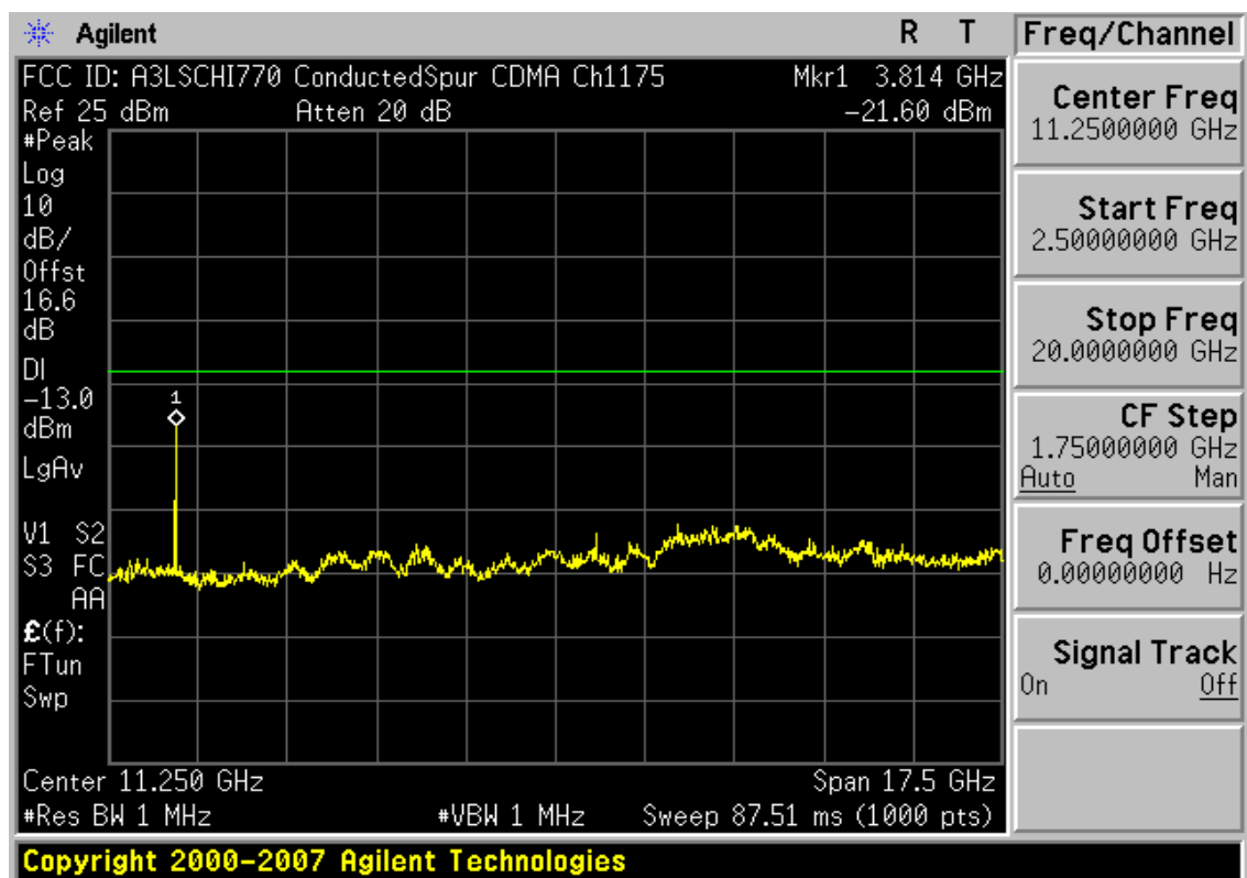
Plot 7-38. Conducted Spurious Plot (PCS CDMA Mode – Ch. 1175)
