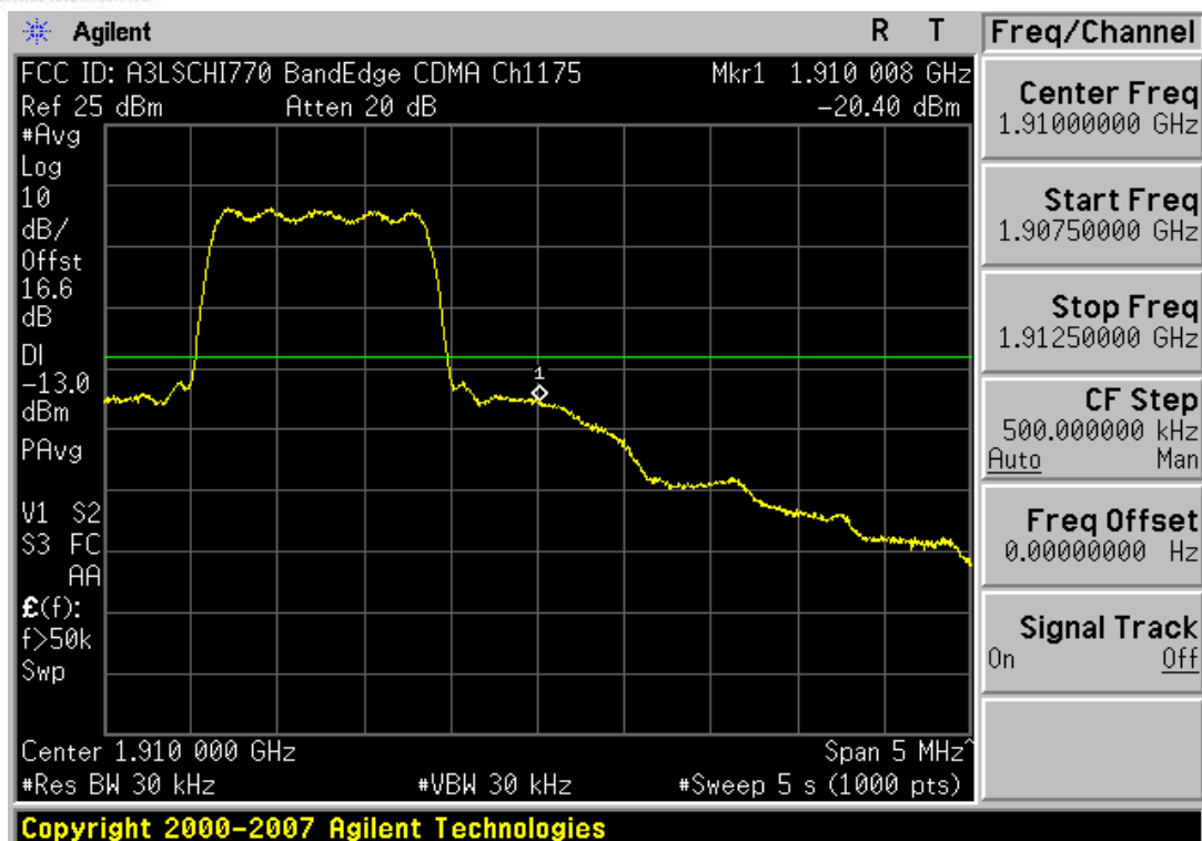
Plot 7-39. Band Edge Plot (PCS CDMA Mode – Ch. 1175)
