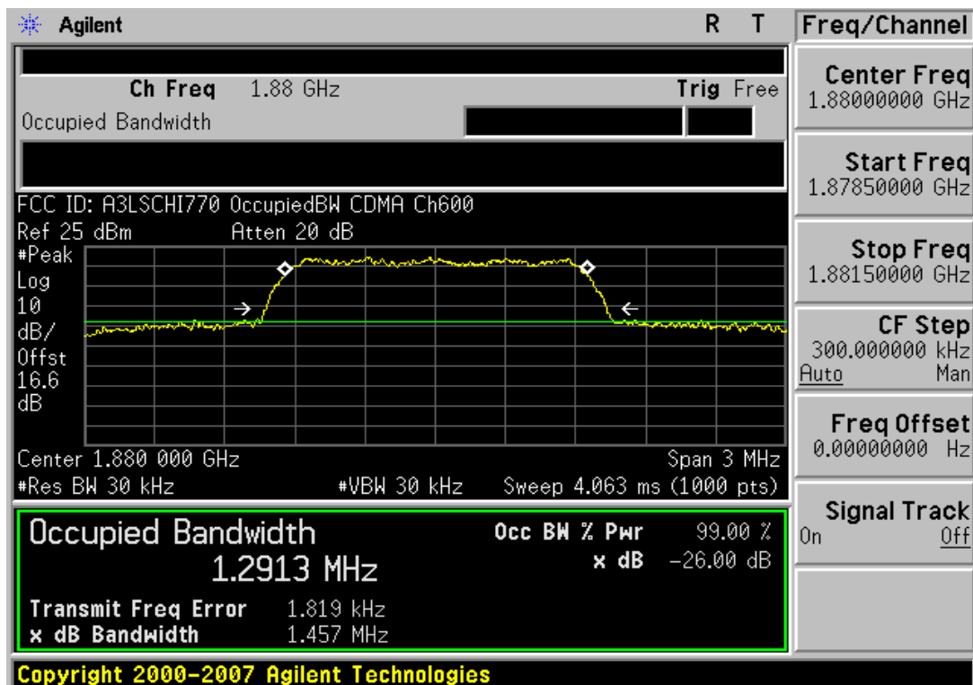
Plot 7-36. Occupied Bandwidth Plot (PCS CDMA Mode – Ch. 600)
