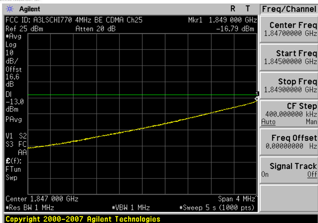
Plot 7-33. 4MHz Span Plot (PCS CDMA Mode – Ch. 25)
