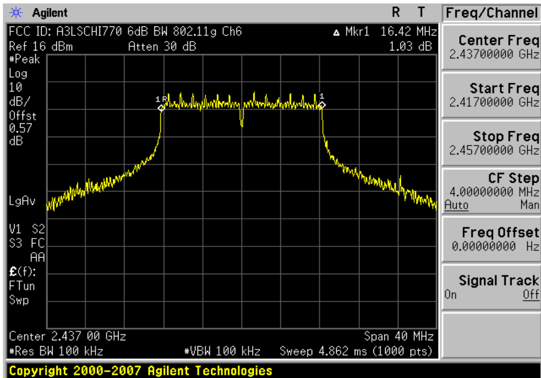
Plot 6-5. 6dB Bandwidth Plot (802.11g - Ch. 6)
