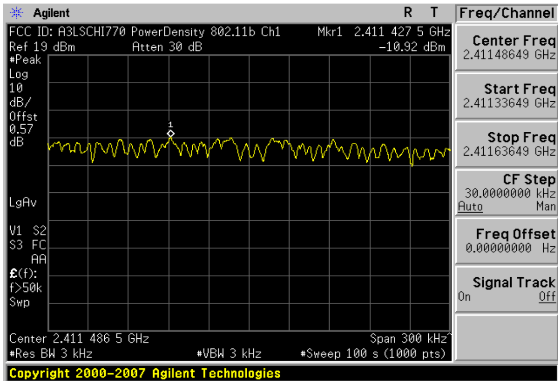
Plot 6-7. Power Spectral Density Plot (802.11b – Ch. 1)
