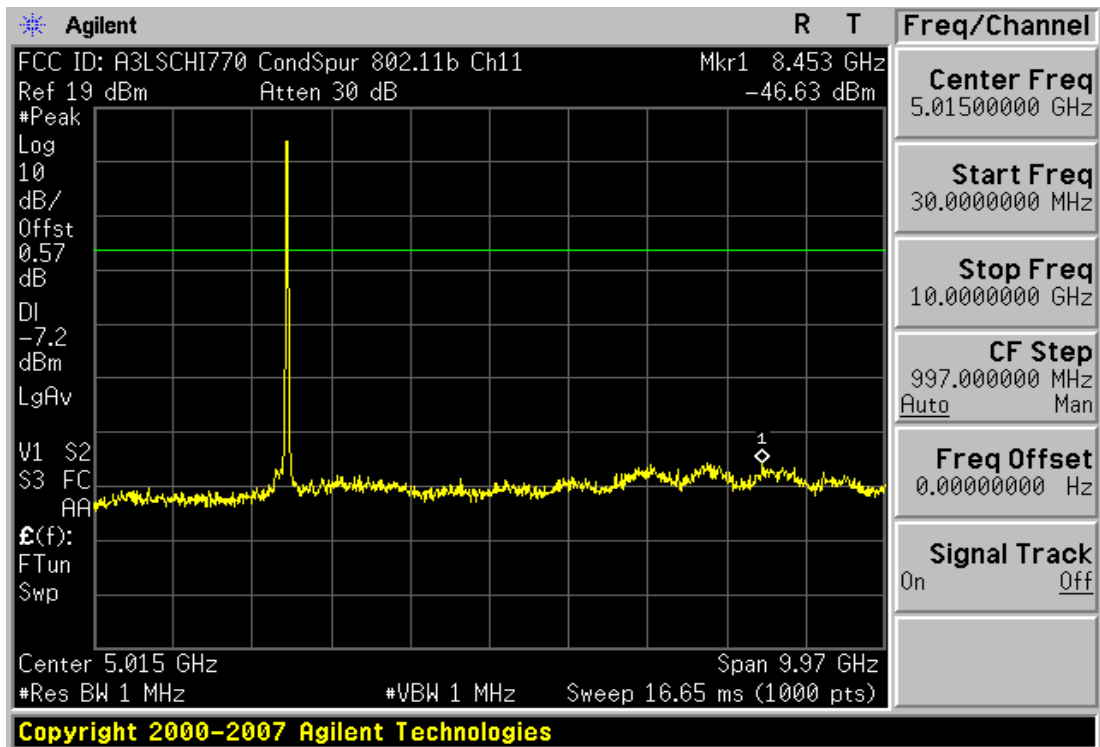
Plot 6-21. Conducted Spurious Plot (802.11b – Ch. 11)
