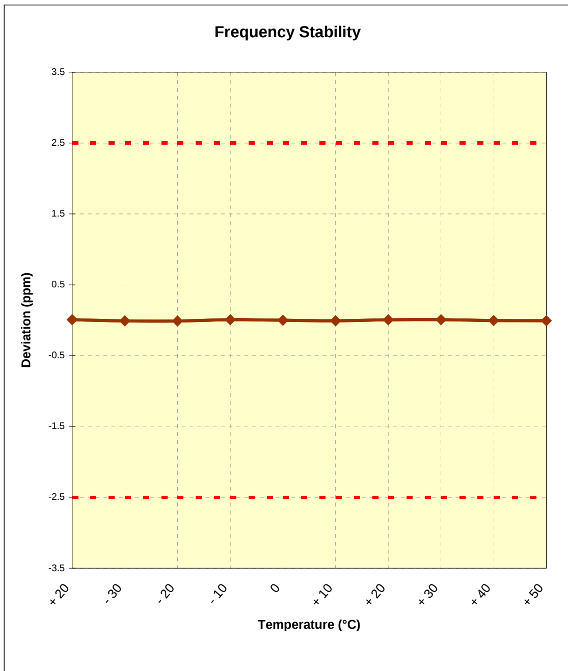
Figure 6-1. Frequency Stability Graph (PCS GSM Mode – Ch. 661)
