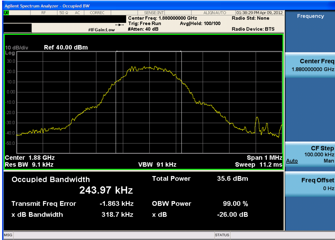
Plot 7-11. Occupied Bandwidth Plot (EDGE1900 Mode – Ch. 661)
