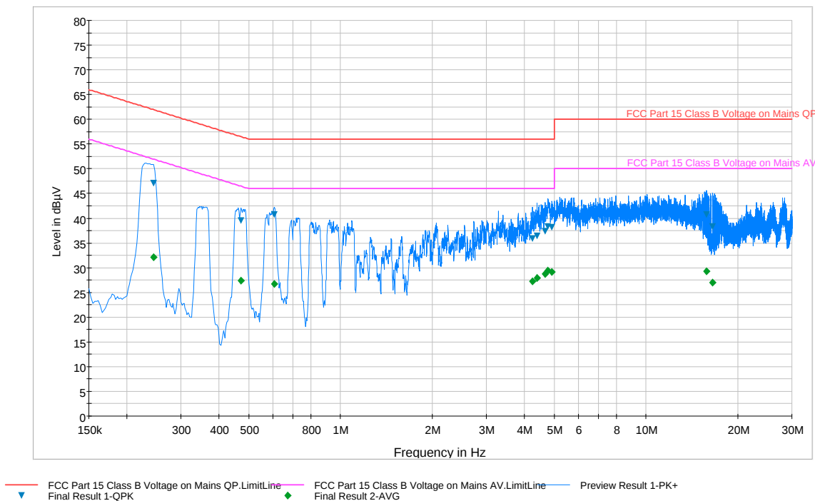
Plot 6-24. Line Conducted Plot with Bluetooth (L1)
