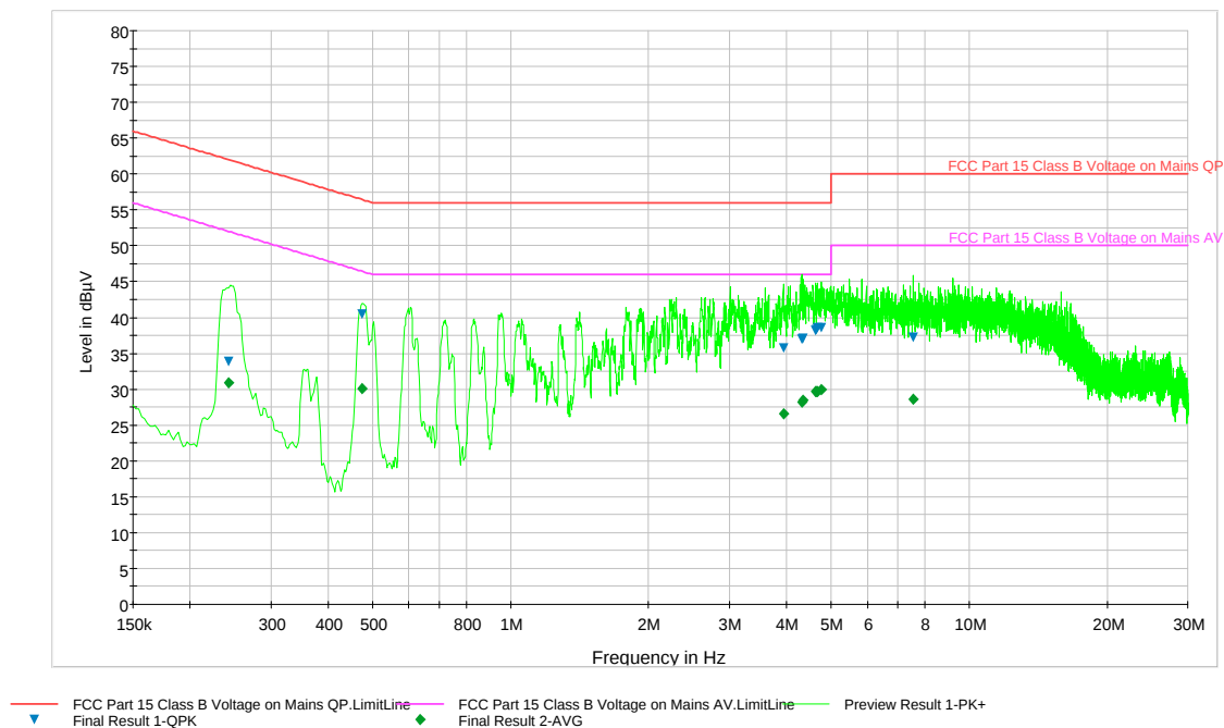
Plot 6-25. Line Conducted Data with Bluetooth (LN)
