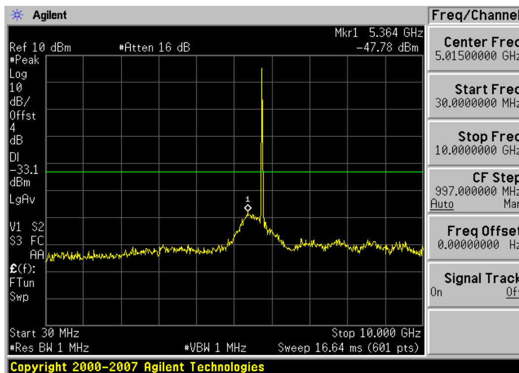
Plot 6-47. Conducted Spurious Plot (802.11a – Ch. 149)
