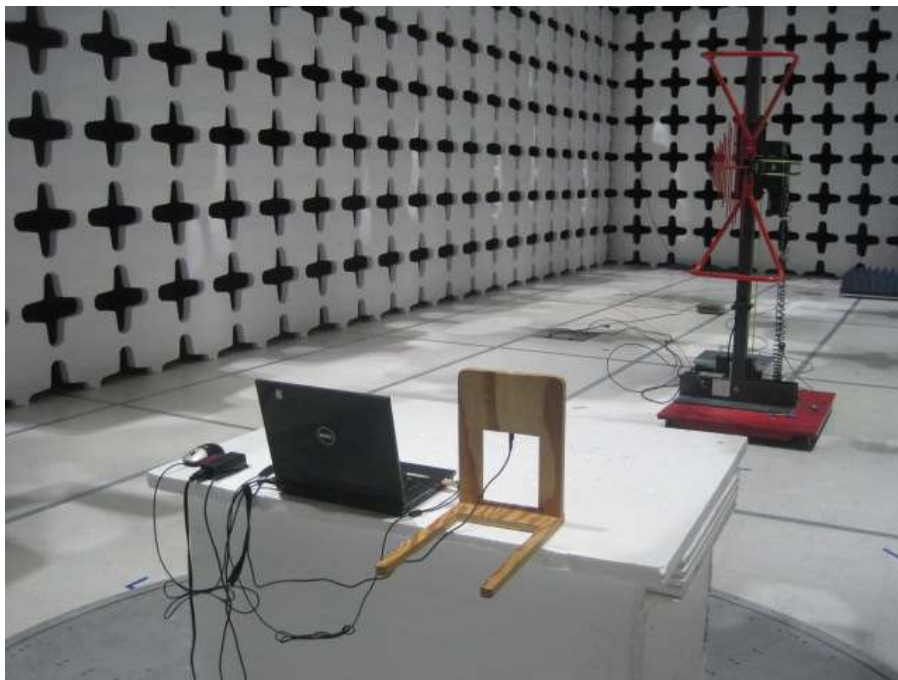
Part 15B Radiated Emission Below 1 GHz Back View
