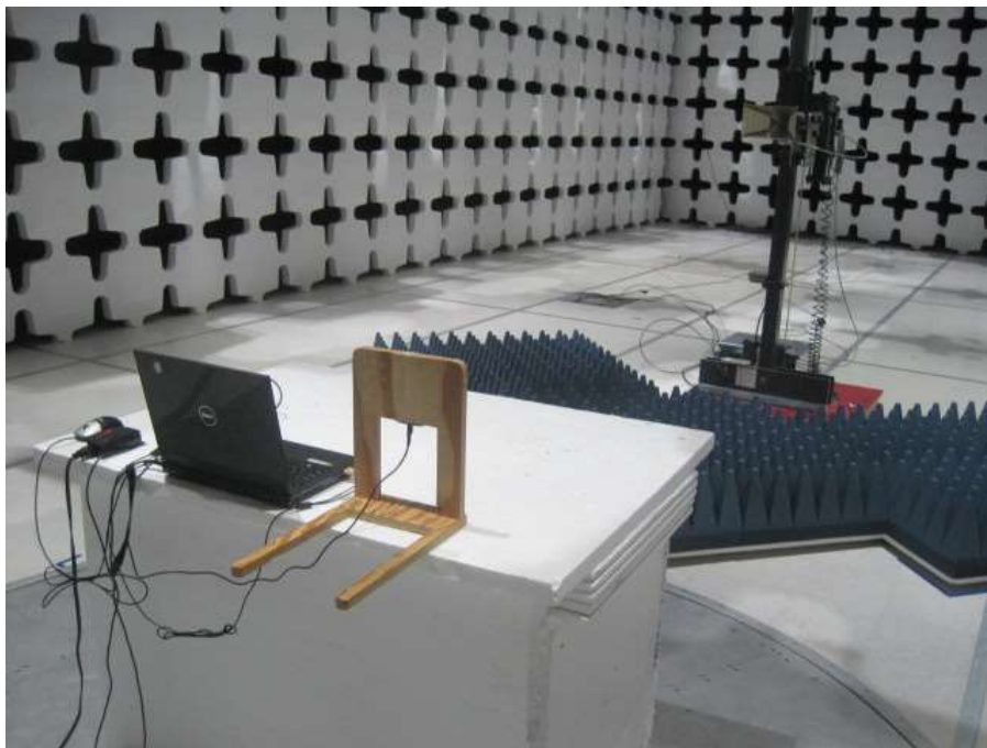
Part 15B Radiated Emission above 1 GHz Back View
