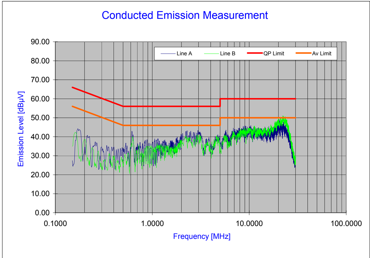
Plot 6-35. Line Conducted Plot with 802.11b
