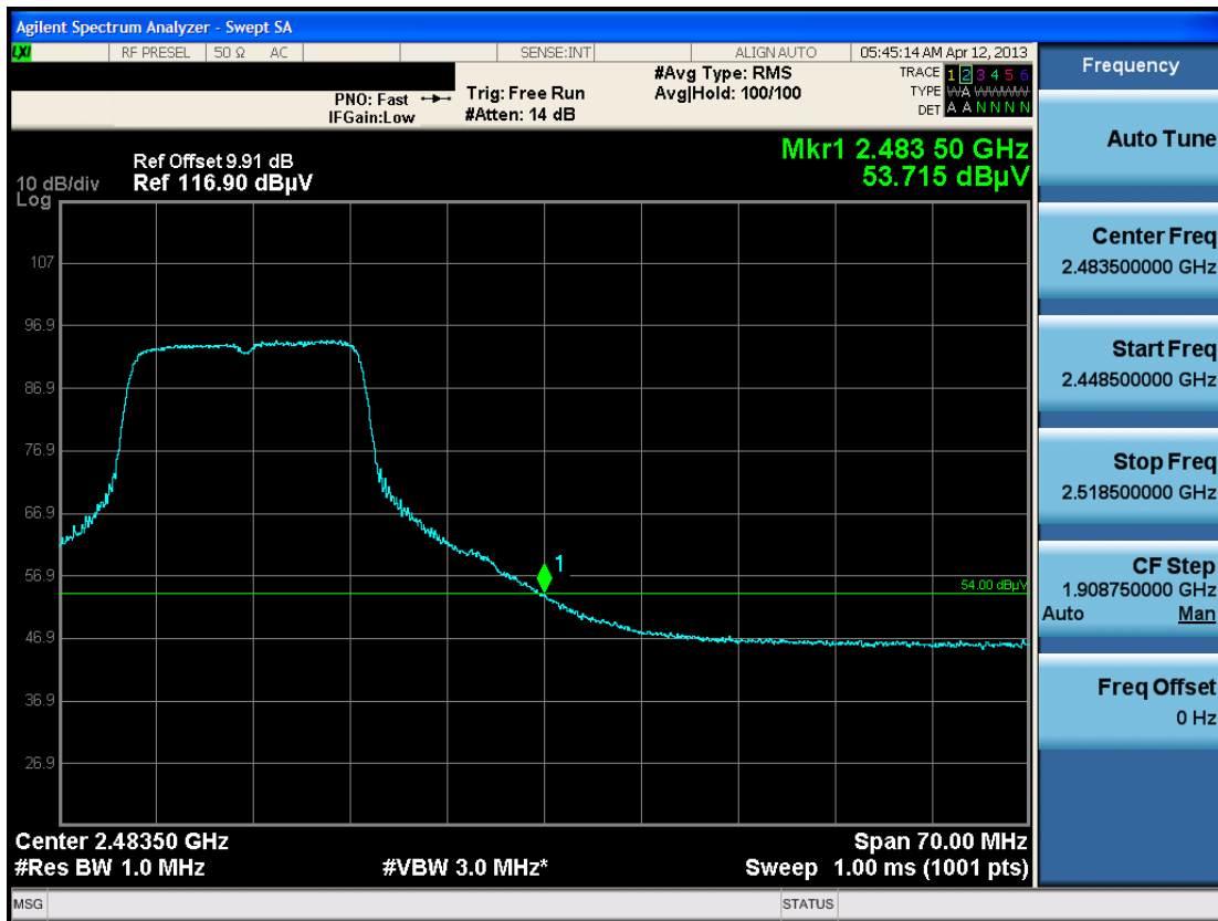
Plot 6-33. Radiated Restricted Upper Band Edge Measurement (Average)
