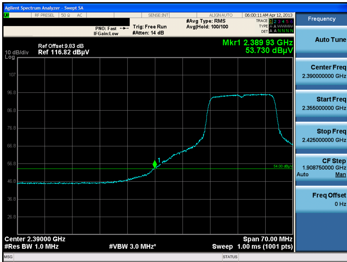
Plot 6-31. Radiated Restricted Lower Band Edge Measurement (Average)
