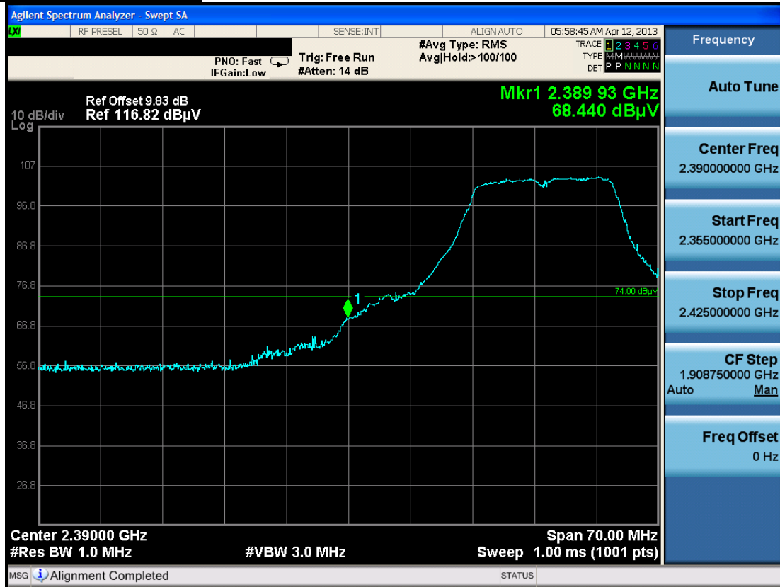
Plot 6-32. Radiated Restricted Lower Band Edge Measurement (Peak)
