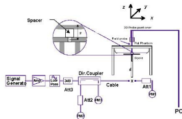
Figure 14-1 System Verification Setup Diagram
