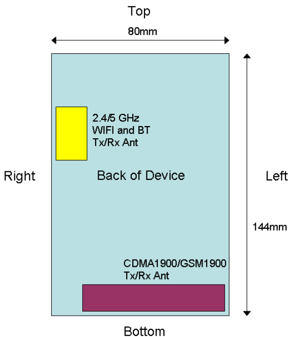
Figure 13-1 Identification of Sides for SAR Testing
