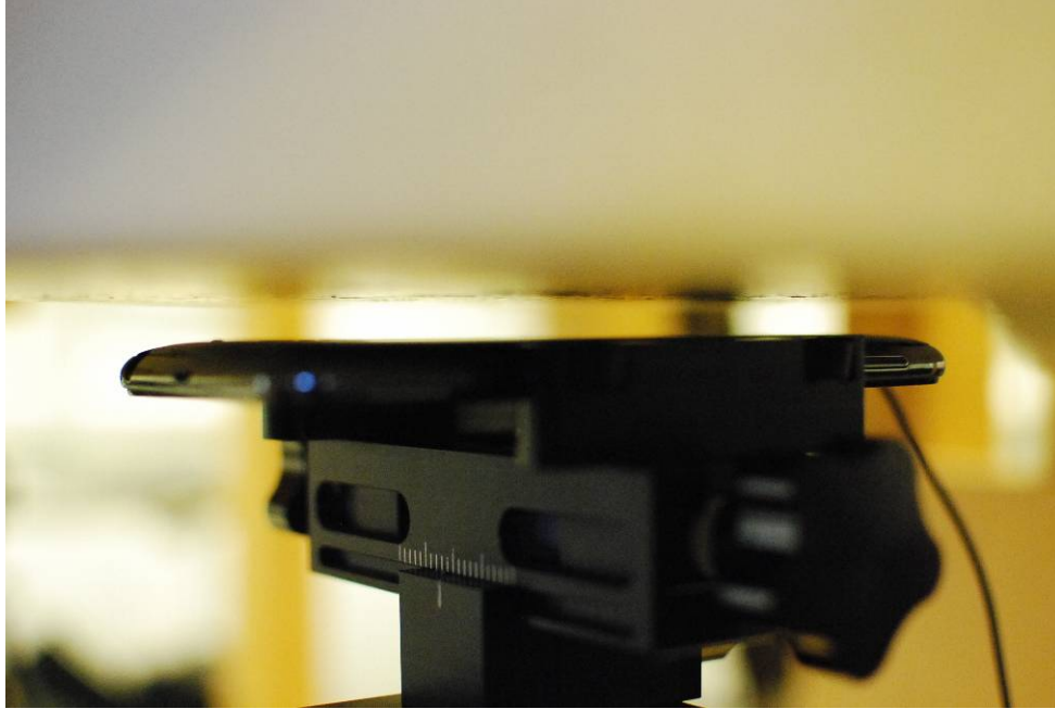
SAR Test Setup Photo 11: Body Worn at 1.0 cm
