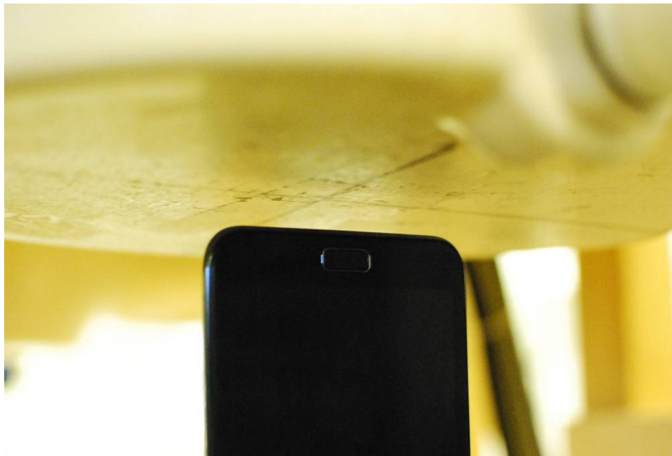
SAR Test Setup Photo 8: Body Bottom at 1.0 cm
