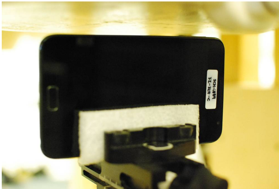
SAR Test Setup Photo 10: Body Left at 1.0 cm
