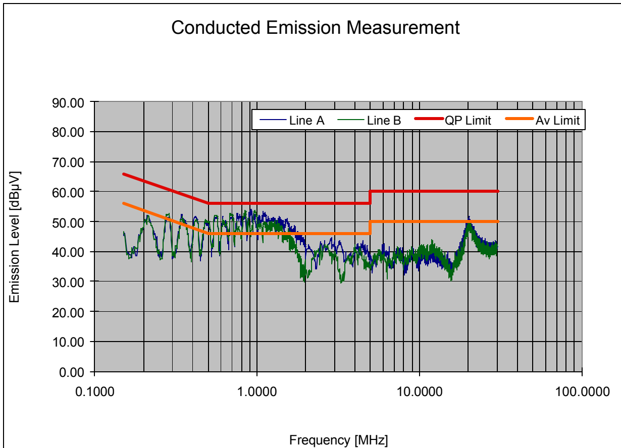
Plot 6-56. Line Conducted Plot with 802.11n
