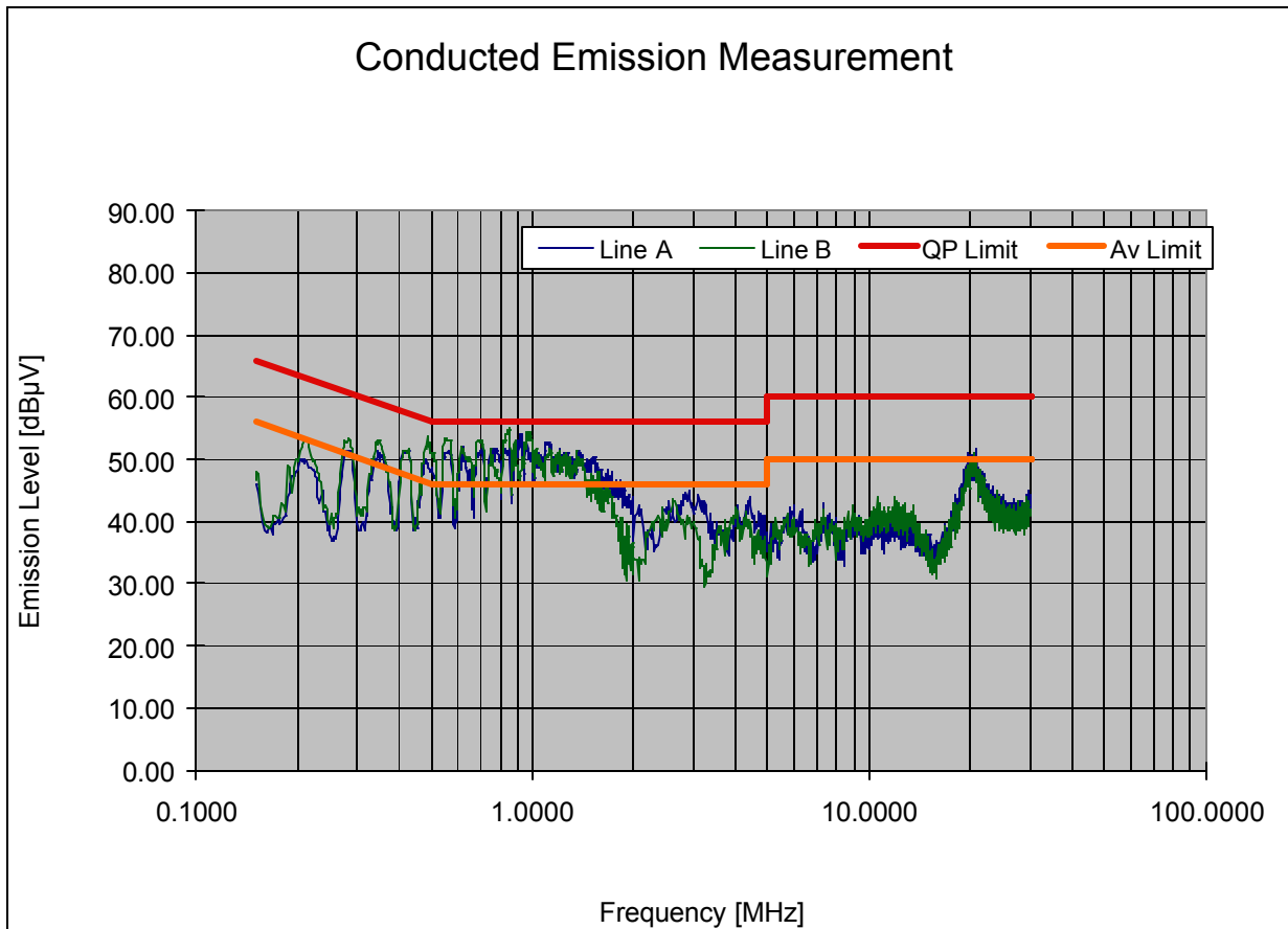
Plot 6-55. Line Conducted Plot with 802.11a
