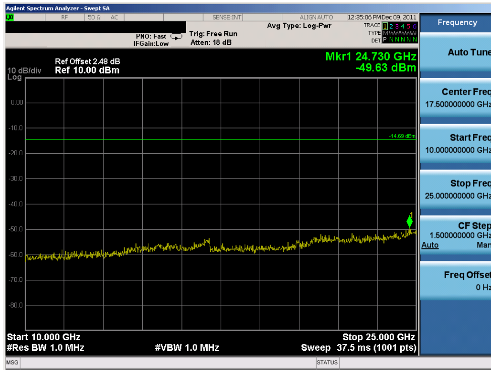
Plot 6-17. Conducted Spurious Plot (Bluetooth, 1Mbps – Ch. 0)
