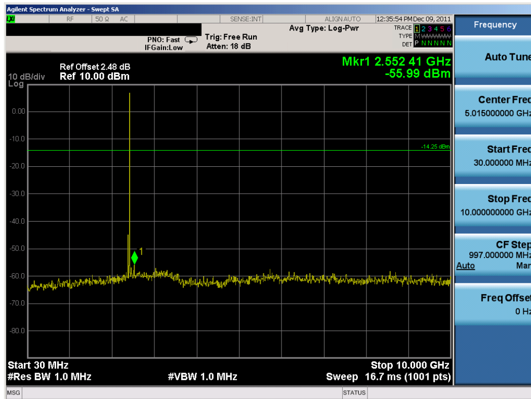
Plot 6-18. Conducted Spurious Plot (Bluetooth, 1Mbps – Ch. 39)
