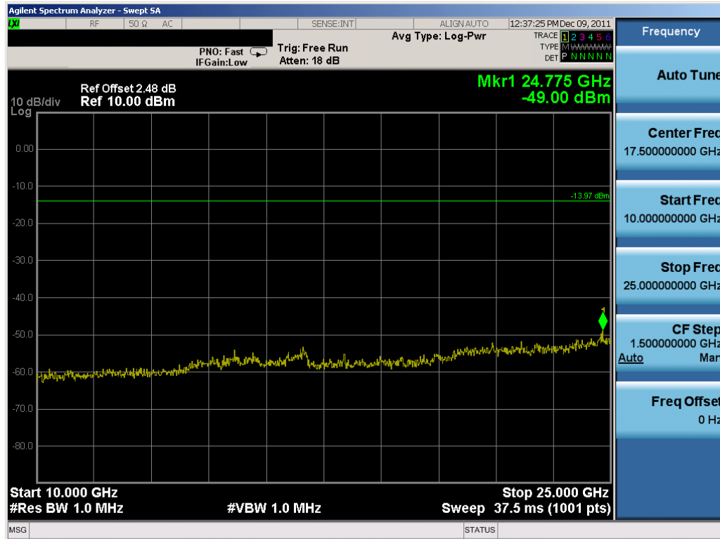
Plot 6-21. Conducted Spurious Plot (Bluetooth, 1Mbps – Ch. 78)
