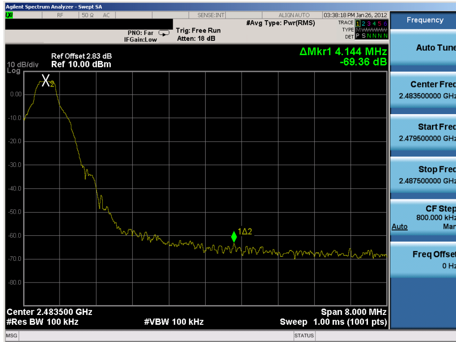
Plot 6-11. Band Edge Plot (Bluetooth, 1Mbps – Ch. 78)
