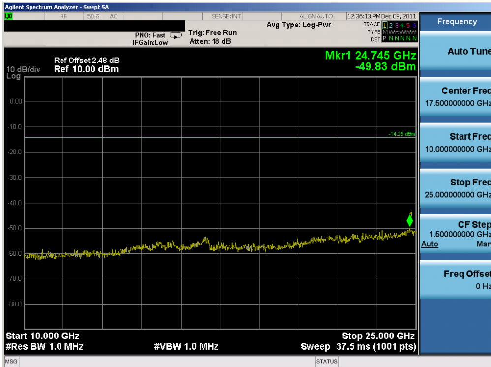
Plot 6-19. Conducted Spurious Plot (Bluetooth, 1Mbps – Ch. 39)
