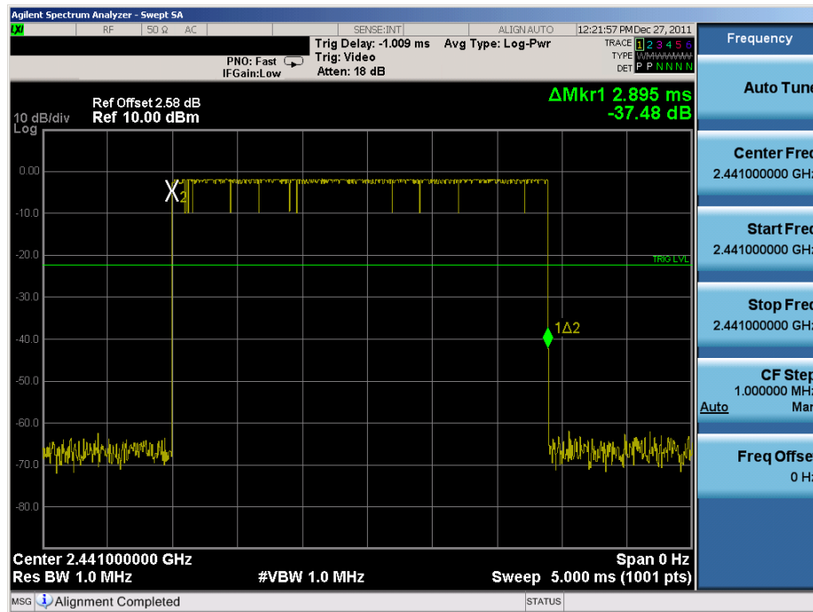
Plot 6-13. Time of Occupancy Plot (Bluetooth)
