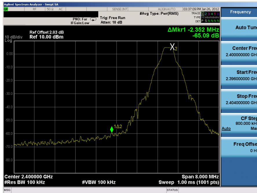
Plot 6-10. Band Edge Plot (Bluetooth, 1Mbps - Ch. 0)
