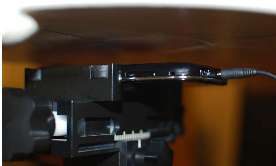
Figure 19-5 SAR Test Setup Photo 5
