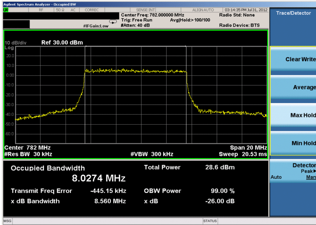
Plot 7-6. Occupied Bandwidth Plot (16-QAM – RB Size 50)
