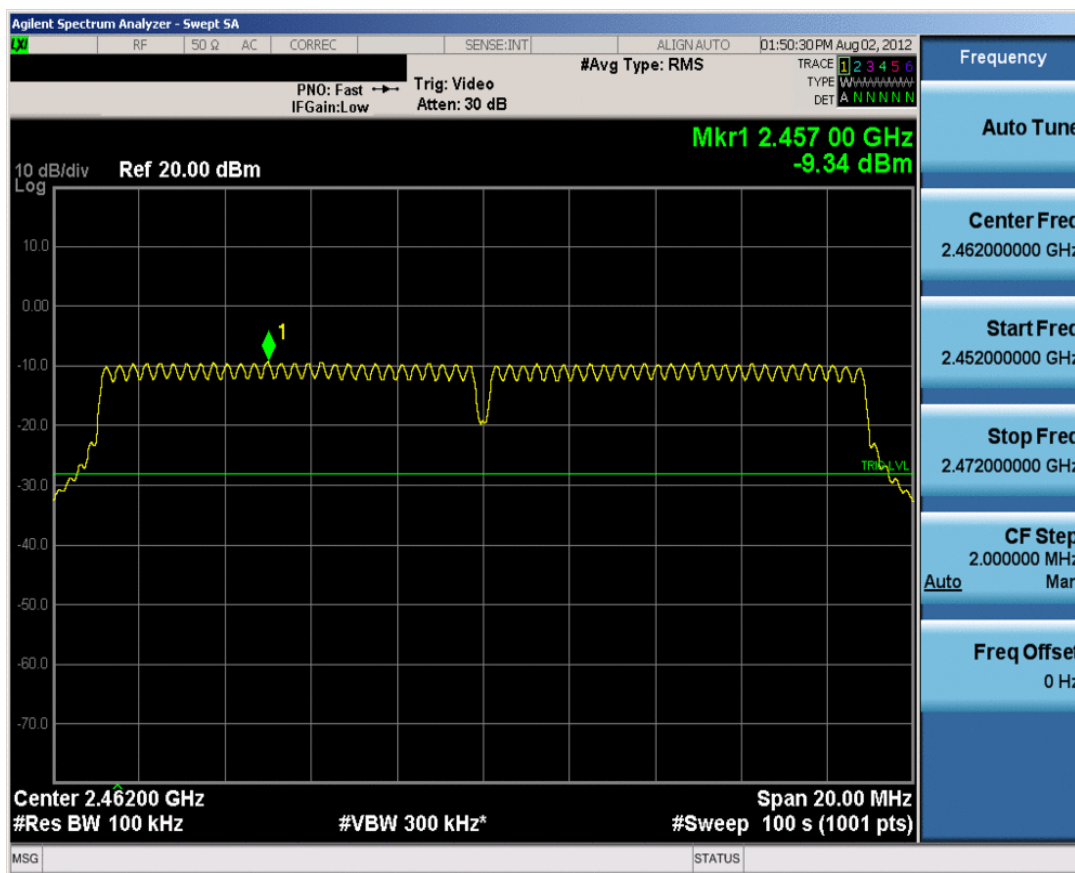
Plot 6-18. Power Spectral Density Plot (802.11n – Ch. 11)
