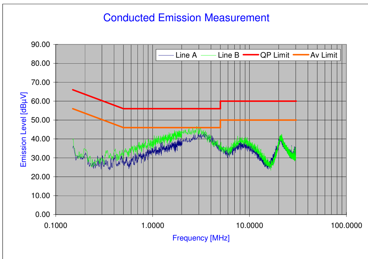
Plot 6-52. Line Conducted Plot with 802.11a
