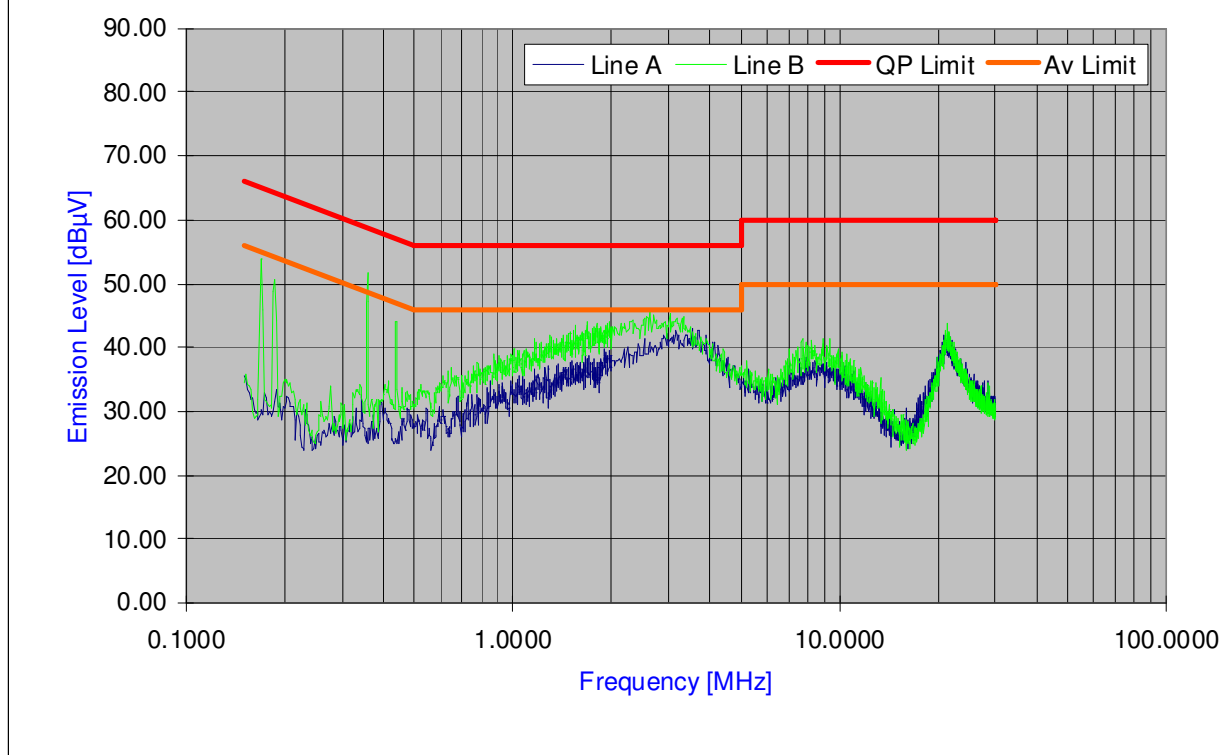
Plot 6-57. Line Conducted Plot with 802.11a (UNII Band 3)
