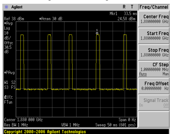
Figure 8.6 1/8 rate Signal
