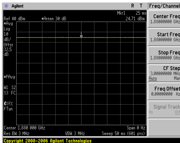
Figure 8.3 CW Signal
