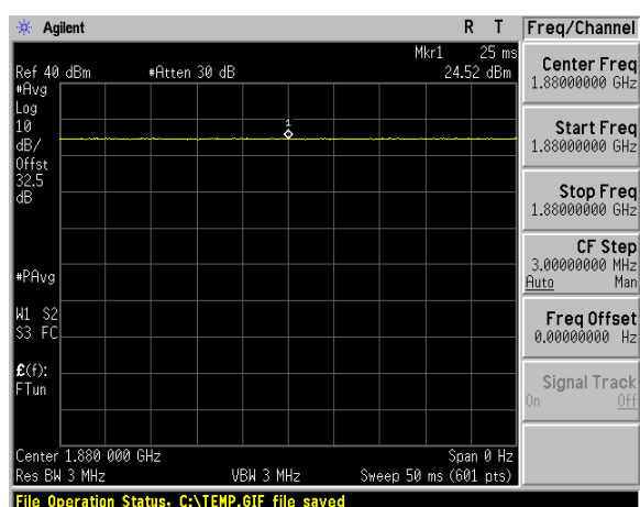
Figure 8.4 PCS Signal
