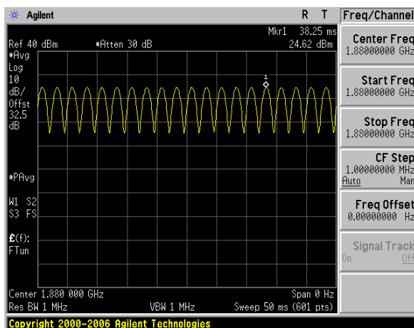
Figure 8.5 AM 80% Signal
