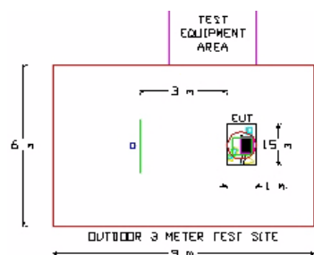
Figure 2-2. Dimensions of Outdoor Test Site
