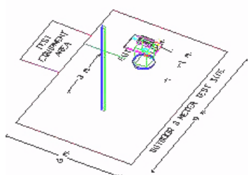
Figure 2-3. Turntable and System Setup
