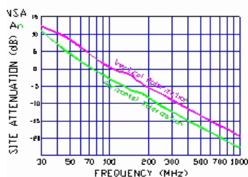
Figure 2-4. Normalized Site Attenuation Curves (H&V)
